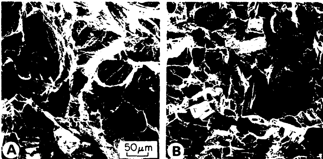
Fig. 4 Fracture surface of Ti-6Al containing approximately 100 ppm hydrogen tested at -70^{\circ}\text{C} . (a) 5 min hold at K_{\text{max}} ( da/dt = 6 \times 10^{-6} mm/s, K_{\text{max}} = 42.7 \text{ mPa}\cdot\text{m}^{3/2} ), (b) SLC ( da/dt = 7 \times 10^{-6} mm/s, K_{\text{max}} = 49.4 \text{ mPa}\cdot\text{m}^{3/2} ).
