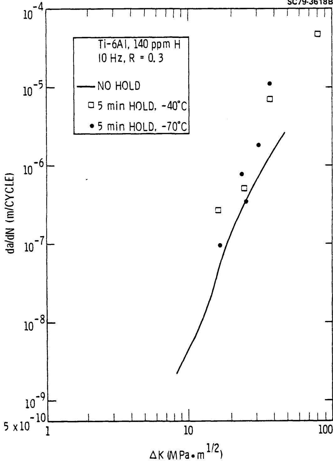
Fig. 2 Fatigue crack propagation results for Ti-6Al containing 140 ppm hydrogen tested at -40 and -70^\circ\text{C} .
