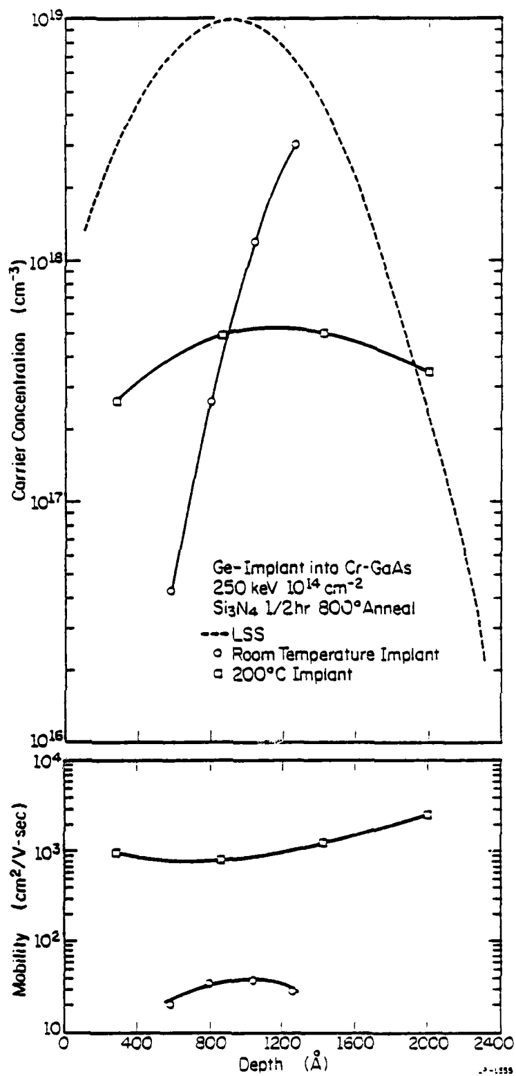
Fig. 3.7 Carrier concentration and mobility profiles for 10^{14} \text{ ions/cm}^2 Ge implants at room temperature and 200^\circ\text{C} .
