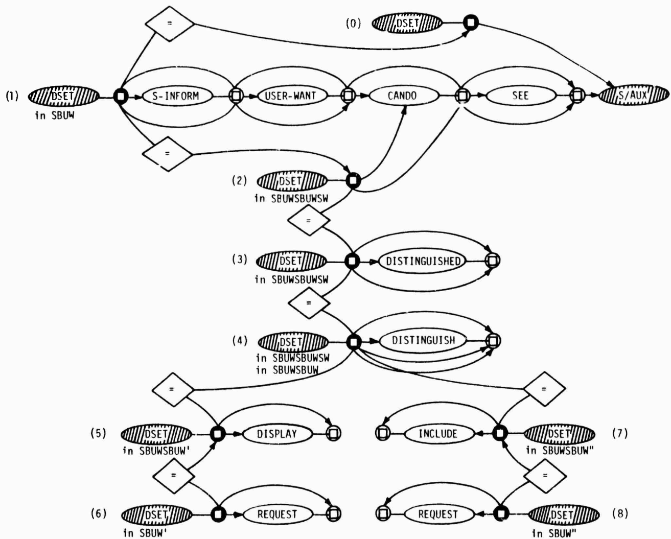
Fig. 23. The alternatives of DISPLAYing or INCLUDing.
