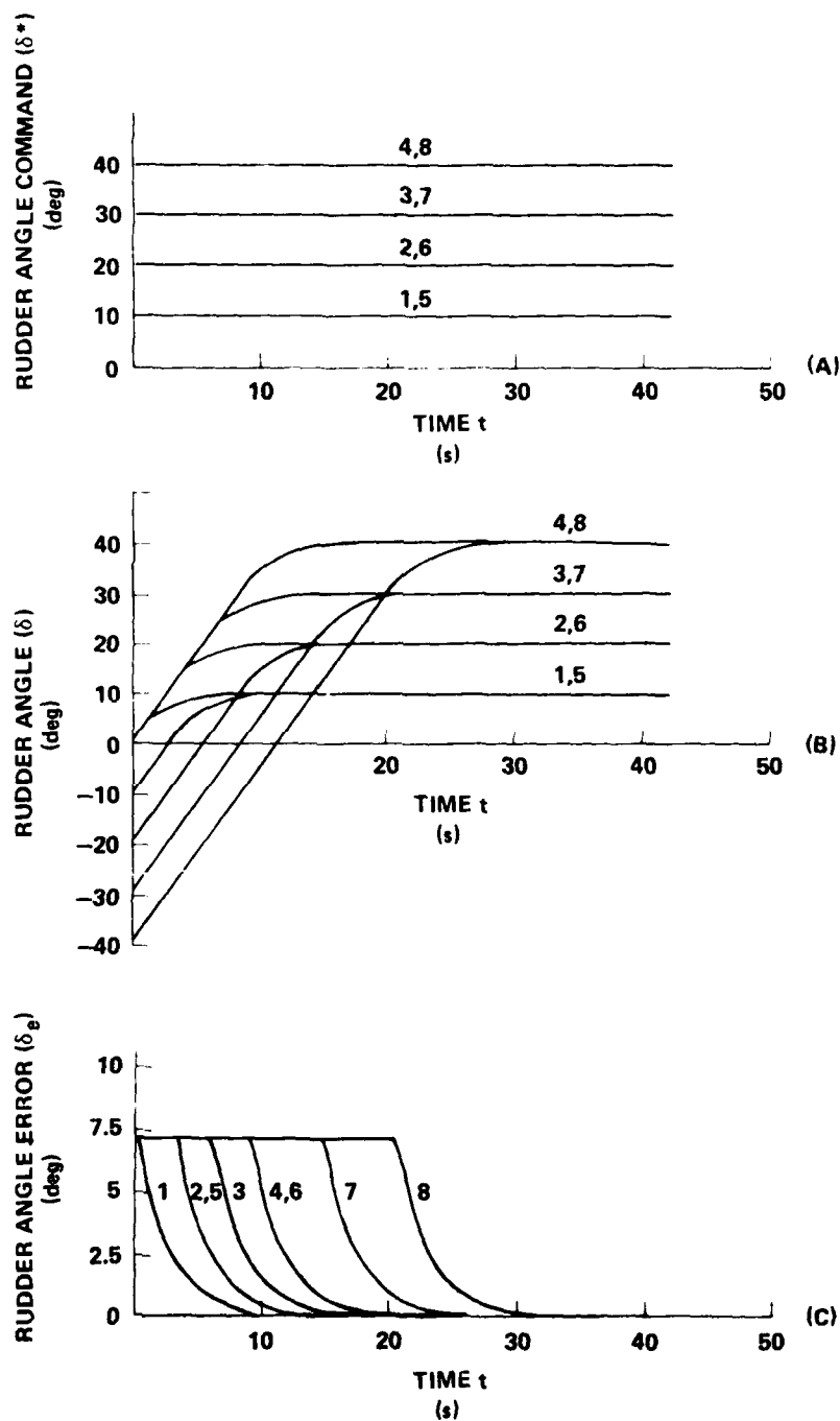
Figure A.4 - Response of Rudder System to Step Commands
