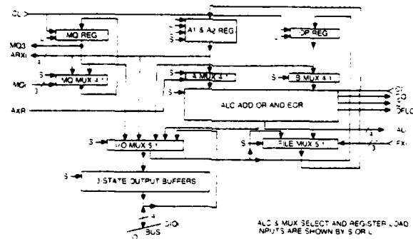
FIGURE 2.3-2 GPU DATA FLOW DIAGRAM
