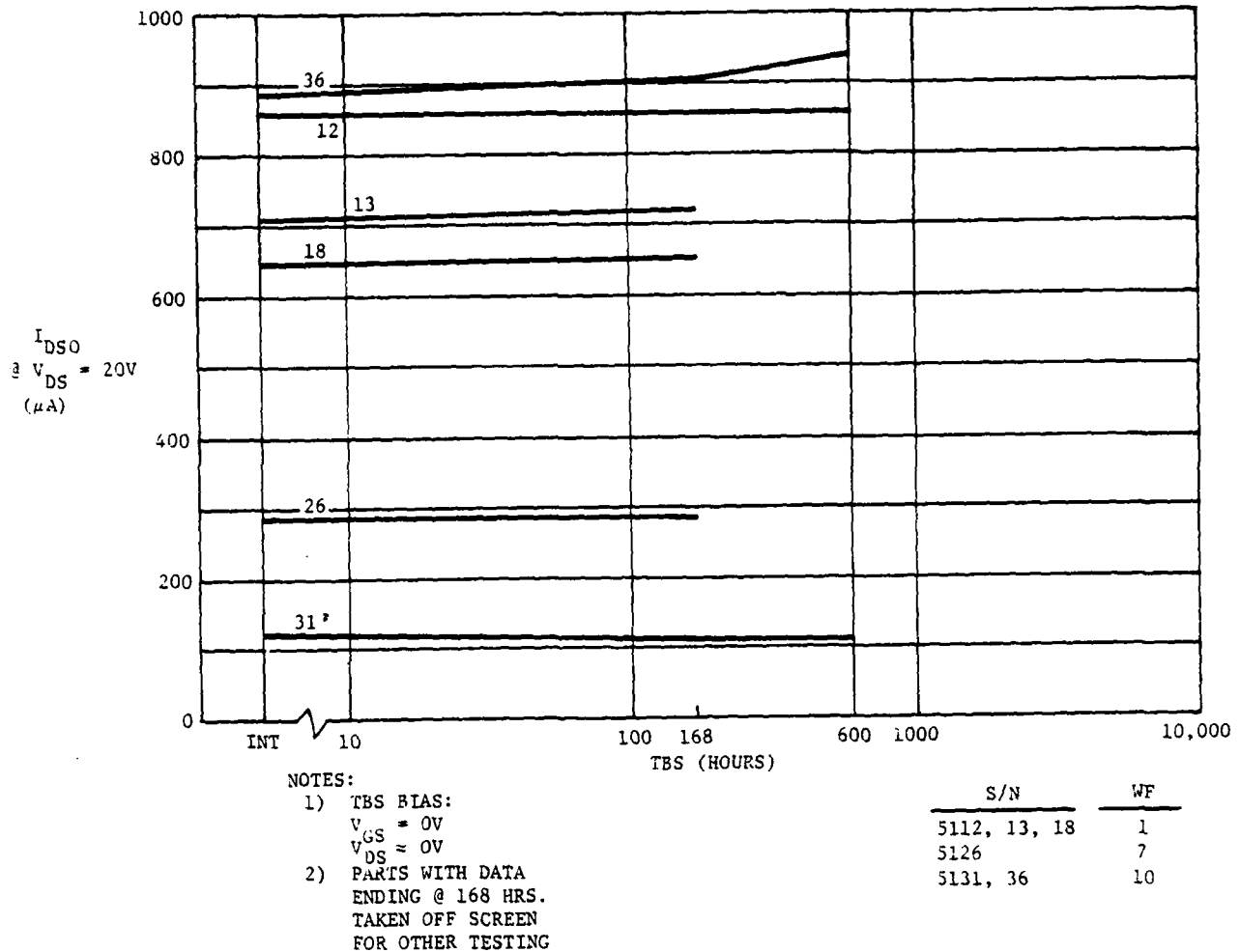
FIGURE 3.50 LOT 3888 SCREEN & LIFE TEST IDS0 VS TBS (T = 125°C)
