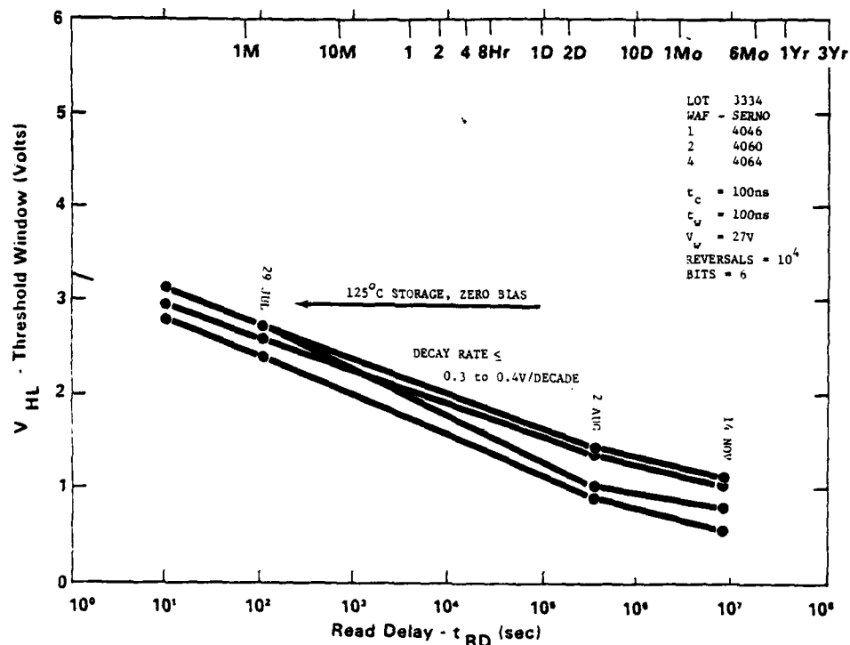
Figure 3.62. PSM: Pulse Response and Retention 125^\circ\text{C} , R = 10^4 52436
