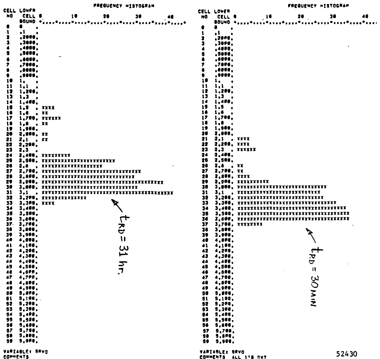
FIGURE 3.45 DI100 MEMORY WINDOW HISTOGRAM (256 BITS VS TIME)
