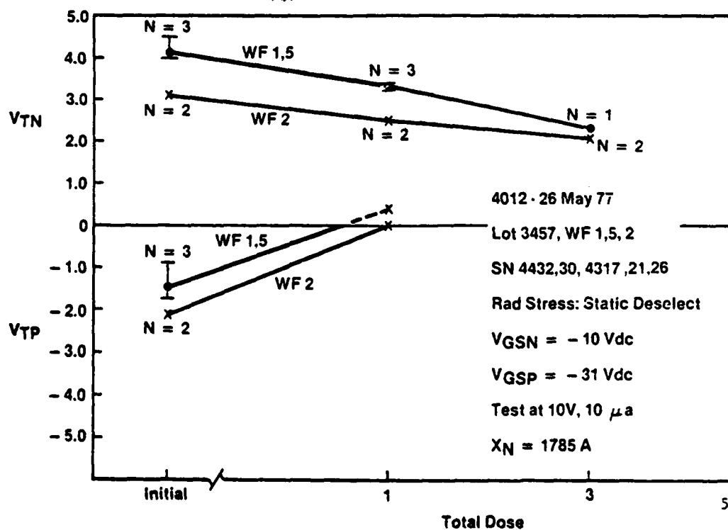
FIGURE 3.87 TSM: HIGH VOLTAGE THRESHOLD VS TOTAL DOSE
