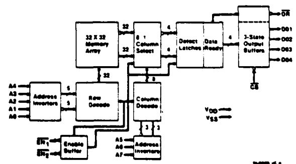
Figure 3. CMOS/SOS ROM Mask Programmable Organization for 256 Words by 4-Bits
