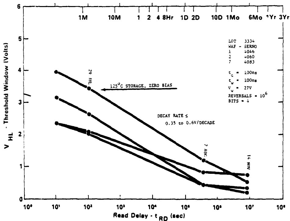
Figure 3.63. PSM: Pulse Response and Retention 125^\circ\text{C} , R = 10^6 52437
