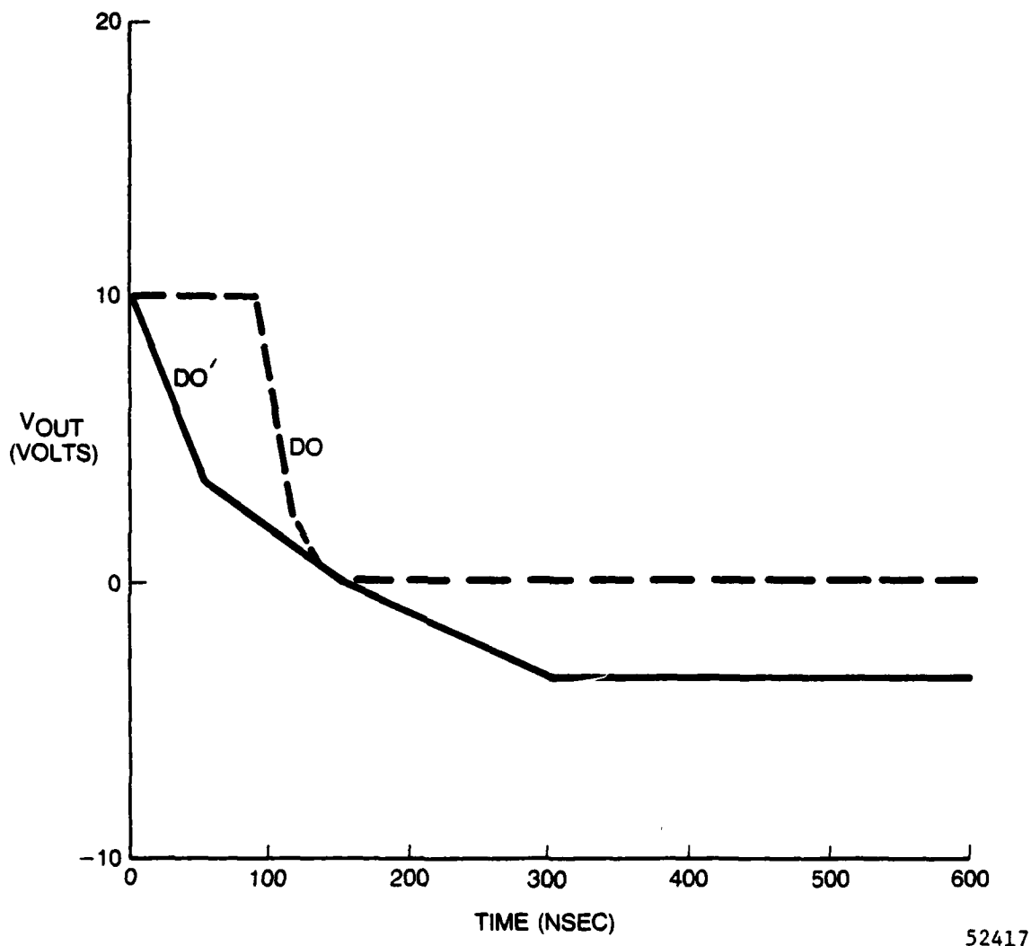
FIGURE 3.21 PSM: I/O BUFFER (DO) SIMULATION POST RAD, 125°C
