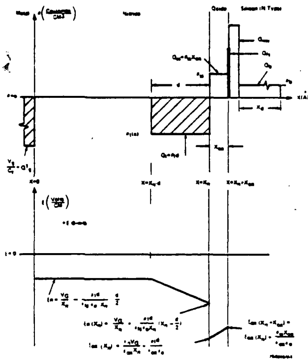
Figure 2. Charge Density ( C/cm^3 ) vs Insulator Thickness
