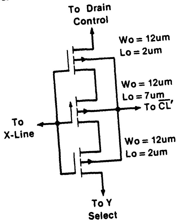
FIGURE 3.17 PSM: 3 FET MNOS MEMORY ARRAY DEVICE
