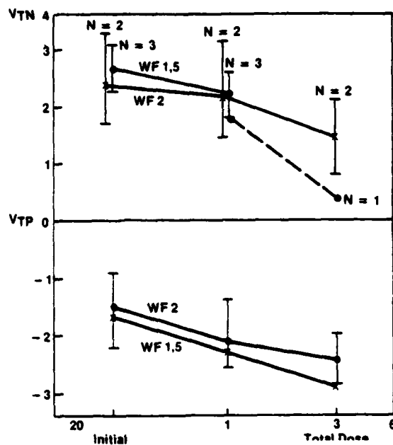
FIGURE 3.86 TSM: THRESHOLD VOLTAGE VS TOTAL DOSE
