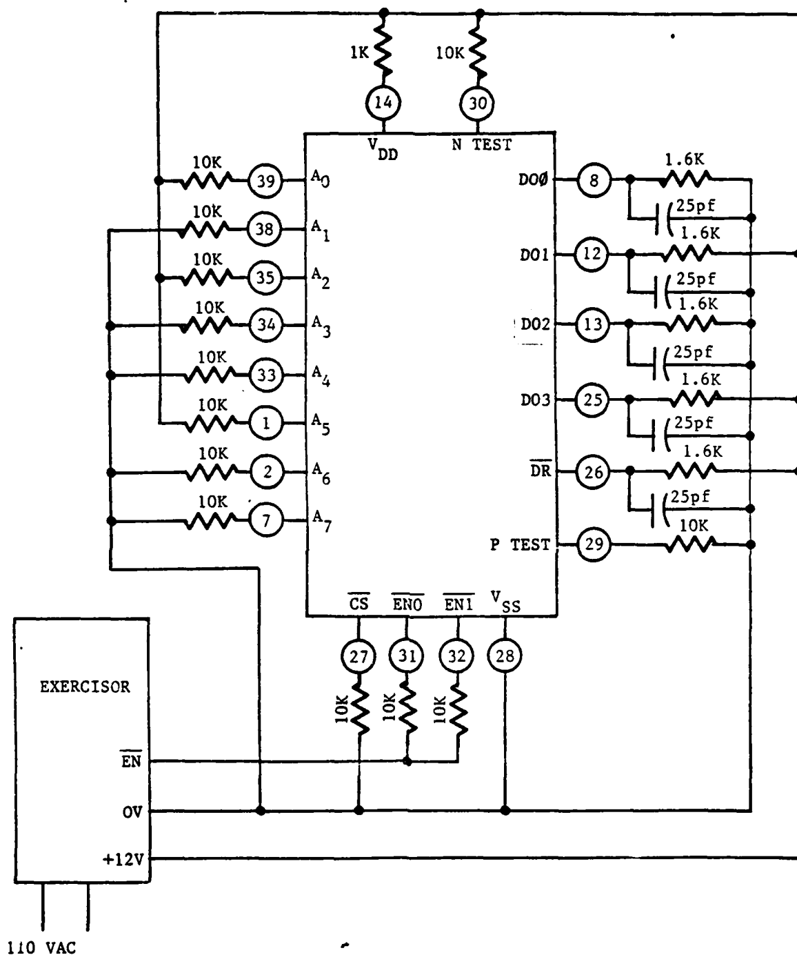
FIGURE 8B BURN-IN CIRCUIT, STATIC SELECT PARALLEL
