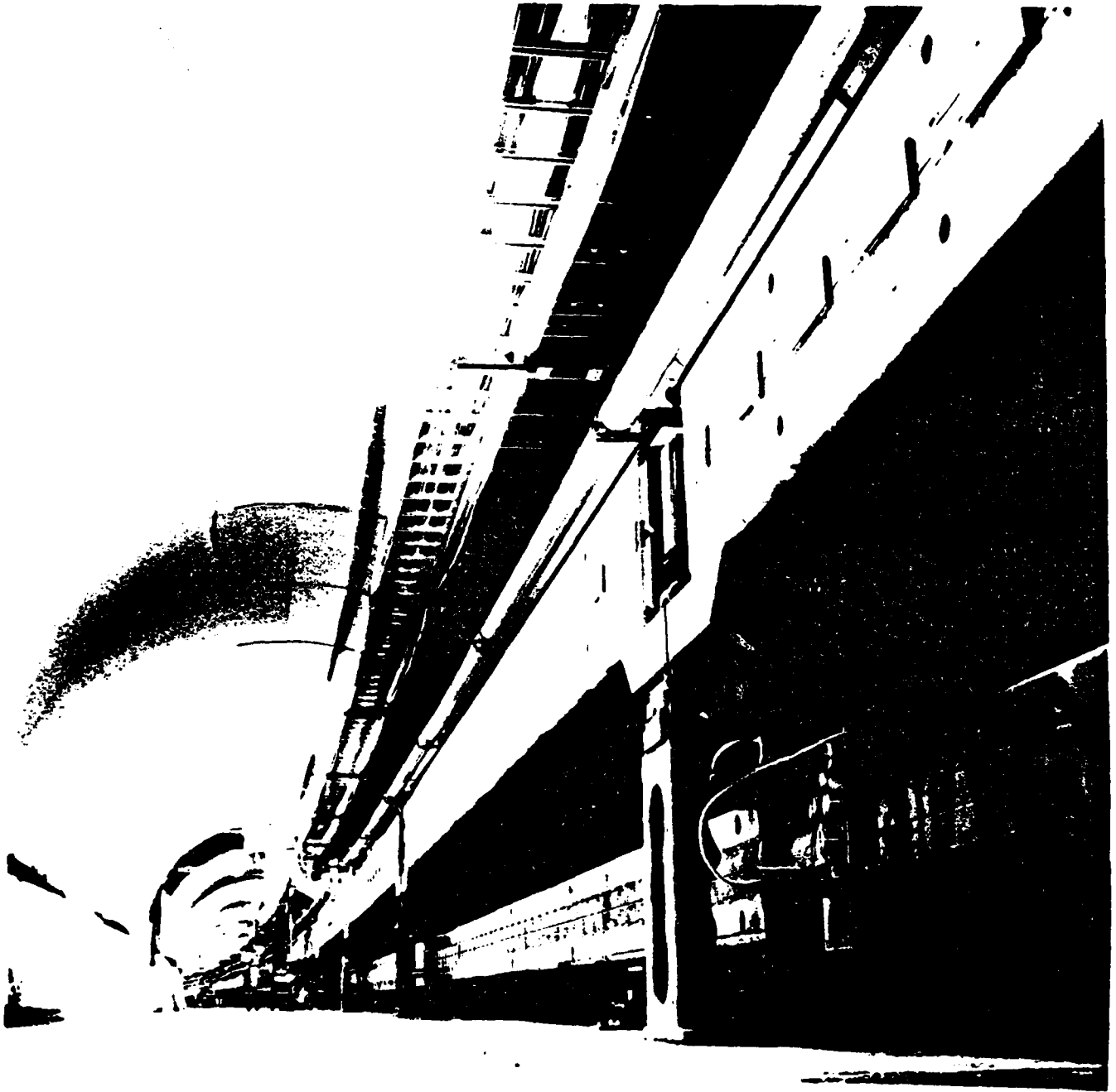
Superconductive and ordinary accelerator dipoles and quadrupoles at FNAL. There are 4 miles of NbTi accelerator magnets.
