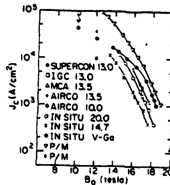
Fig. 14. Comparison of overall critical current density J_c versus applied field B_0 for commercial, "in situ" and cold-chamber process materials.
