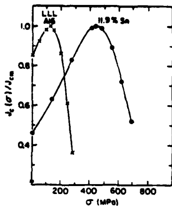
Fig. 7. Normalized J_c = J_c(\sigma)/J_{c0} where J_{c0} is the maximum critical current density under stress, as a function of stress \sigma at 14 T for 11.9 and 11.9 wt % Sn in Cu-35 wt % Nb "to 5-sec" wires. (After Ref. 6.)
