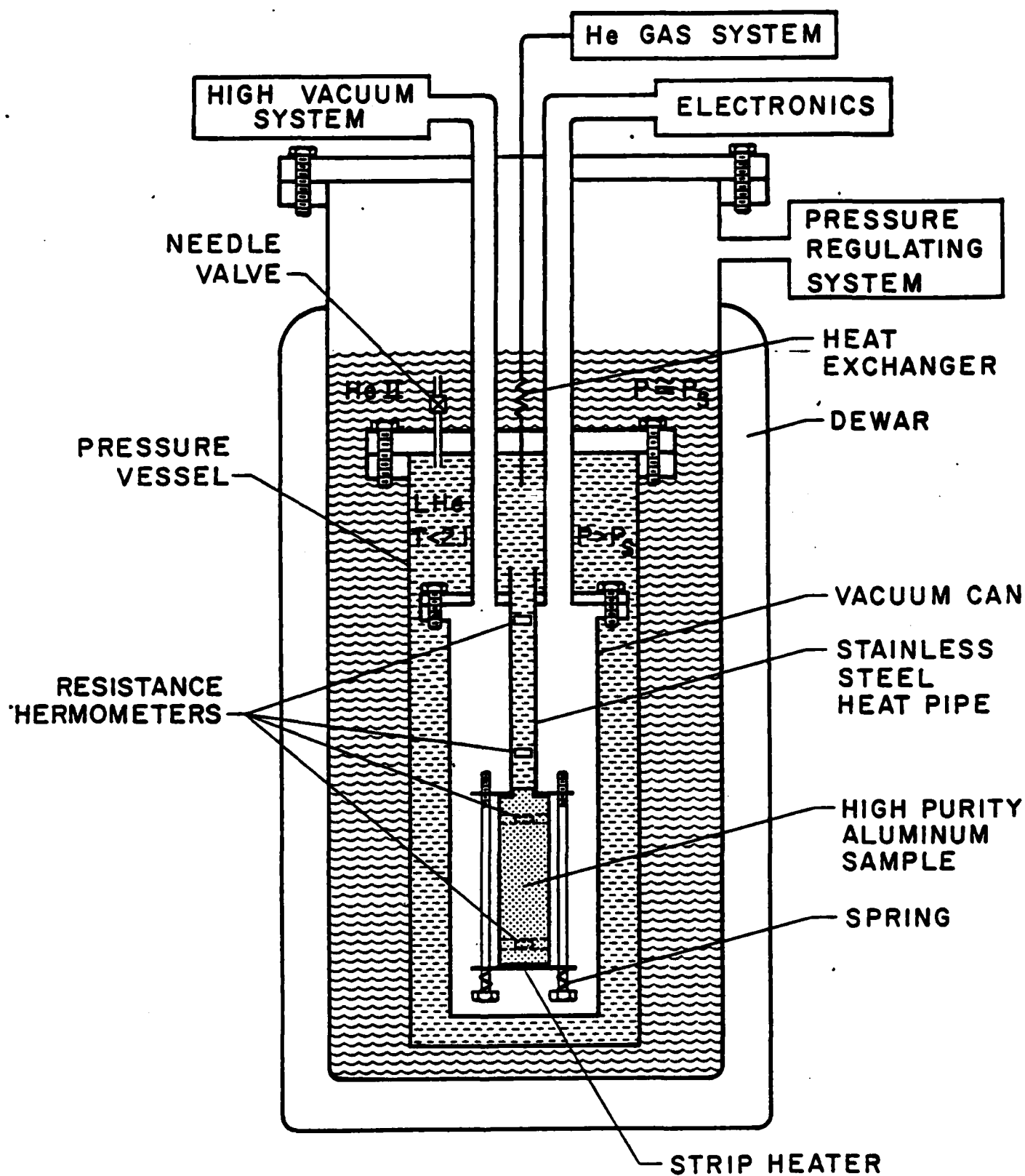
Pulsed heaters in He II.
