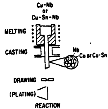
Fig. 2. Processing of "In Situ" multilayered superconductors proceeds from melting to the final stage of reaction to form filaments. (After Ref. 2)
