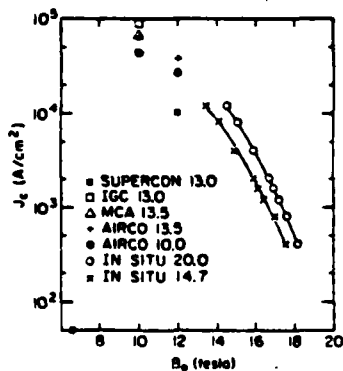
Fig. 3. Overall critical current density J_c versus applied field B_0 for "In Situ" Cu-36 wt% Nb-20 wt% Sn wires compared to published results for various techniques obtained in lower B_0 . (After Ref. 1.)
