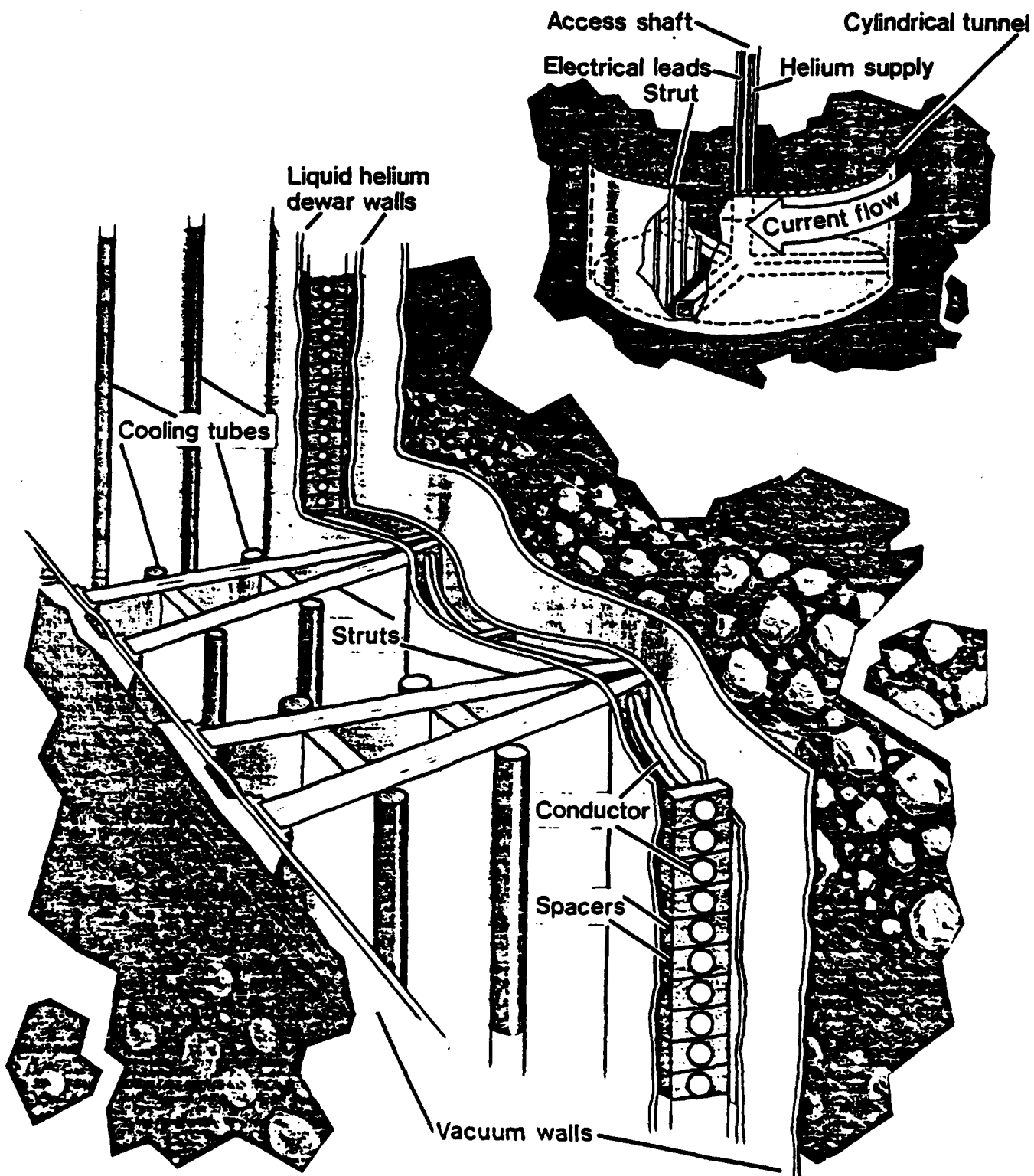
Storage solenoid cut-away.
