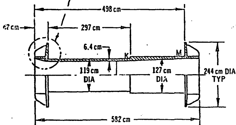
BORE TUBE & END FLANGES
