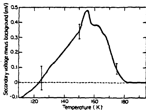
FIG. 1. This figure shows the deviation of the secondary voltage beyond background drift as a CuCl sample was warmed under 5 kbar pressure. The positive deviation indicates increased diamagnetism. The error bars indicate uncertainty in the background. The secondary voltage deviated from the background only between 120 and 180 K.
