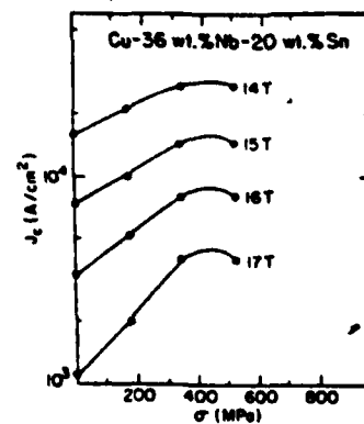
Fig. 5. Overall current density J_c versus stress, \sigma , for a Cu-36 wt% Nb-20 wt% Sn wire. The applied transverse field, B_0 is indicated for each curve. (After Ref. 5.)
