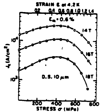
Fig. 9. Overall critical current density, J_c , versus stress and strain at 4.2 K for a 10 μm dendrite size directionally solidified in air. The base alloy was Cu-35 wt % Nb. (After Ref. 11.)
