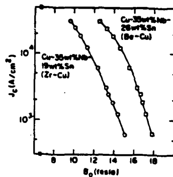
Fig. 12. Overall critical current density J_c versus applied field B_0 for cold-chamber process (P/M) processed Cu-Nb-Sn materials at 4.2 K. The two curves show representative results for two sets of P/M materials fabricated with a 12-μm grain size and a 10-μm grain size. The curves are in compression and axial reduction ratio 1. The wt % in the Cu-Nb-Sn is 35 wt % Nb in relation to Cu powder and does not include the external jacket. (After Ref. 14.)
