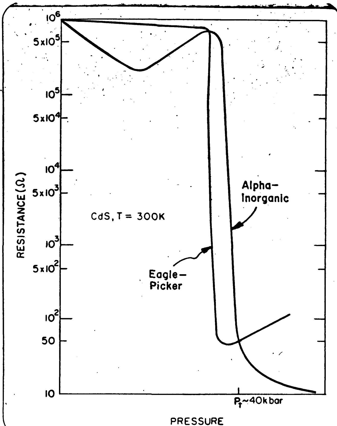
Pressure vs. resistance of two grades of CdS. The alpha inorganic material is the material which shows anomalous magnetic properties.
