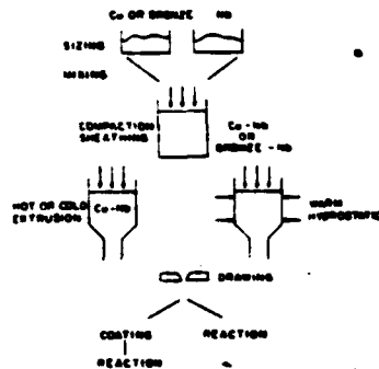
Fig. 2. Schematic of cold powder metallurgy multilayer Cu-Nb-Sn process.
