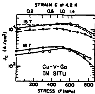
Fig. 10. Overall critical current density J_c at 4.2 K versus stress \sigma at fixed field for Cu-35 wt % Nb wires with in situ Cu-V-Ga. The wires were heat treated for 1 day at 600°C. The closed circles are for a grain growth at 4.2 K in presence of the wire measured 1 day at 600°C. The dashed curve at 15 T is the same wire measured after annealing the wire from 600 K to 4.2 K. (After Ref. 12.)
