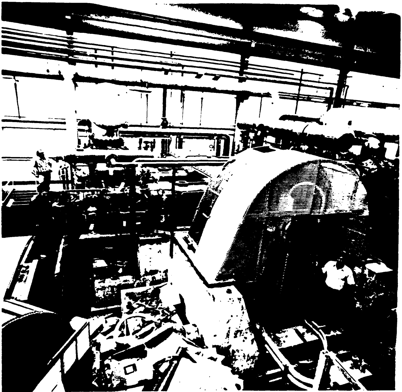
FNAL, 4000 hp compressor, two compressors provide 5000 liters of helium per hour (largest helium liquifier).
