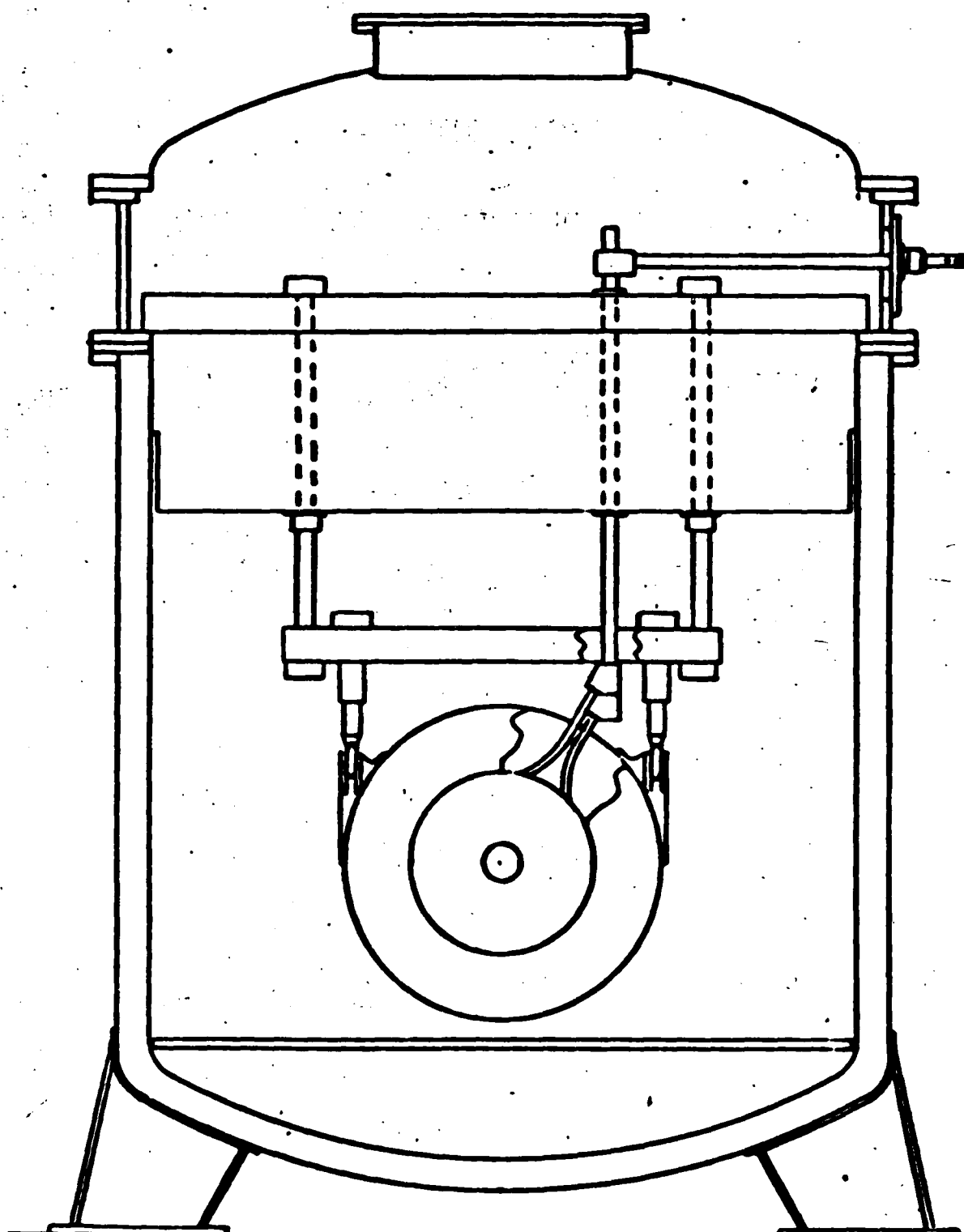
12 T HIGH FIELD TEST FACILITY 4 METER DIA. CRYOSTAT
