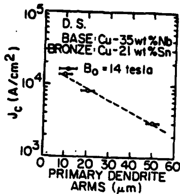
Fig. 8. Overall critical current density J_c at 14 T as a function of the primary dendrite arm size of the original alloy (open circles). All had the same composition and same heat treatment 1 day at 600°C. The closed circles are for a short-time anneal. (After Ref. 11.)
