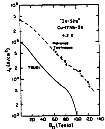
Fig. 4. Critical current density J_c tested small cross-sectional area of the wires versus applied field B_0 at 4.2 K. Results of Tsuei (Ref. 3) are compared with present "In-Situ" material: 0.25 mm-diam wire, 17 wt% Nb-7 wt% Sn annealed for 3 days at 650°C. (After Ref. 4.)
