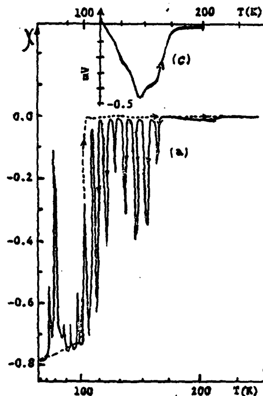
FIG. 3. Oscillatory susceptibility behavior: (a) the differential magnetic susceptibility observed at 20 Hz in CuCl redrawn from Brandt et al. , Ref. 6; (b) negative of phase change observed in secondary coil during 100 Hz susceptibility measurement in americium redrawn from Olsen. (Ref. 10); SC: superconducting. INT: intermediate state. N: normal; (c) work reported herein redrawn on the same (logarithmic) temperature scale as Brandt et al. , (Ref. 6).
