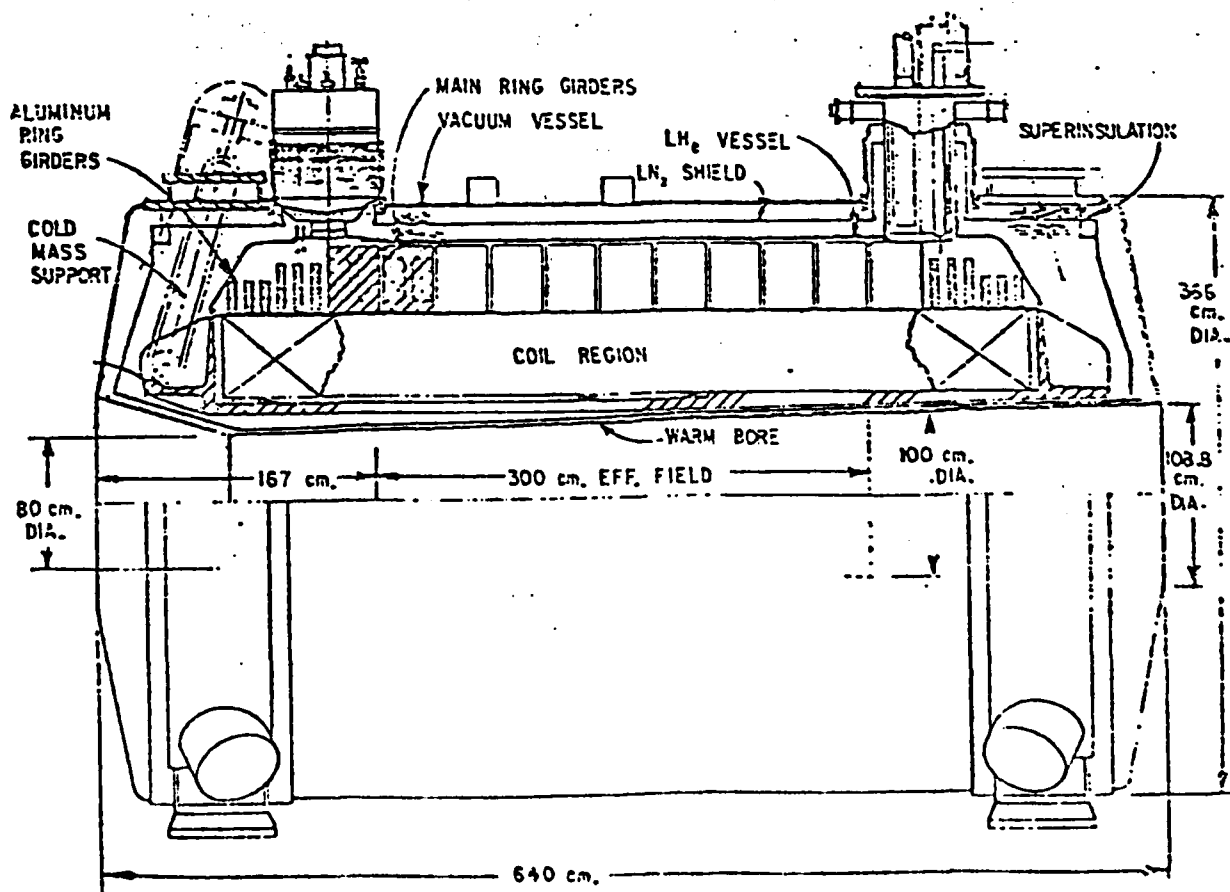
Magnet Overall Detail
