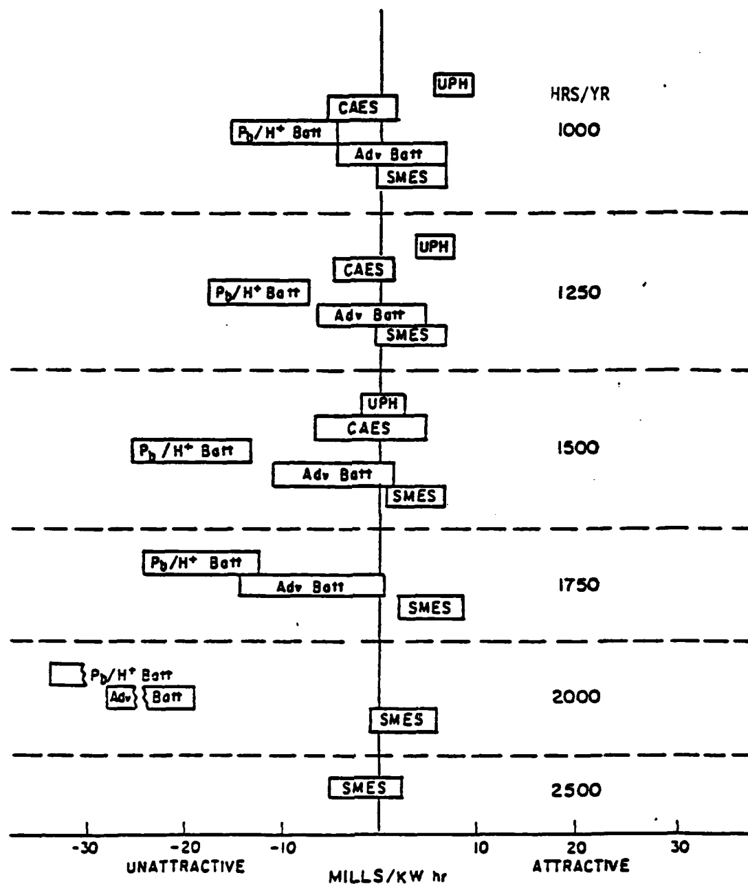
FIGURE 3.6 LEVELIZED BUS BAR COST DIFFERENCE BETWEEN STORAGE AND CONVENTIONAL GENERATION C=15 Mills/kw hr. P_d (max) = 1000 MW
