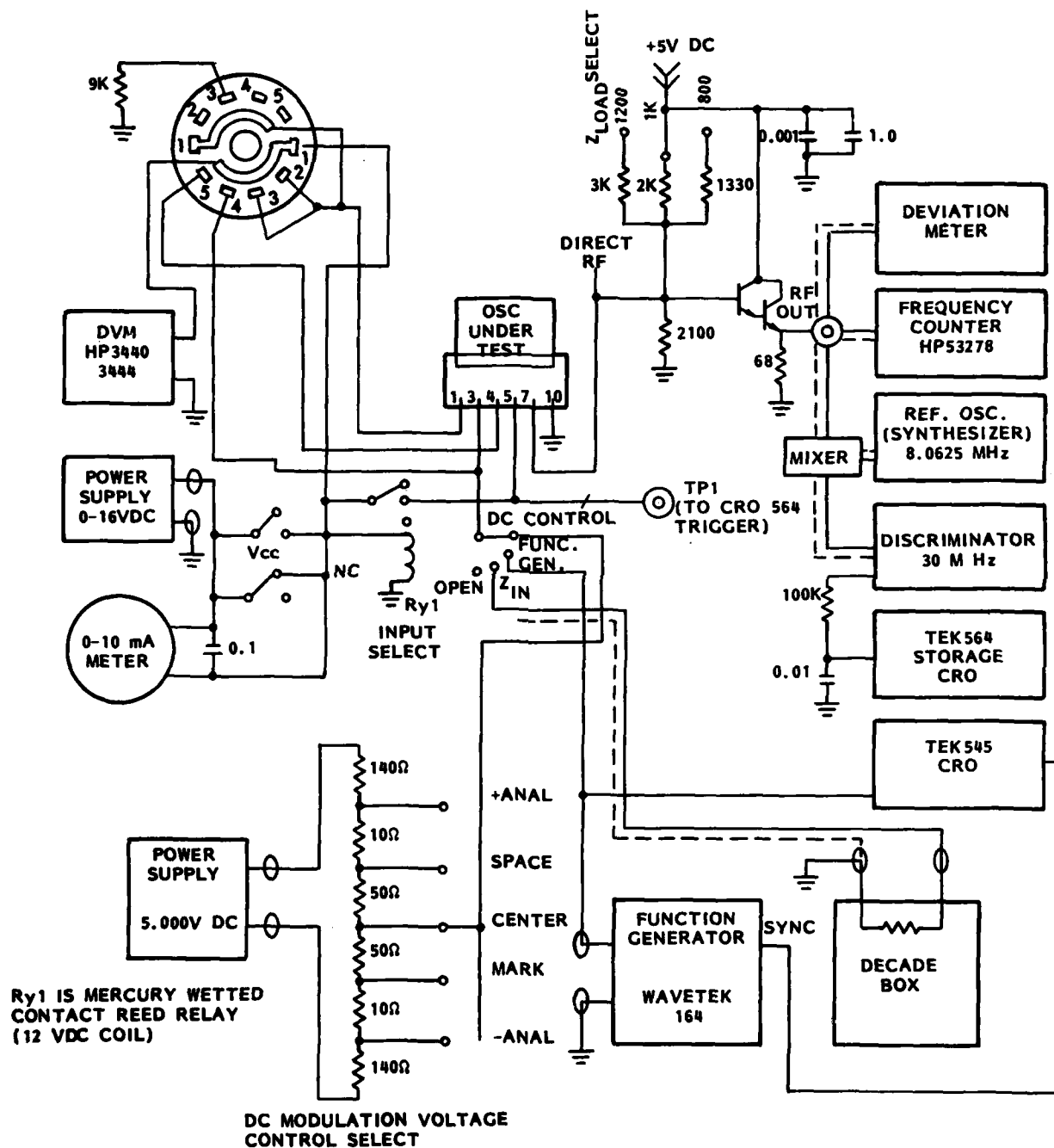
FIGURE 1. TCVCXO MODULE TEST SET
