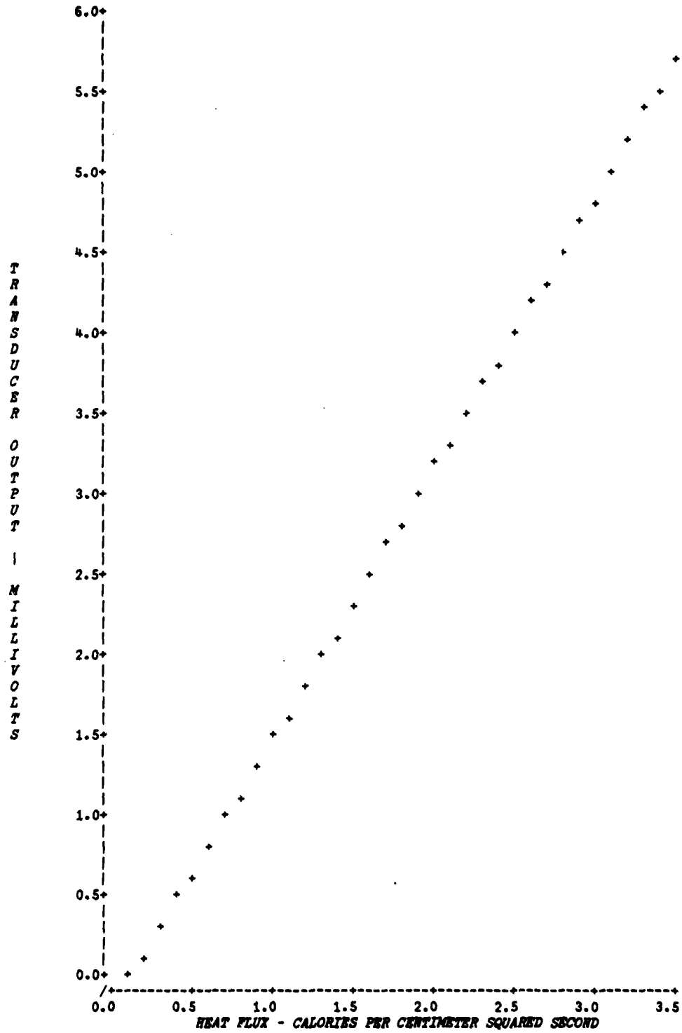
FIGURE 3 - CALIBRATION CURVE FOR NCTR'S HEAT FLUX TRANSDUCER
