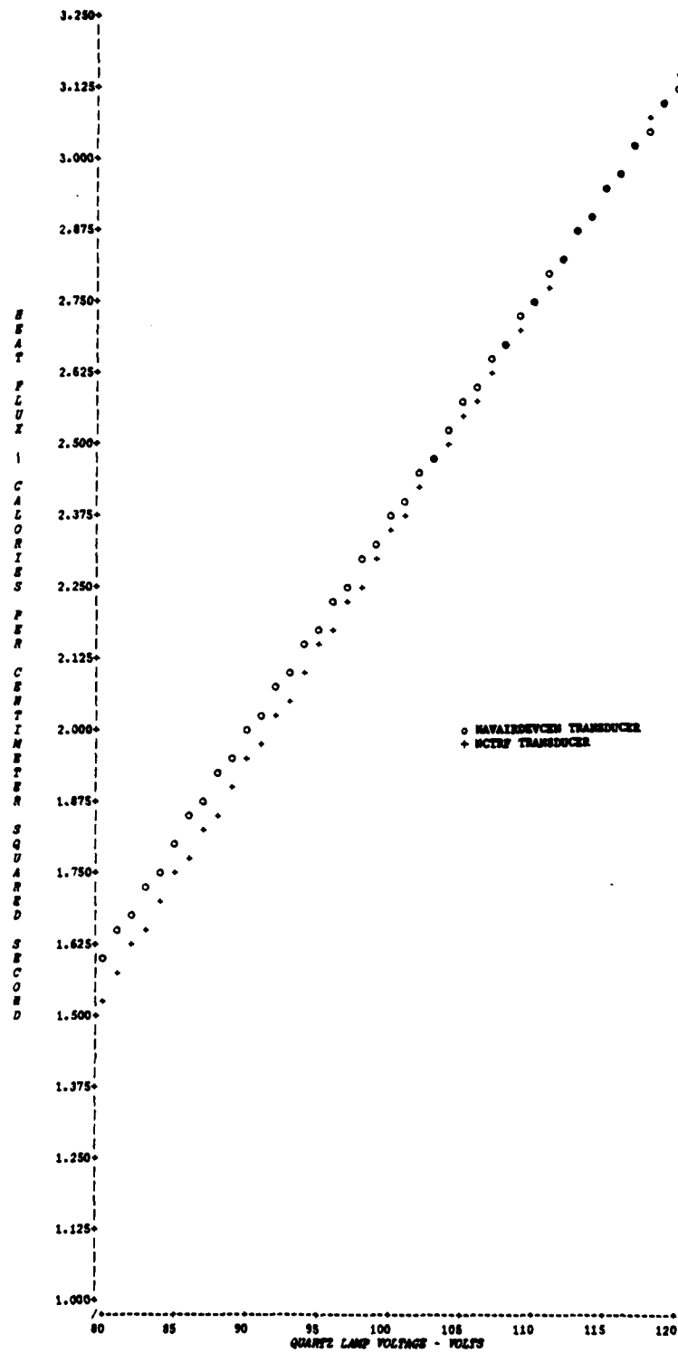
FIGURE 2 - HEAT FLUX VS QUARTZ LAMP VOLTAGE FOR NCTRF AND NAVAIRDEVGEN TRANSDUCERS AT 1.0 in (25.4 mm) LEVEL
