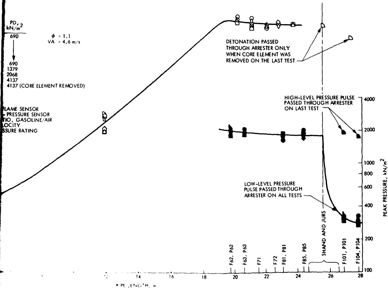
Figure 8-7. Shand and Jurs Spiral-Wound, Crimped Aluminum Ribbon Arresters Assembly Test Results
