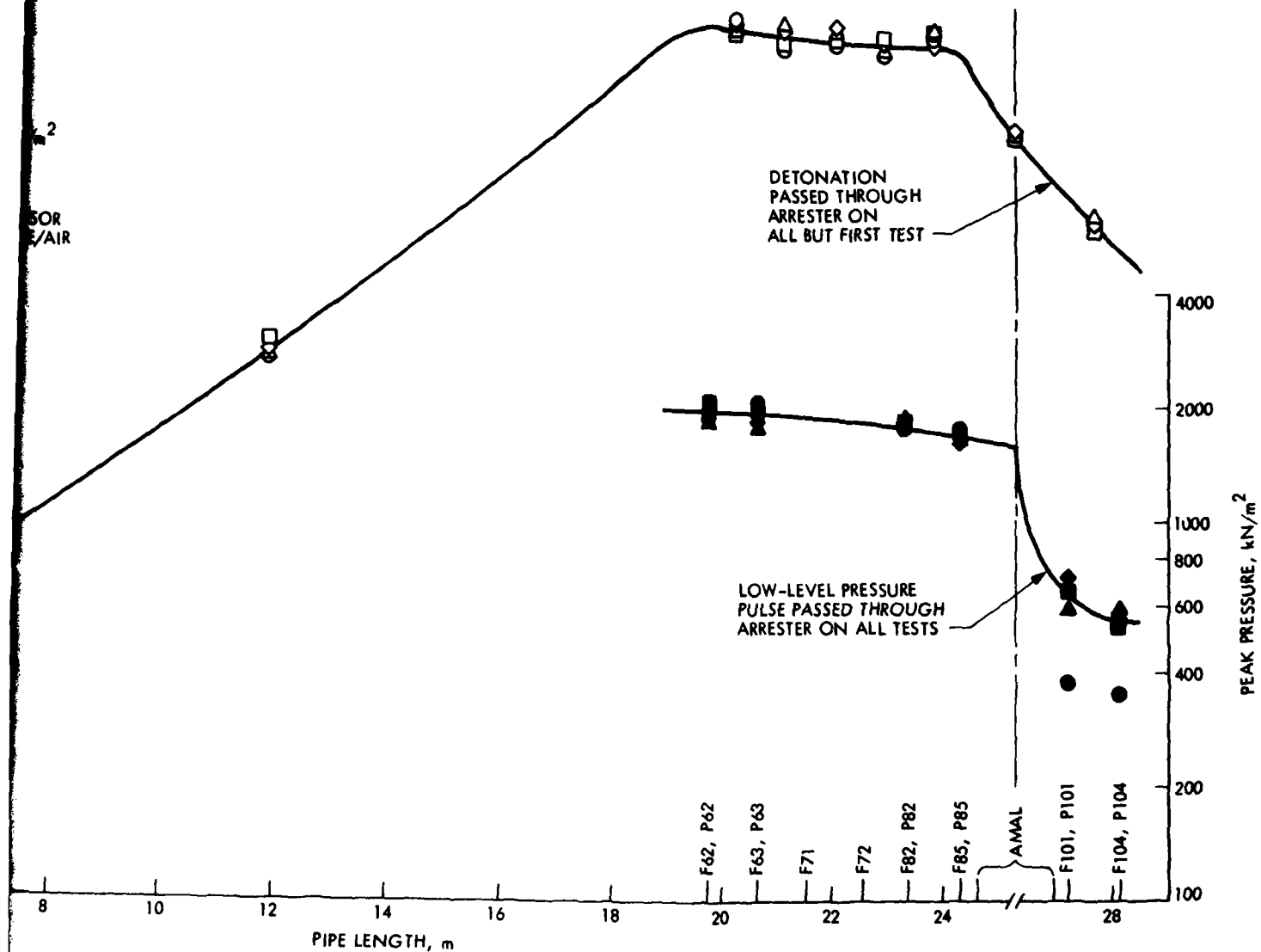
Figure 8-11. Amal Spiral-Wound, Grimped Stainless-Steel Ribbon Arrester Assembly Test Results
