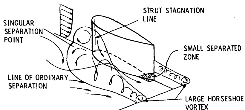
PROPOSED MODEL OF THICK BOUNDARY-LAYER-STRUT INTERACTION
