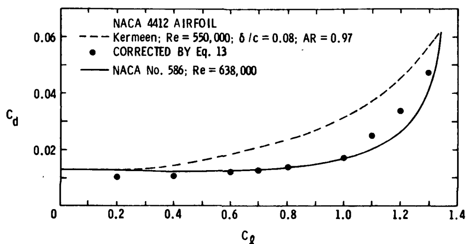
Figure 44. Kermeen's data corrected by Equation (13).
