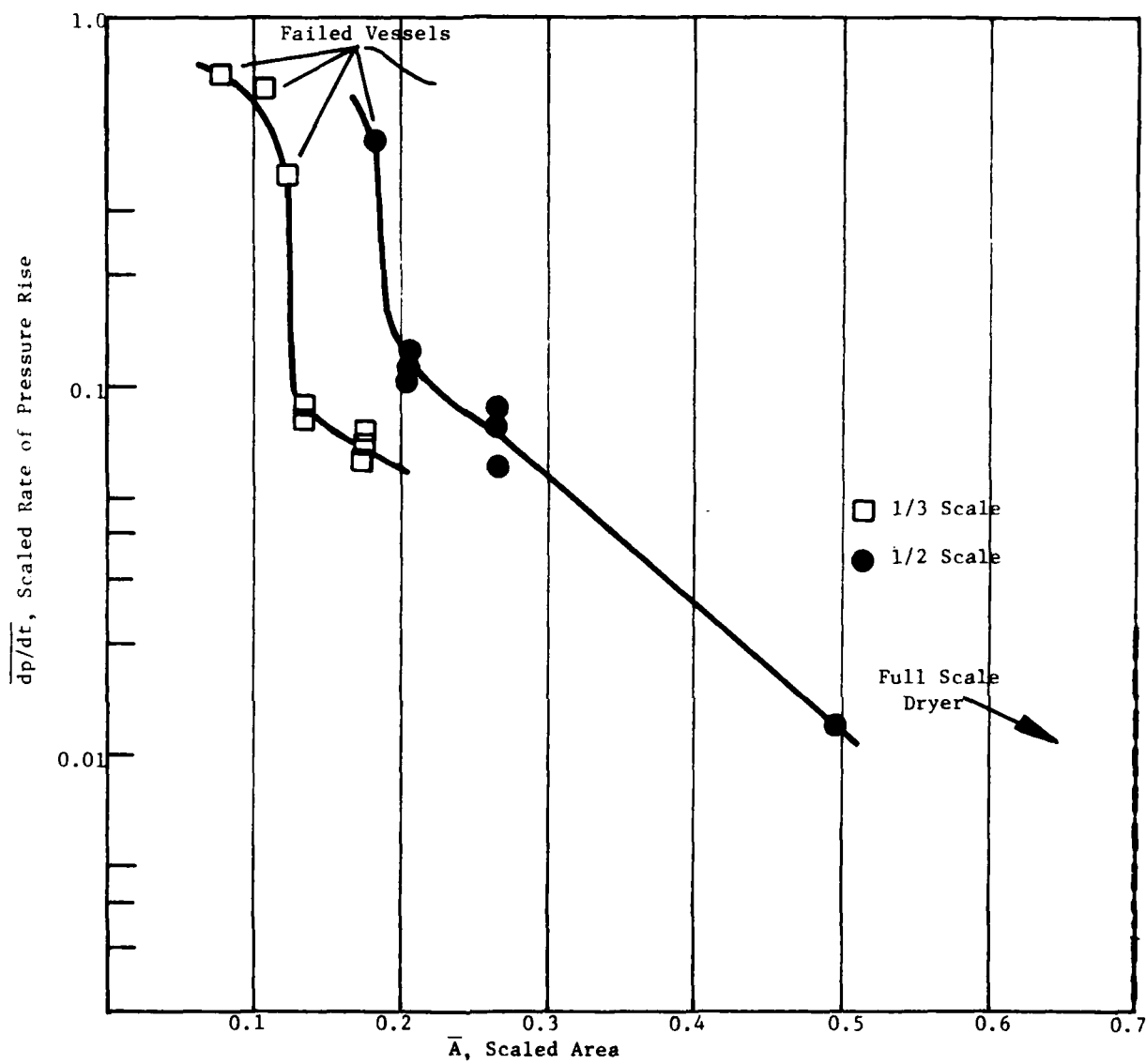
Figure 6. Scaled rate of pressure rise versus scaled vent area for M26 cannon propellant
