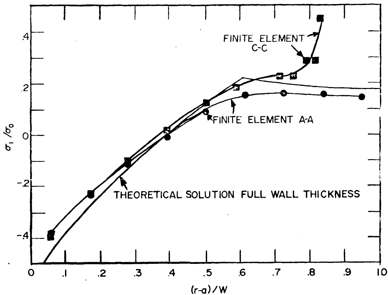
Figure 13. Finite element results for the deep notch 60% overstrain loading condition.
