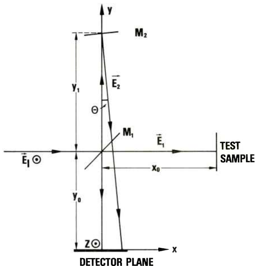
Figure 3. Setup of interferometer for analysis.
