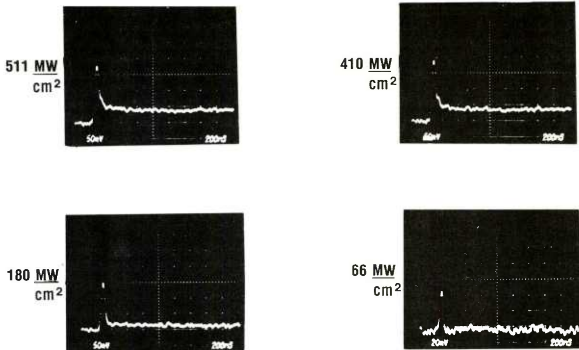
Figure 11. Oscilloscope photographs of received acoustic waves for various power densities, keeping generating spot size constant. The vertical scales are 50 mV/div for all but the 66 \text{MW}/\text{cm}^2 case, when it is 20 mV/div. Horizontal scales are all 200 ns/div.
