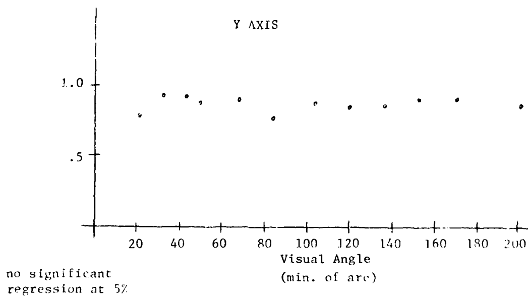
Figure 4-8. Autocorrelation Coefficients
