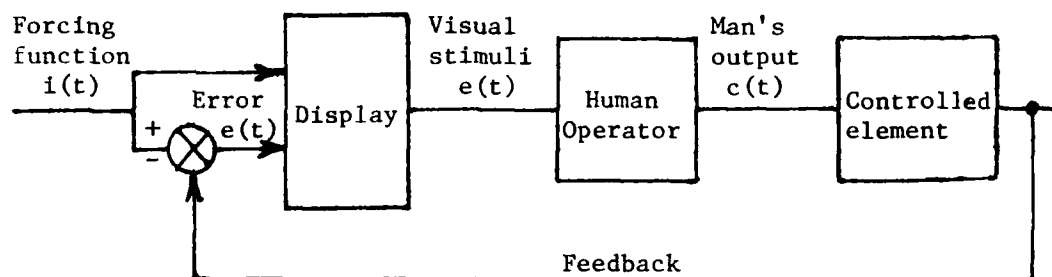
Figure 2-1. Block Diagram of Pursuit Tracking
