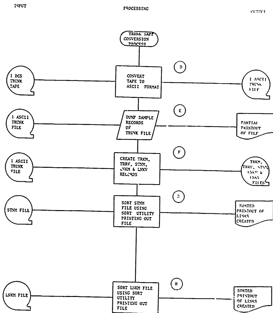
Figure 3-2. Data Base Build Process (sheet 2 of 5)
