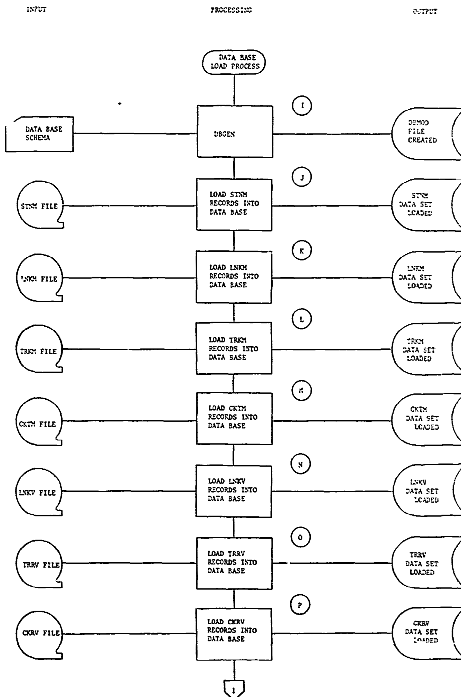
Figure 3-2. Data Base Build Process (sheet 3 of 5)
