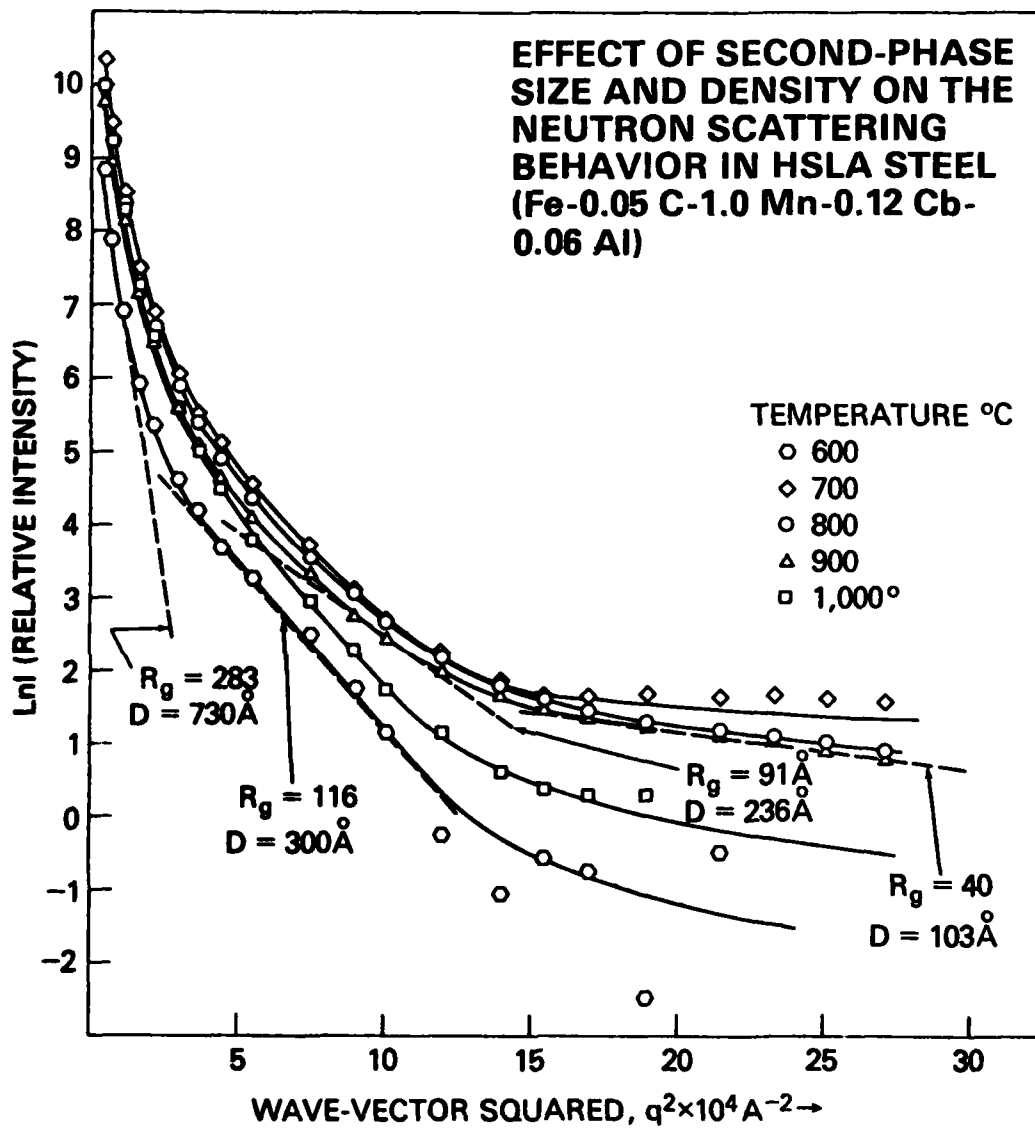
FIGURE 3 - GUINIER PLOTS OF SANS DATA FROM HSLA STEELS
