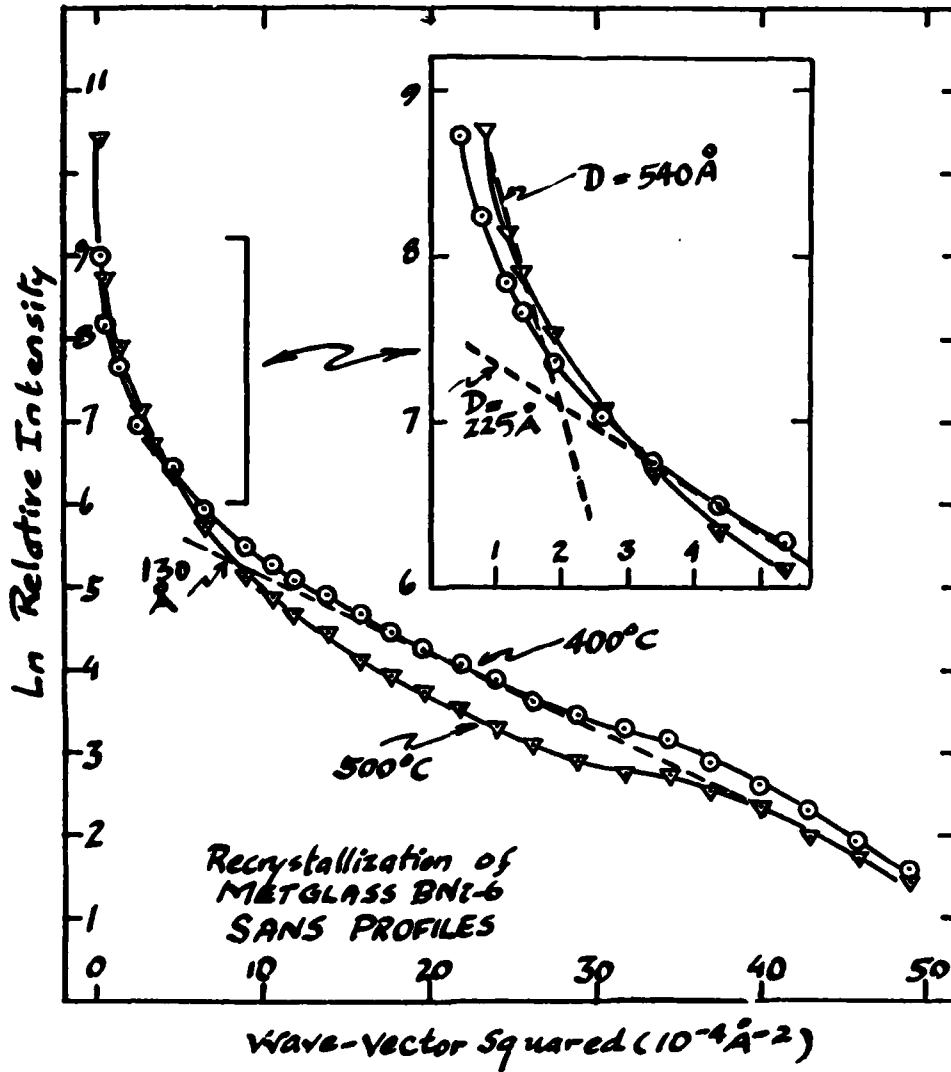
FIGURE 5 - GUINIER PLOTS OF SANS PROFILES FROM Ni-P AMORPHOUS GLASSES
