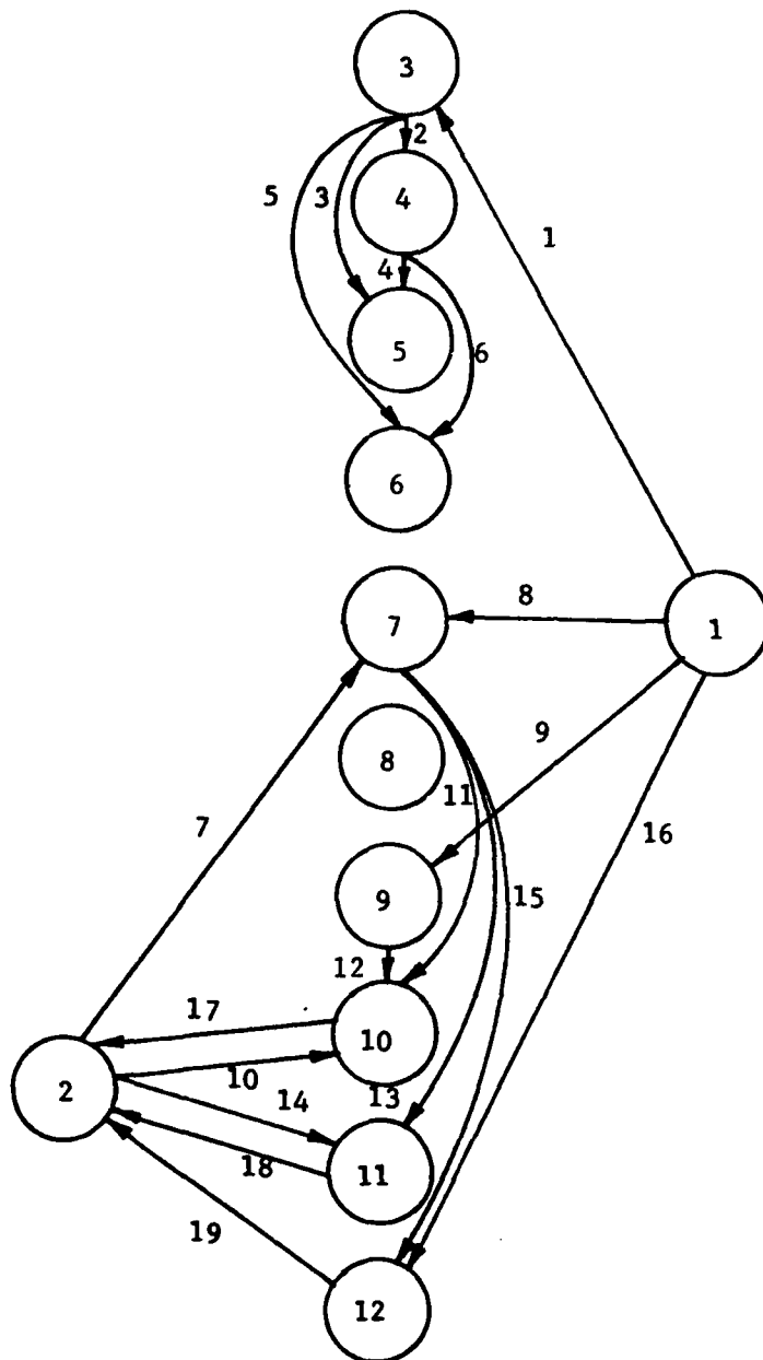
Figure 16. The data-flow graph for blocks 1-12 of LINER.
