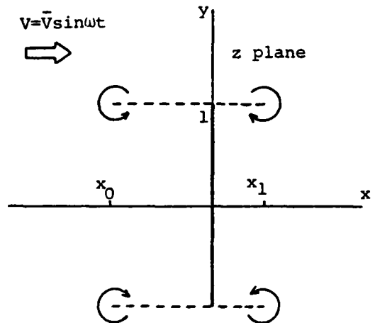
Figure 3.4. Two-vortex-pair model for oscillating flat plate
