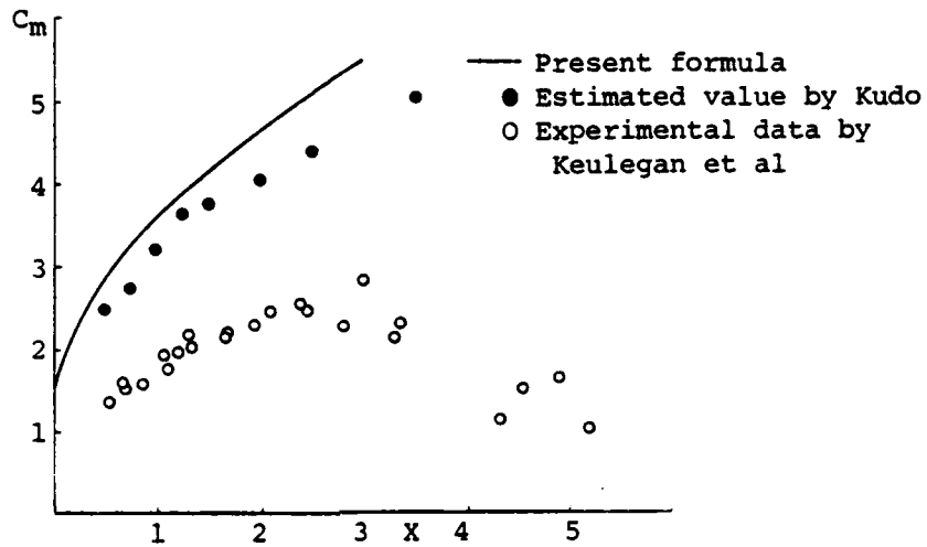
Figure 3.5. Added-mass coefficient of oscillating flat plate
