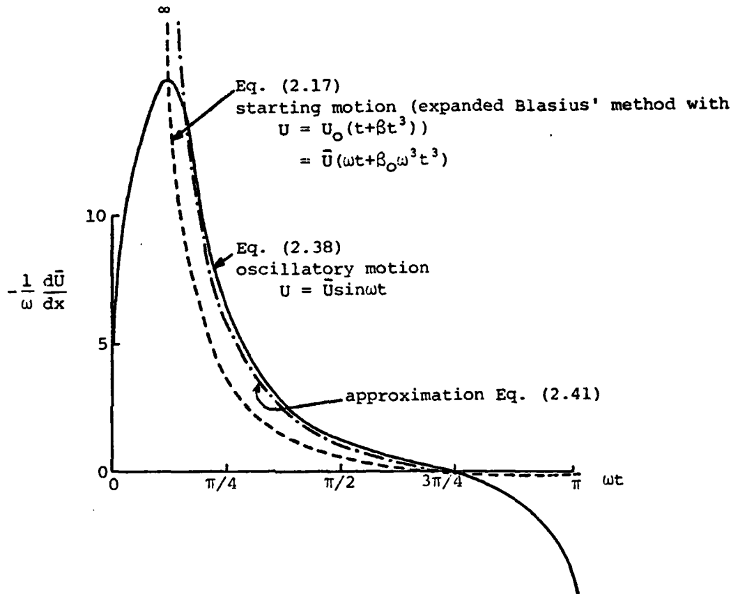
Figure 2-2. Condition of separation in one swing
