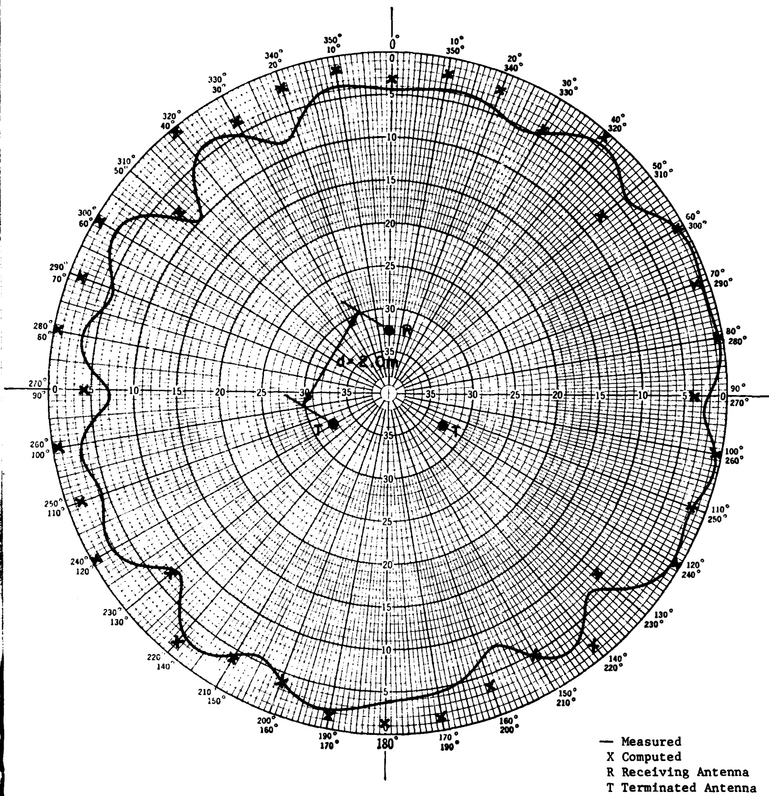
Figure 37. Three AS-1097/GR, f = 400 MHz, d = 2 m, D = 9.75 m
