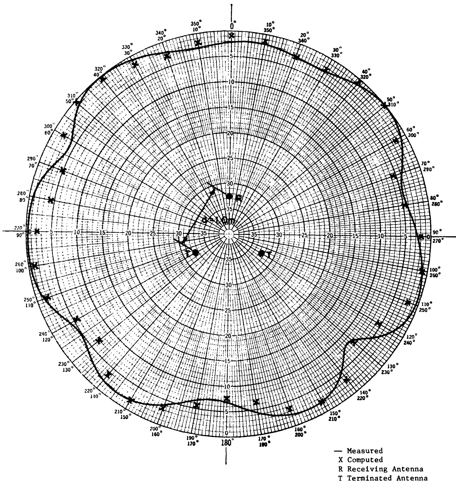
Figure 31. Three AS-1097/GR, f = 400 MHz, d = 1 m, D = 9.75 m
