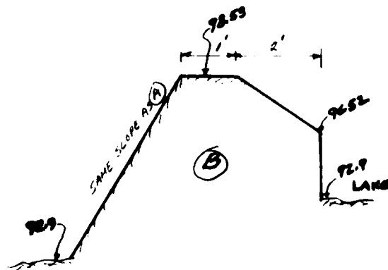
DAM SECTION
