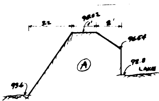
DAM SECTION
