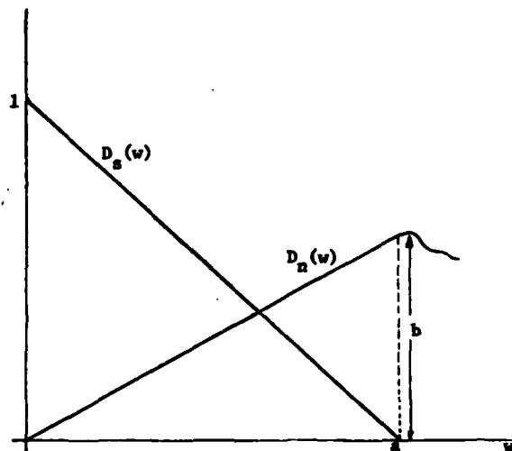
Figure 3 Example spectra of section IV
