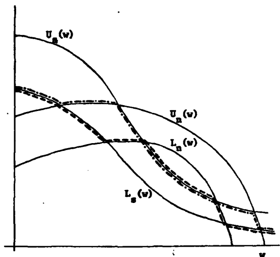
Figure 2 Illustration of functions defined in case 2A, section III — for A_s(w) --- for B_s(w)
