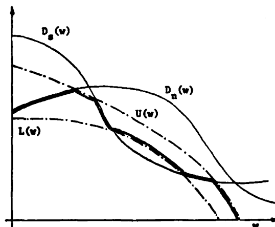
Figure 1 Worst-case |D_m^F| for case 1, section III
