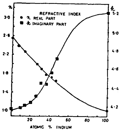
MEASURED OPTICAL CONSTANTS OF LEAD-INDIUM ALLOYS
