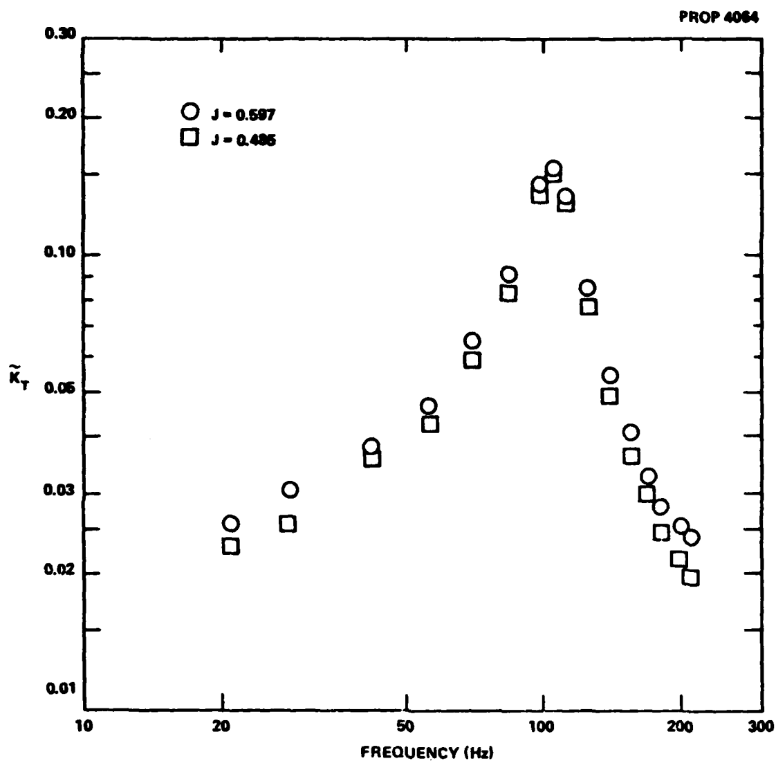
Figure 10 - Measured Unsteady Thrust for Prop. No. 4064
