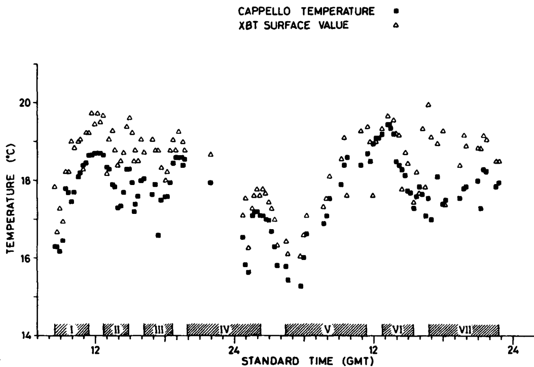
FIG. 4 SEA-SURFACE TEMPERATURE MEASURED BY THE XBTs AND THE "CAPPELLO" THERMISTOR (nominally 5 cm below surface). The numbered bars indicate the duration and number of the cruise leg as shown in Fig. 1
