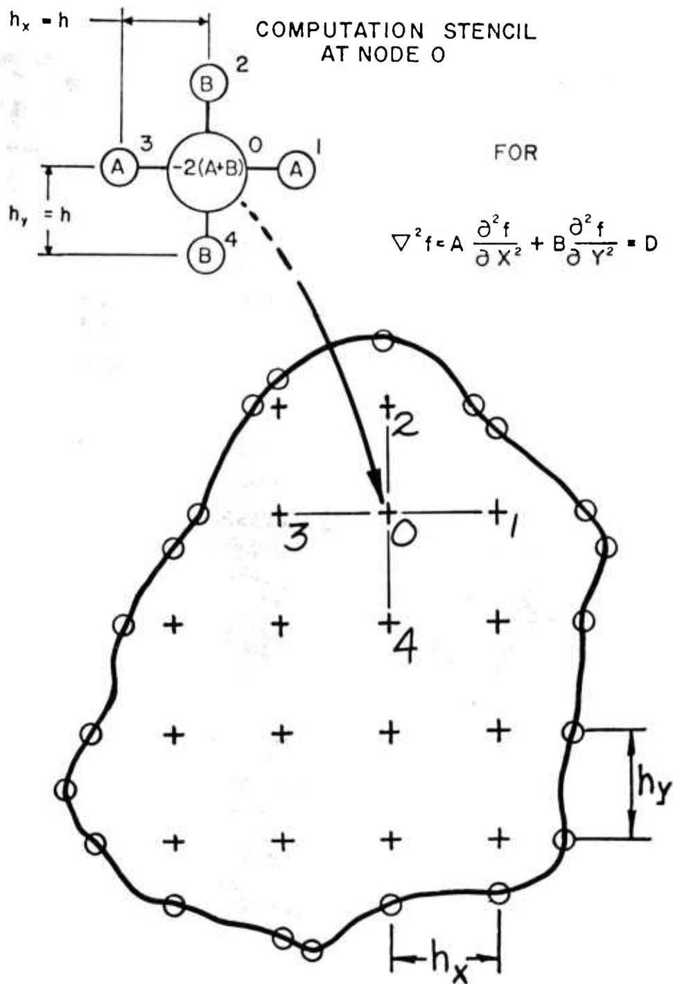
Figure A-4. Harmonic operator for square star in X-Y grid.
