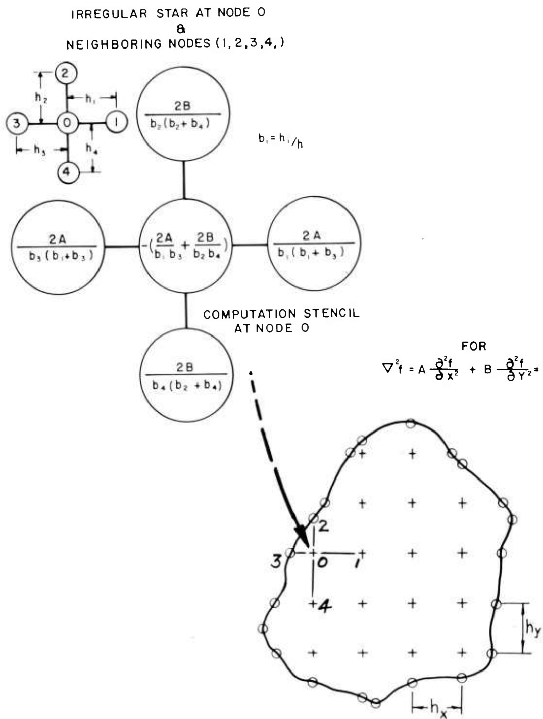
Figure A-5. Harmonic operator for irregular star in X-Y grid.
