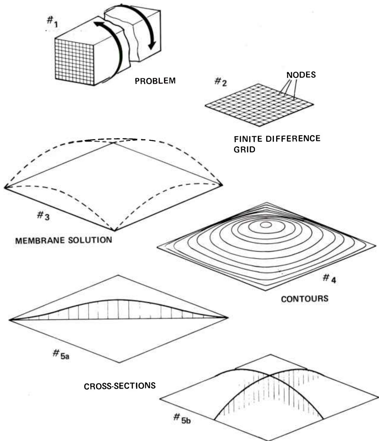
Figure 1. Membrane analogy.
