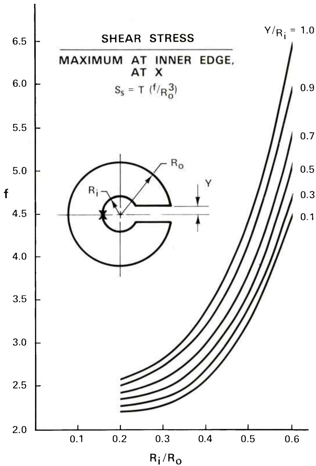
Figure 3. Split shaft, stress.
