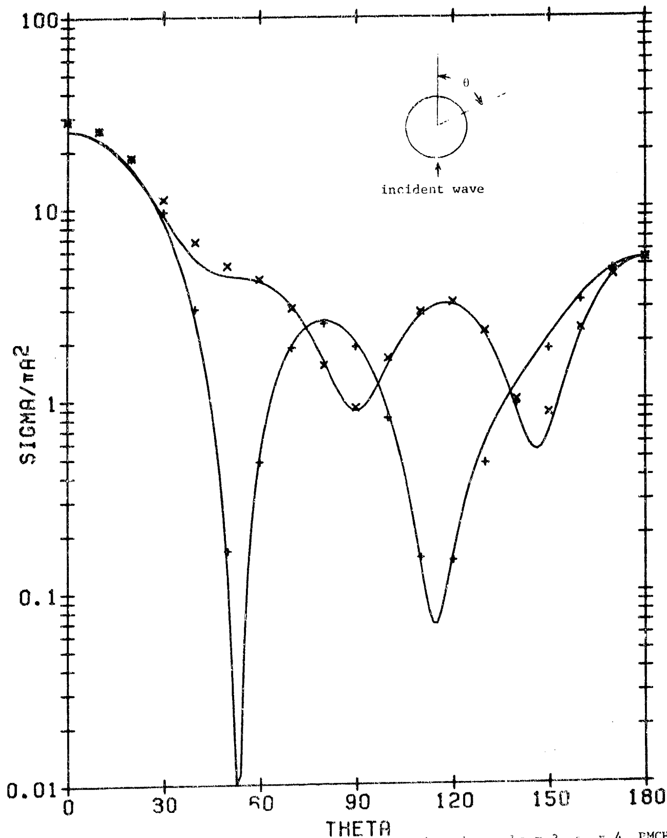
Fig. 10. Plane wave scattering patterns for dielectric sphere, ka = 3 , \epsilon_r = 4 , PMCHW solution. Symbols \times and + denote horizontal polarization and vertical polarization respectively. Solid line denotes exact solution.
