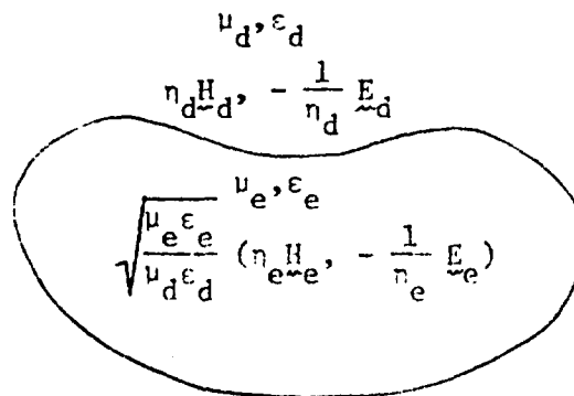
Fig. 5. Composite situation used to prove that (26) and (27) have only the trivial solution \underline{J} = \underline{M} = 0 .
