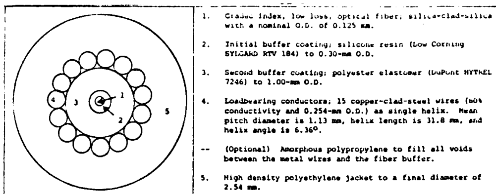
Figure 9. Cable A Composition
