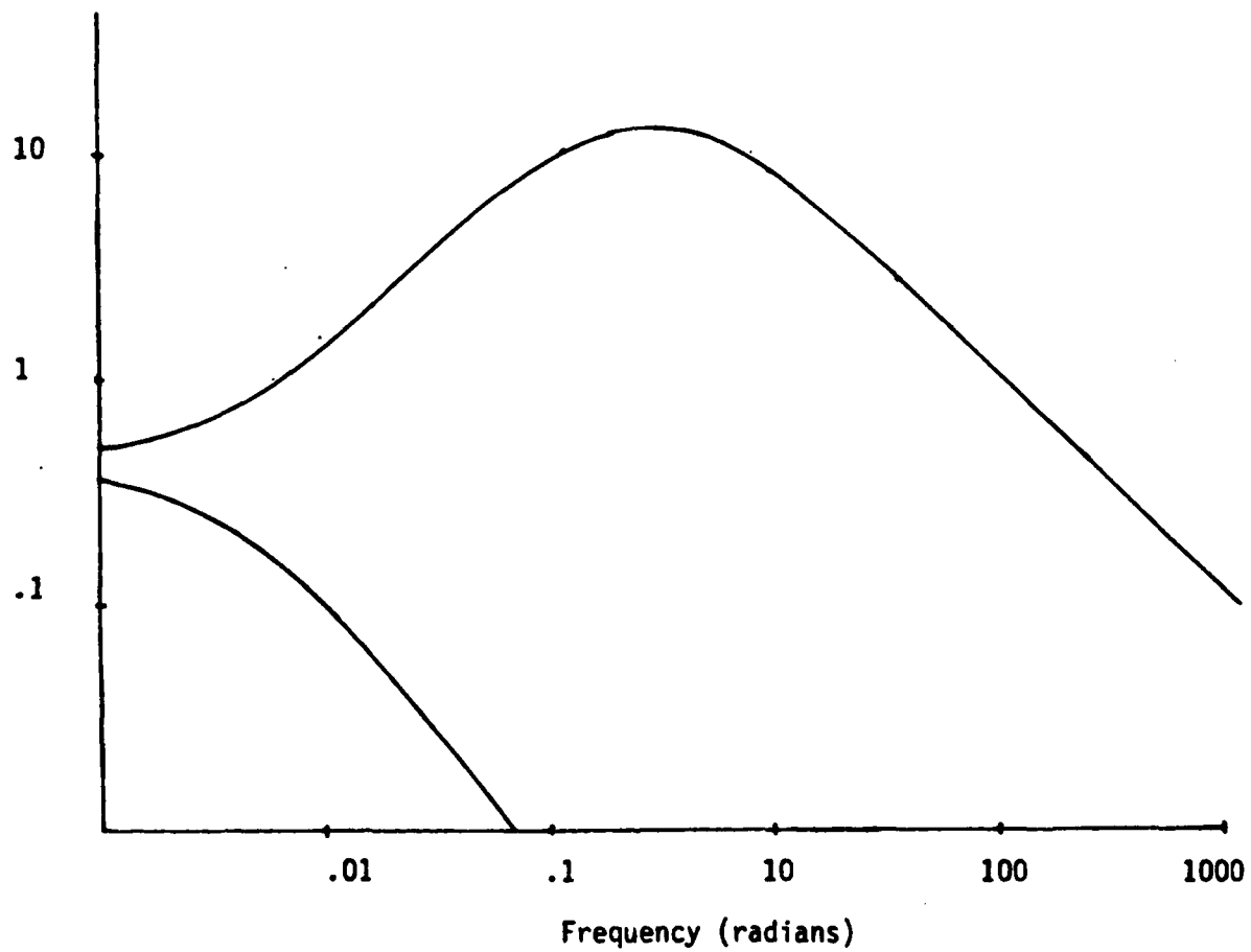
Fig. 10 Closed-Loop Frequency Response - 1/\sigma(1 + G^{-1})
