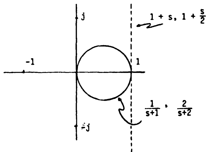
Fig. 7 Example 2 Nyquist and Inverse Nyquist Diagram
