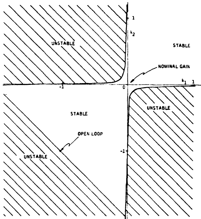
Fig. 6 Example 1 Stability Domain
