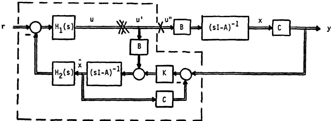
1B. Observer-Based Implementation
