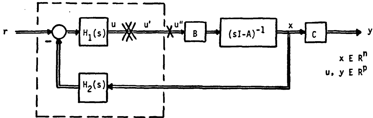
1A. Full-State Feedback Implementation
