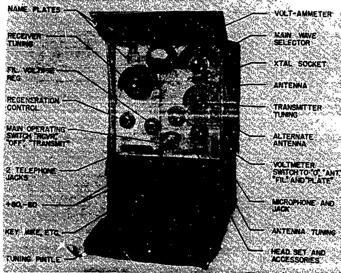
Transmitter-receiver 6-PK.
