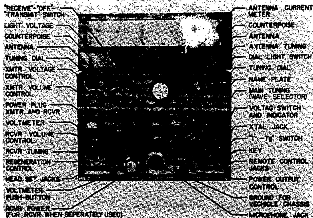
Transmitter-receiver 5-AK-1M.
