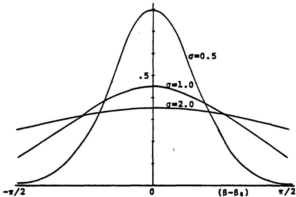
Figure III-3 Gaussian Spreading
