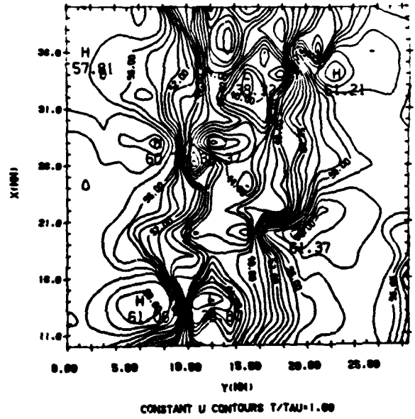
Figure 4.6 - Streamwise velocity contours of the wake of 2.0 mm cylinder.
