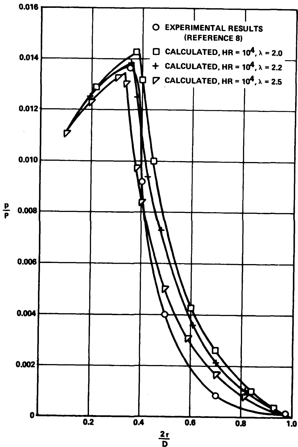
Figure 10. Surface Pressure Distributions, p_{i0} = 0.01108
