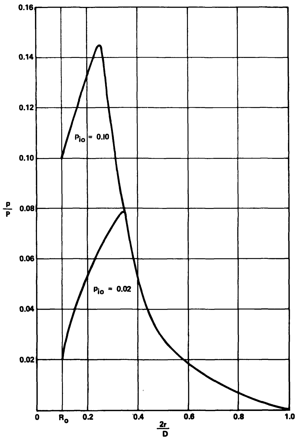
Figure 3. Surface Pressure Distributions for HR = 1,000 p_{i0} = 0.02 and 0.1
