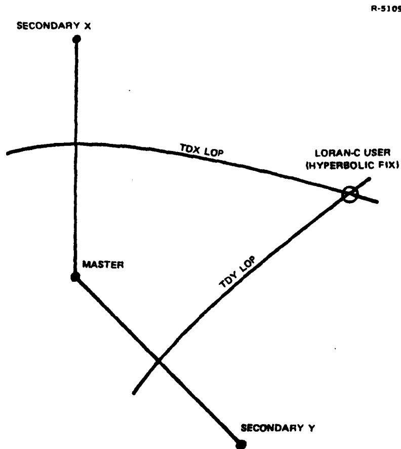
Figure 2.1-3 Hyperbolic Loran-C Position Fix
