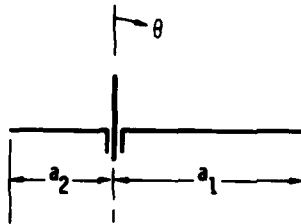
Fig. 5. Geometry of Monopole over Rectangular Ground Plane
