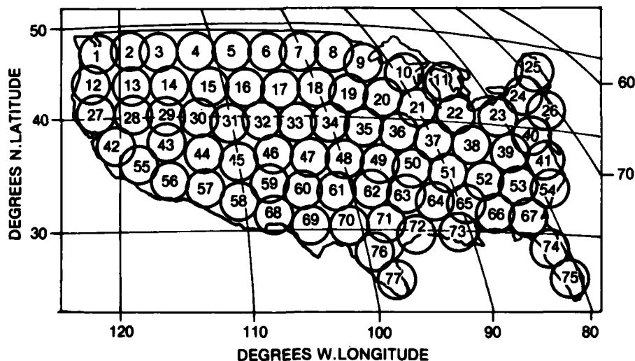
Figure 1 A scheme for spot beam ( 0.5^\circ beamwidth) coverage of the U.S. with 77 beams from geostationary orbit
