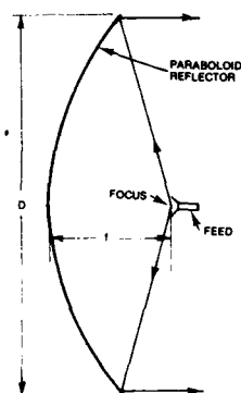
Figure 4(a) Centre fed parabolic reflector antenna concept
