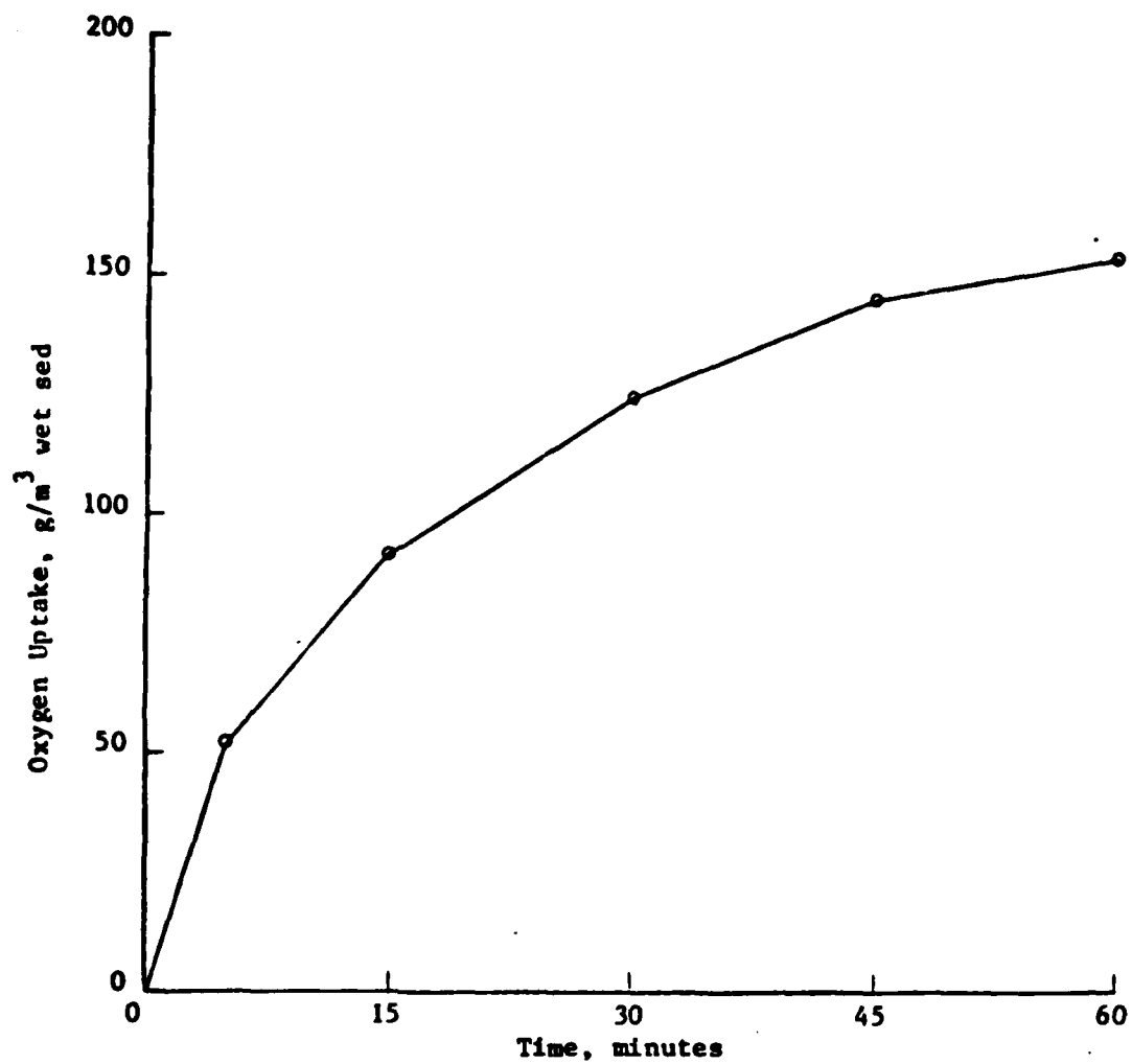
Figure 31. MEDIUM RATE OXYGEN UPTAKE RATE AT 25°C ( KEOKUK, M.P. 356 )
