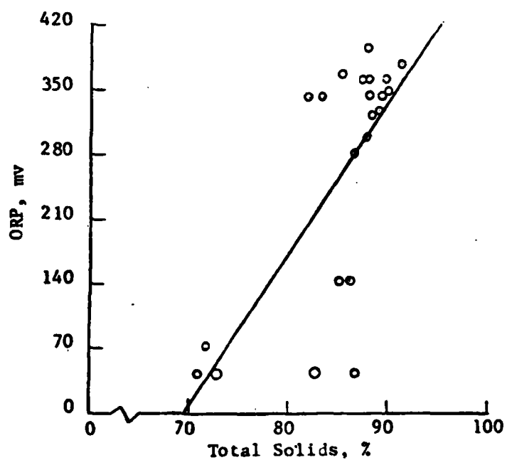
Figure 21. ORP VERSUS TOTAL SOLIDS
