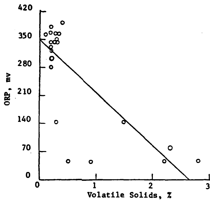
Figure 20. ORP VERSUS VOLATILE SOLIDS
