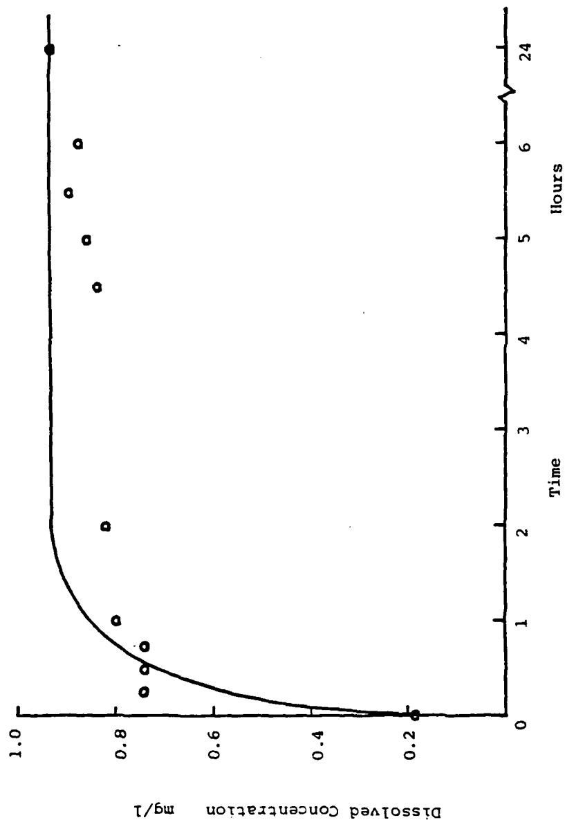
Figure 47. Ammonia at Grey Chute - 7.5^{\circ} \text{C} M.P. 356.
