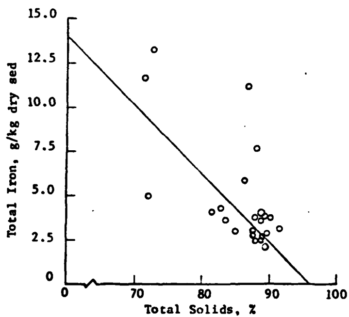
Figure 19. TOTAL IRON VERSUS TOTAL SOLIDS
