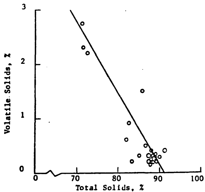
Figure 25. VOLATILE SOLIDS VERSUS TOTAL SOLIDS
