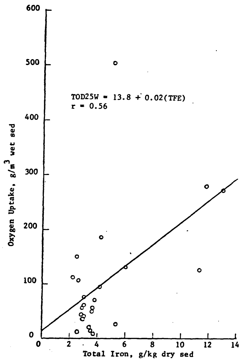
Figure 14. OXYGEN UPTAKE VERSUS SEDIMENT TOTAL IRON. TEMPERATURE = 25°C
