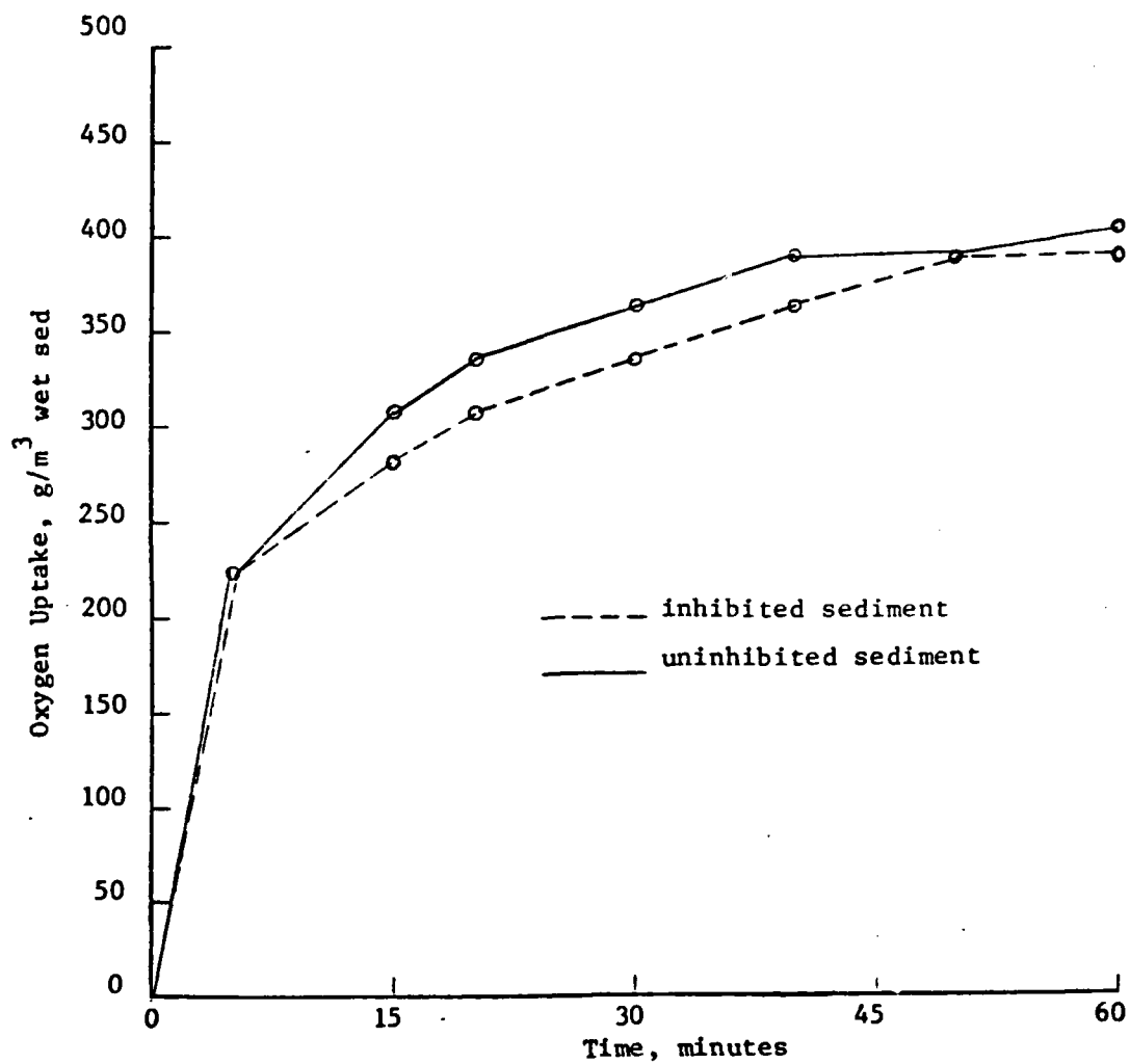
Figure 26. INFLUENCE OF BIOLOGICAL ACTIVITY ON OXYGEN UPTAKE
