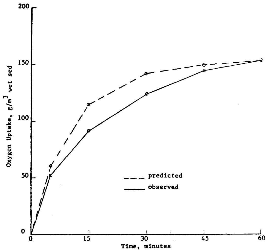
Figure 33. OBSERVED OXYGEN UPTAKE AT 25°C VERSUS OXYGEN UPTAKE PREDICTED BY TOD_t = TOD_u (1 - e^{-kt}) . KEOKUK, M.P. 356
