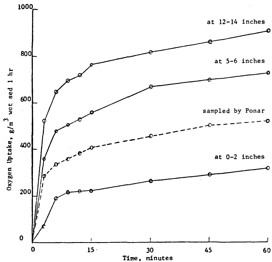
Figure 27. OXYGEN UPTAKE AT DIFFERENT DEPTHS
