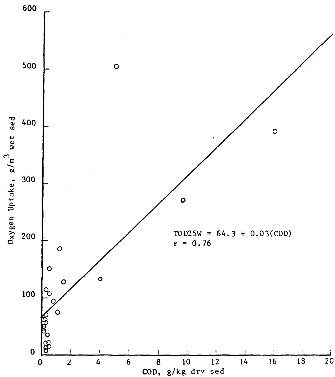
Figure 13. OXYGEN UPTAKE VERSUS SEDIMENT COD. TEMPERATURE = 25°C
