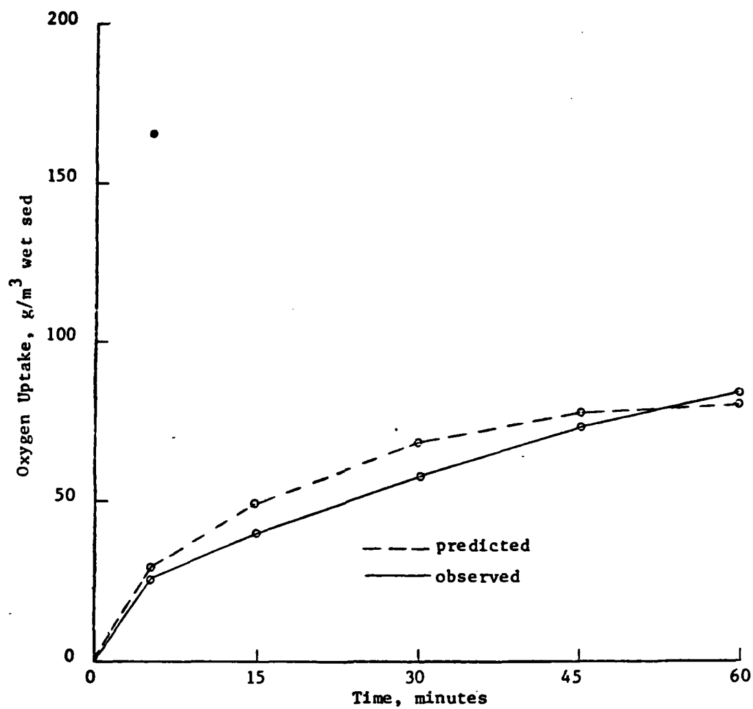
Figure 34. OBSERVED OXYGEN UPTAKE AT 25°C VERSUS OXYGEN UPTAKE PREDICTED BY \text{TOD}_t = \text{TOD}_u (1 - e^{-kt}) . MUSCATINE, M.P. 447
