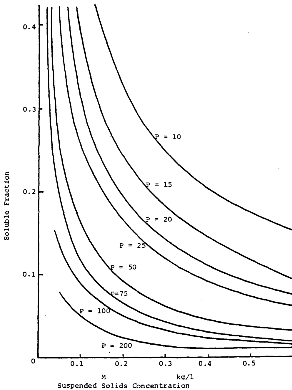
Figure 42. Soluble Fraction Vs. Suspended Solids Concentration
