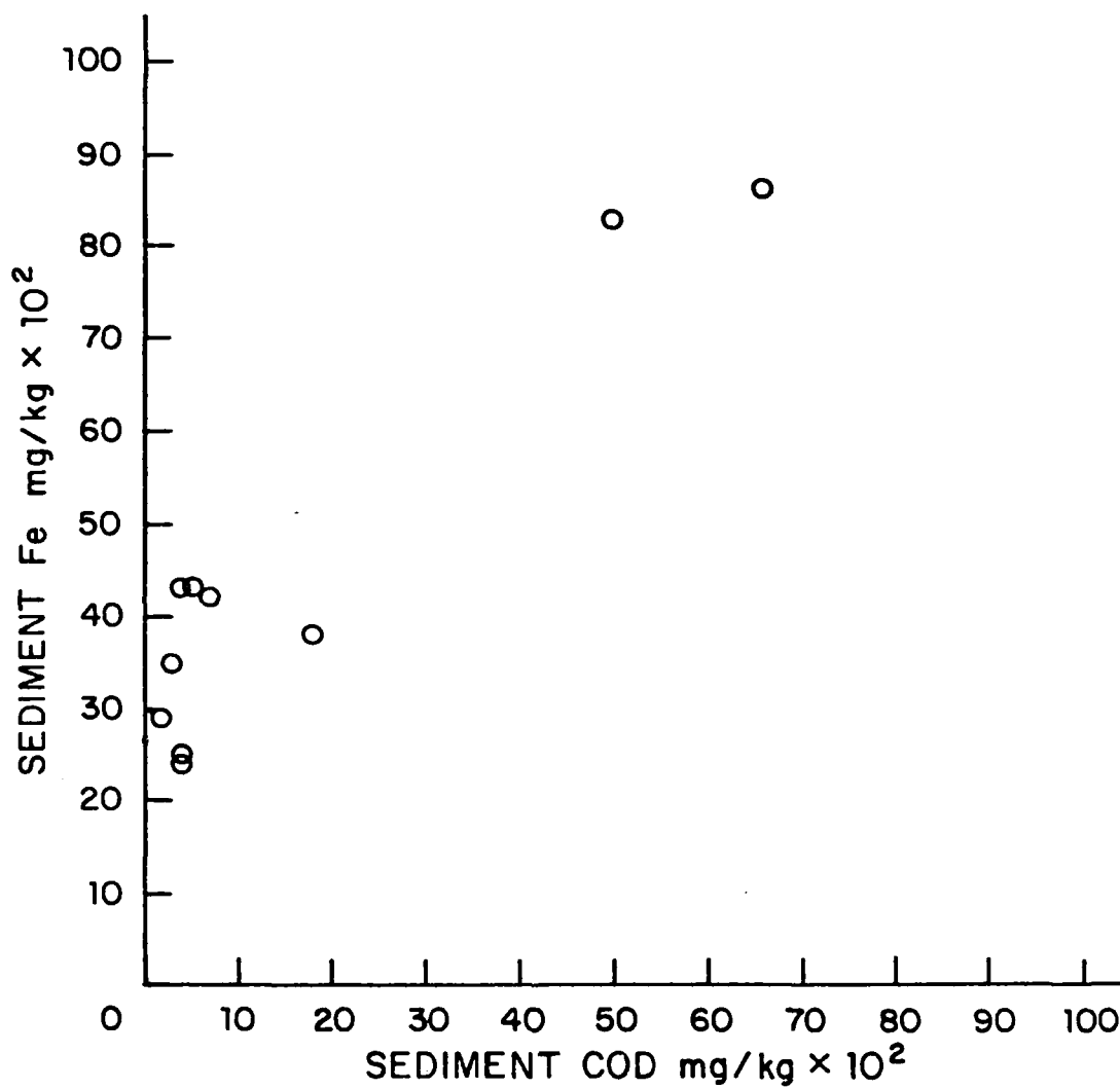
Figure 6. Sediment Iron Concentration vs. Chemical Oxygen Demand
