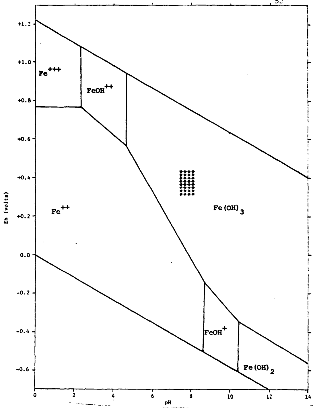
Figure 9. Eh - pH Diagram for the Iron-Water System: Iron = 2.8 \times 10^{-6} M.
