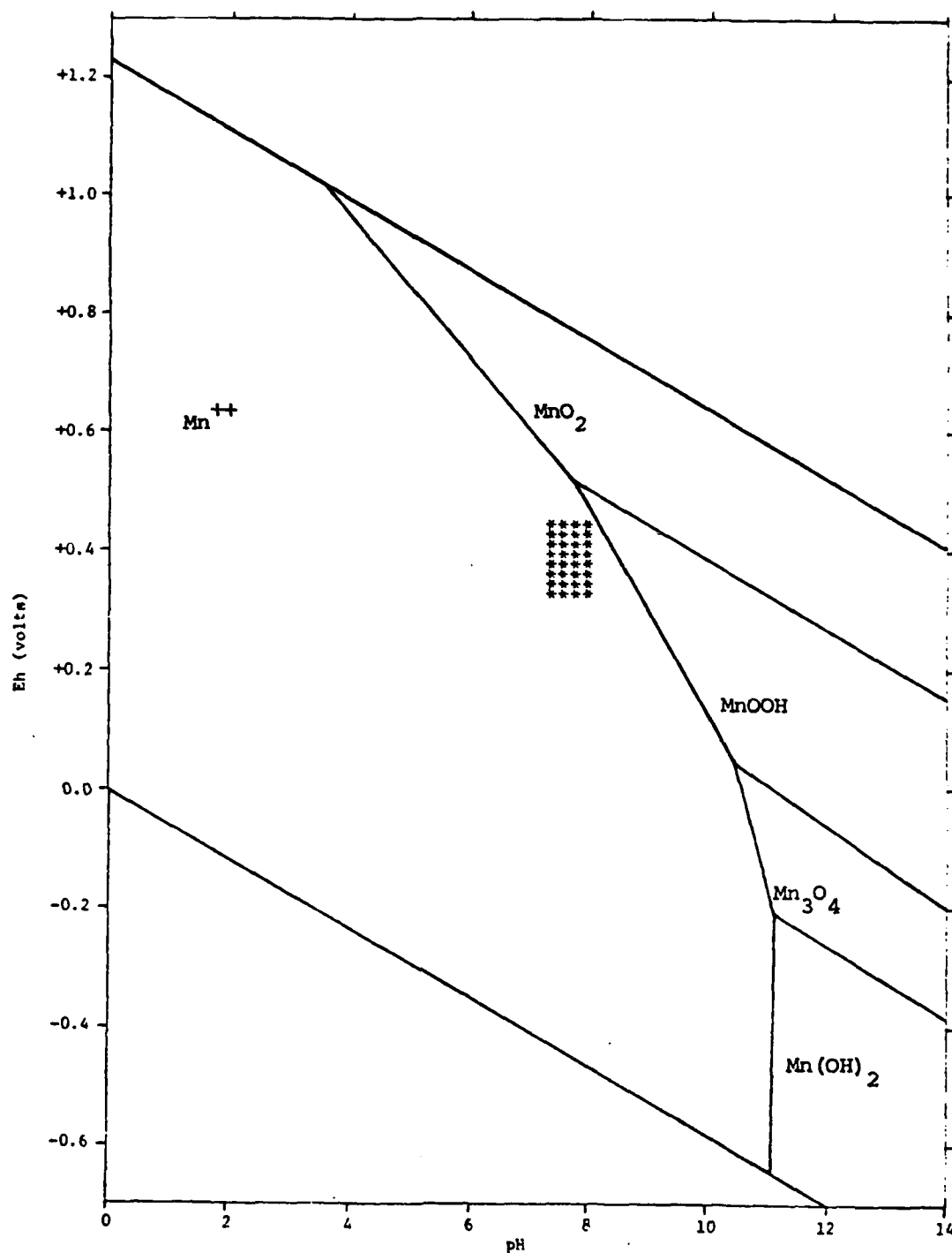
Figure 10. Eh-pH Diagram for the Manganese-Water System: Manganese = 8.2 \times 10^{-8} M.
