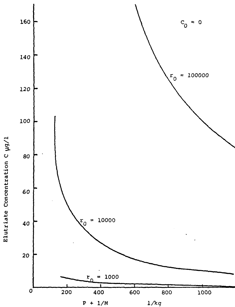
Figure 40. Elutriate Concentration Vs. P + 1/M
