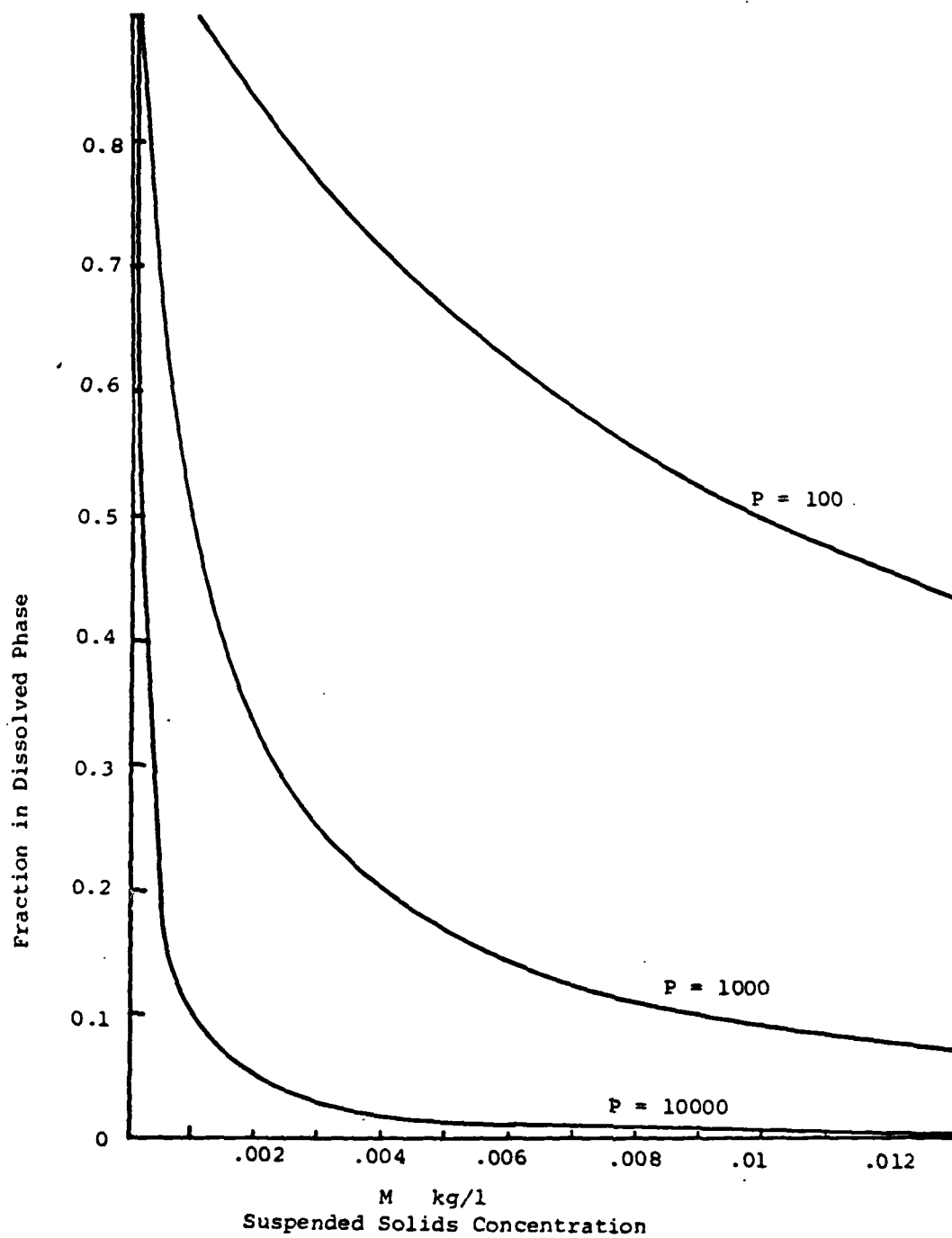
Figure 37. Fraction in Dissolved Phase Vs. Suspended Solids Concentration
