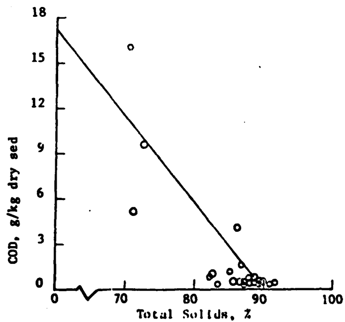
Figure 23. COD VERSUS TOTAL SOLIDS
