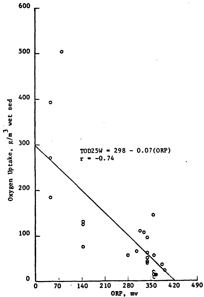
Figure 15. OXYGEN UPTAKE VERSUS SEDIMENT ORP. TEMPERATURE = 25°C
