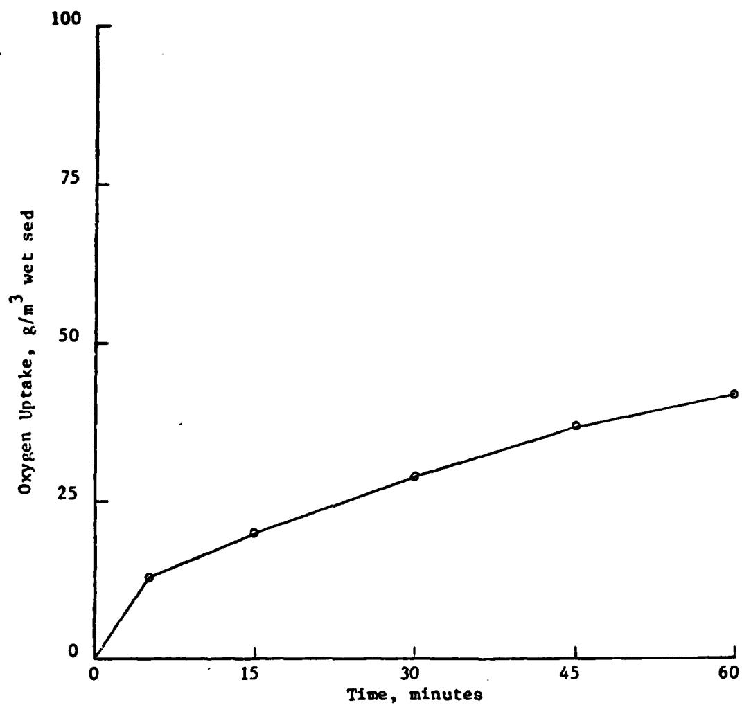
Figure 32. LOW RATE OXYGEN UPTAKE AT 25°C ( MUSCATINE, M.P. 447 )
