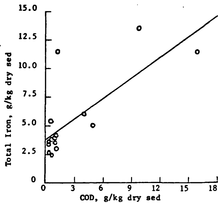
Figure 24. TOTAL IRON VERSUS COD
