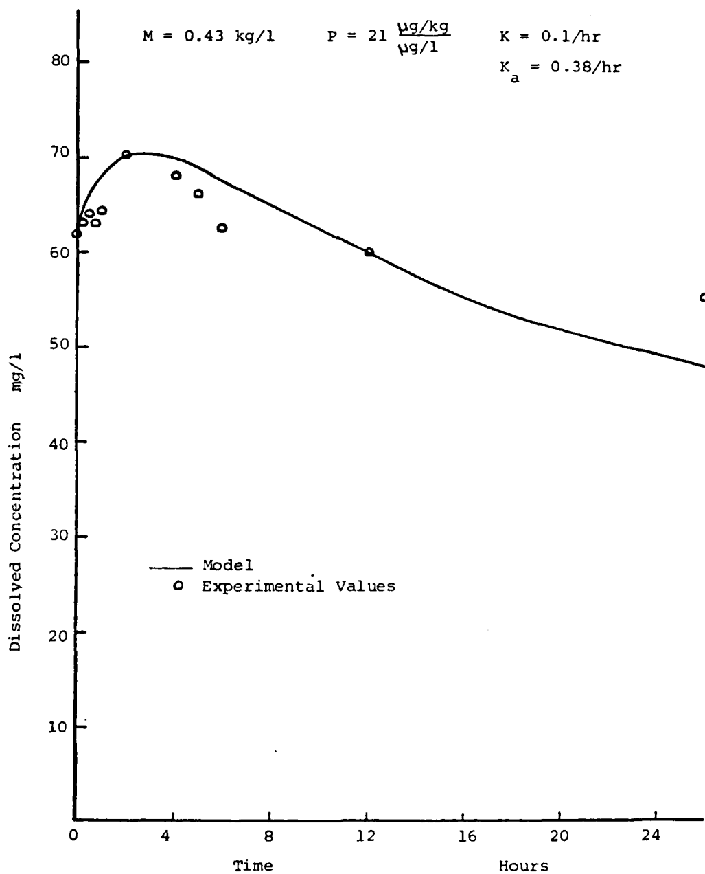
Figure 50. COD at Keokuk - 8^{\circ} - 18^{\circ} C M.P. 356.
