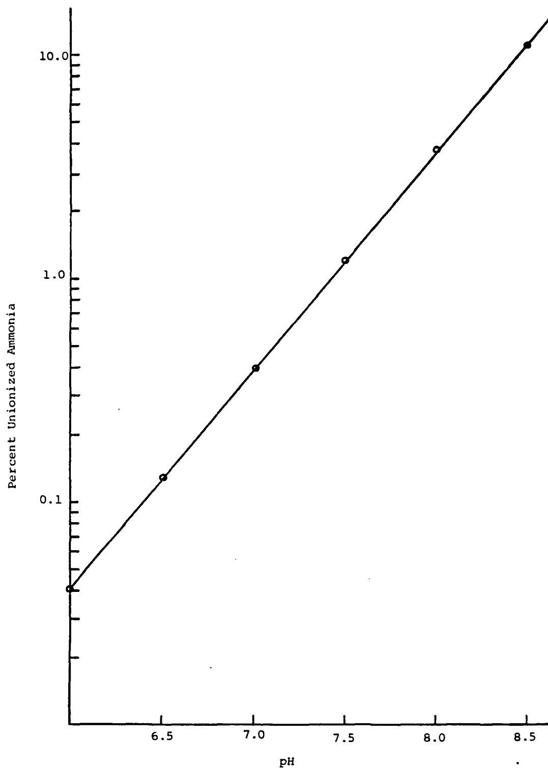
Figure 44. Percent Unionized Ammonia Vs. pH
