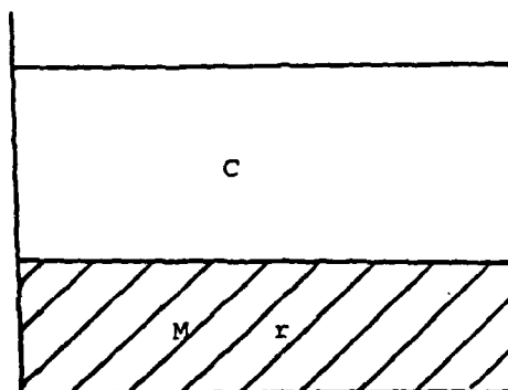
Equilibrium 4:1 :: Water:Sediment T = 90 minutes
