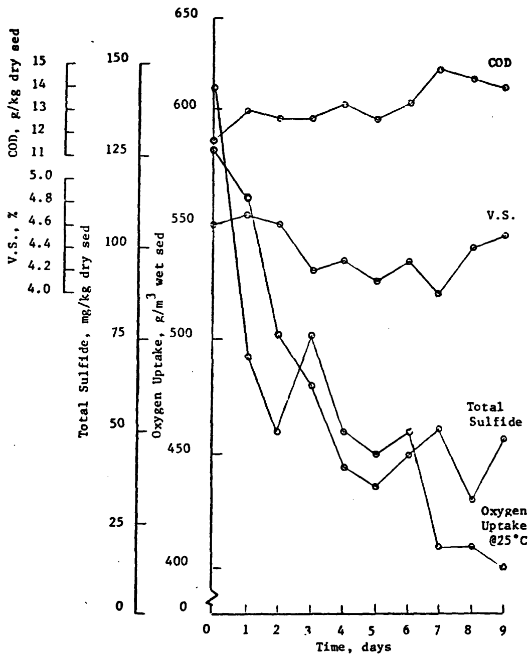
Figure 29. EFFECT OF STORAGE TIME ON SEDIMENT CHARACTERISTICS
