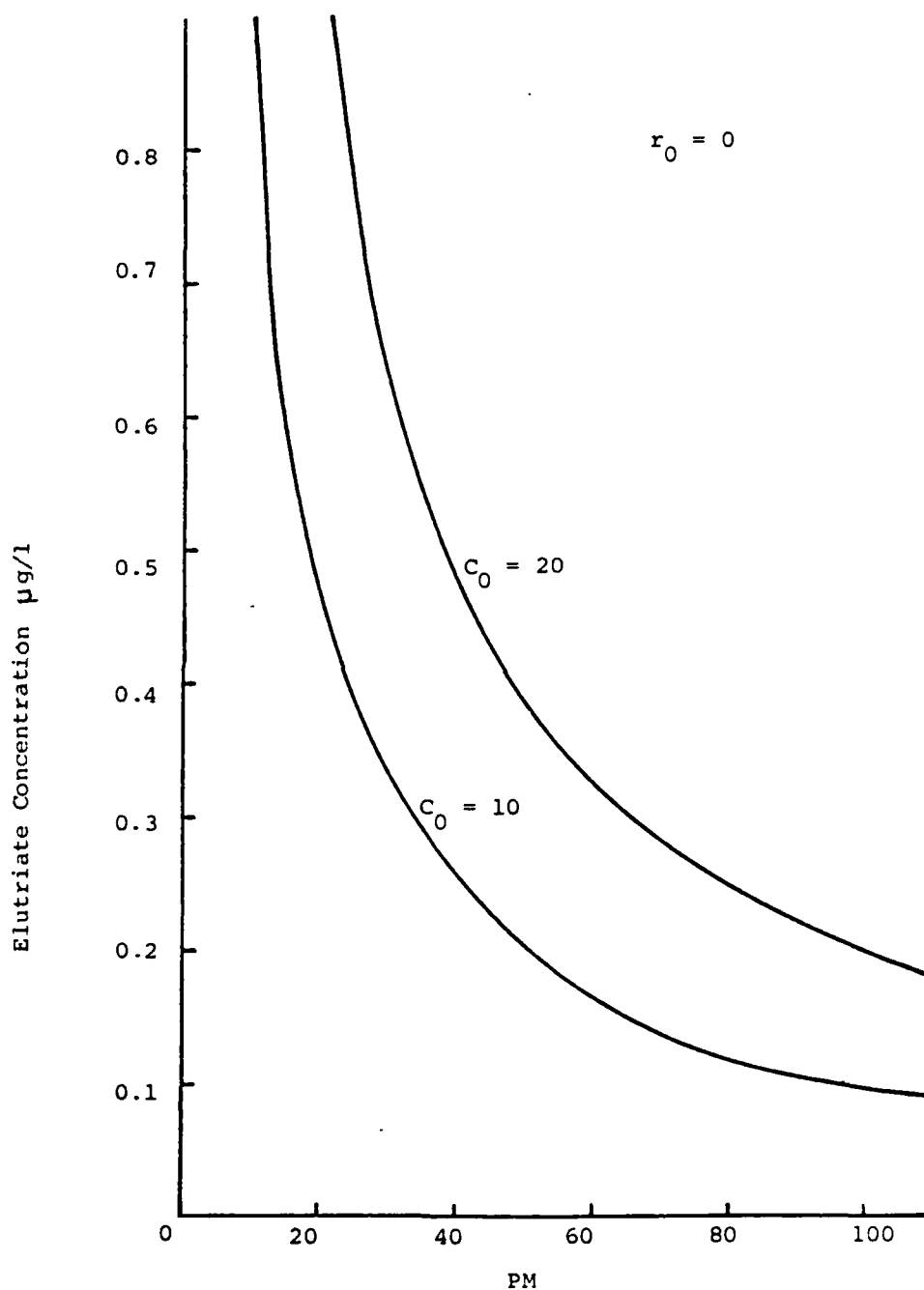
Figure 41. Elutriate Concentration Vs. PM
