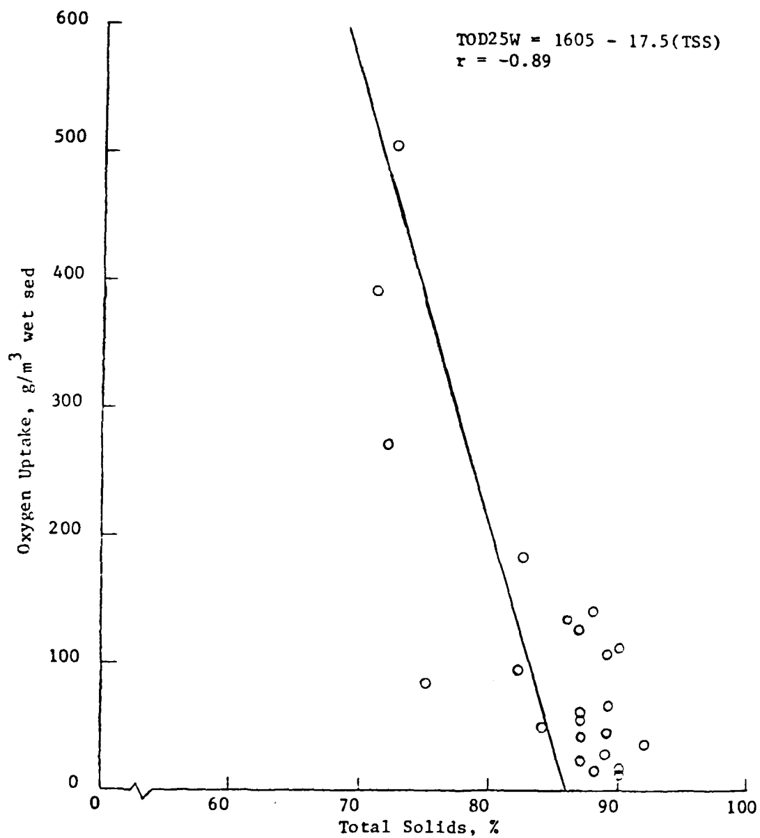
Figure 12. OXYGEN UPTAKE VERSUS SEDIMENT TOTAL SOLIDS. TEMPERATURE = 25°C
