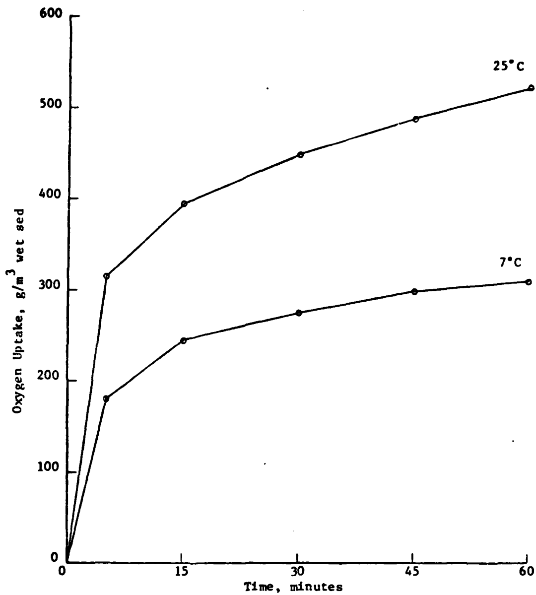
Figure 30. HIGH RATE OXYGEN UPTAKE AT 25°C AND 7°C ( GREYS CHUTE, M.P. 356 )
