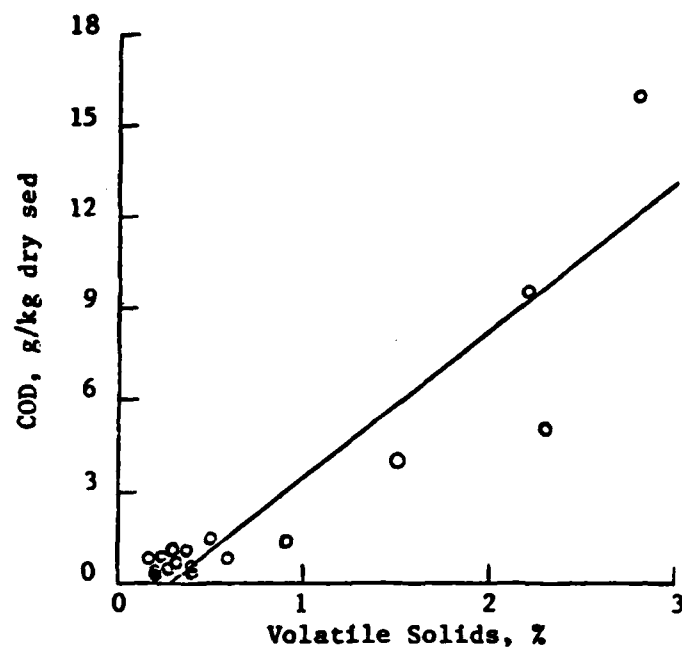
Figure 22. COD VERSUS VOLATILE SOLIDS
