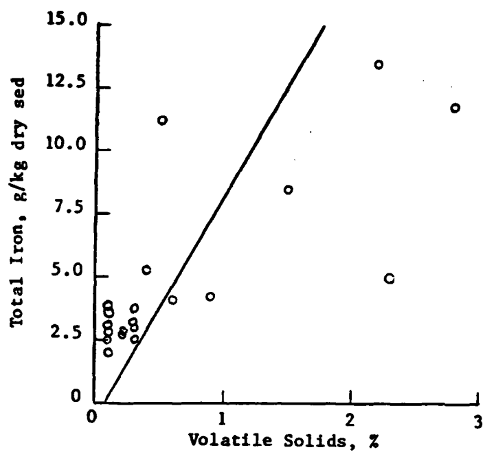
Figure 18. TOTAL IRON VERSUS VOLATILE SOLIDS
