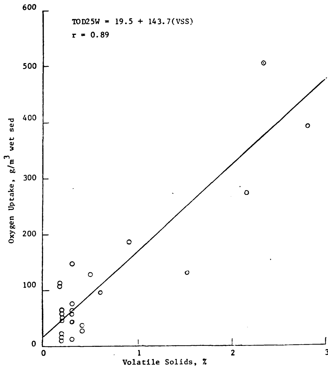
Figure 11. OXYGEN UPTAKE VERSUS SEDIMENT VOLATILE SOLIDS. TEMPERATURE = 25°C
