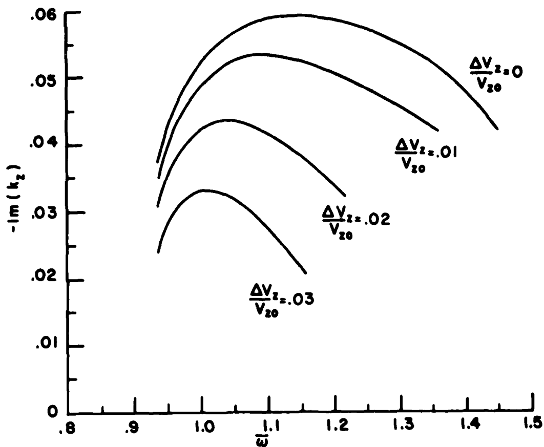
Fig. 3 — \text{Im}(\bar{k}_z) vs \bar{\omega} for different values of velocity spread at a fixed magnetic field ( \Omega_0/\gamma_0 = .72 ). Parameters used: n = s = 1 , \gamma_0 = 1.062 , \bar{v}_{10}/\bar{v}_{z0} = 1.35 , \bar{v}_{z0} = .2 , \nu = .002 , \bar{d} = .6 , \epsilon_r = 20 , \bar{L}_z = 2\bar{d} .
