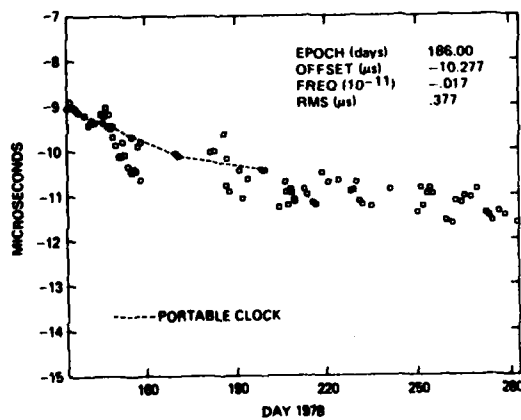
Fig. 6 - Time transfer results from the Institute for Applied Geodesy, Wettzell, West Germany (USNO,MC1)-(IFAG)
