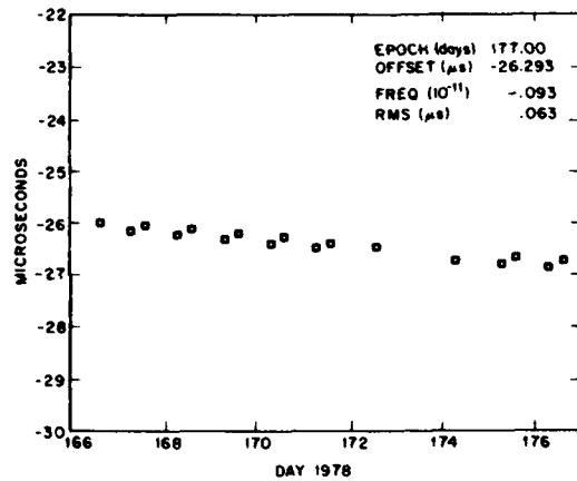
Fig. 14 — Panama results (12 day segment)
