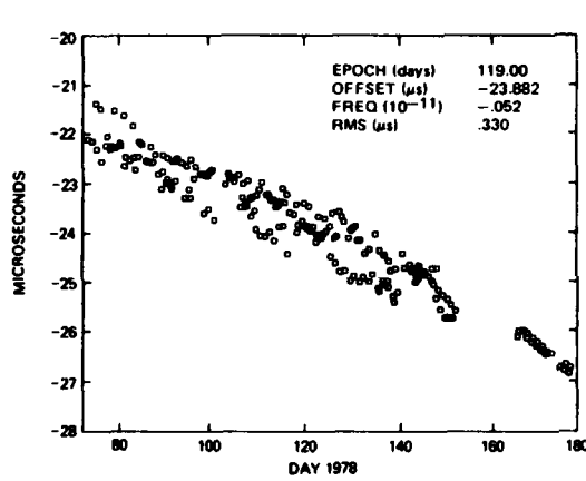
Fig. 13 — Time transfer results from Panama USNO,MC1)-(PMA)
