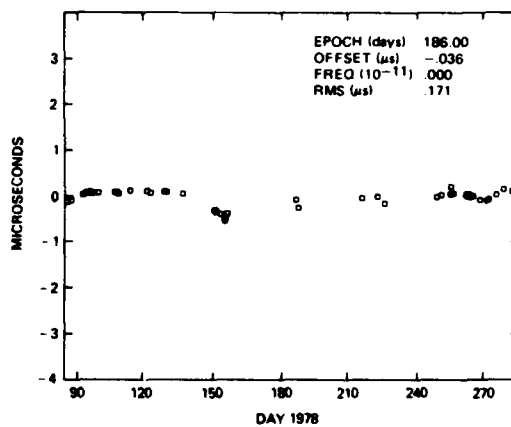
Fig. 12 — Time transfer results from USNO (USNO,MC1)-(USNO,MC1,NTS)
