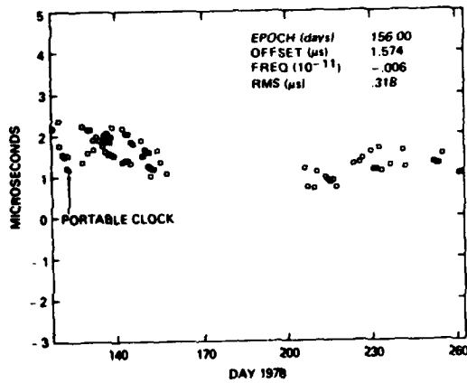
Fig. 4 - Time transfer results from Paris OP (USNO,MC1)-(OP)
