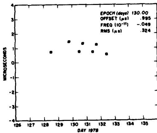
Fig. 5 - Time transfer results from Cerga, France (USNO,MC1)-(CERGA)
