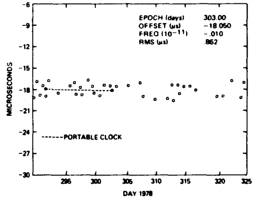
Fig. 8 — Time transfer results from RRL, Japan (USNO,MC1)-(RRL)
