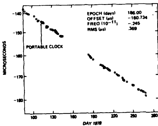
Fig. 3 - Time transfer results from Royal Greenwich Observatory (USNO,MC1)-(RGO,JP)
