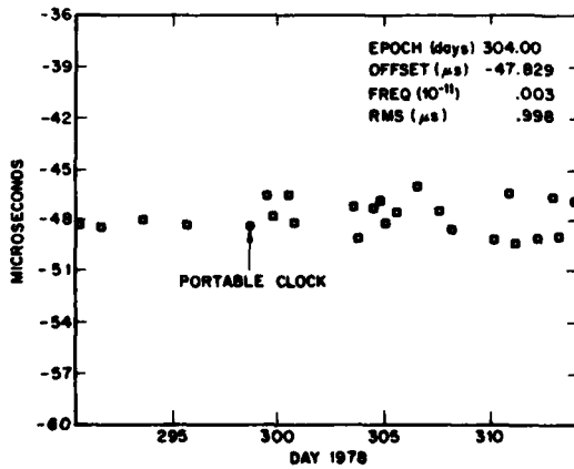
Fig. 9 — Time transfer results from NRLM, Japan (USNO,MC1)-(NRLM)
