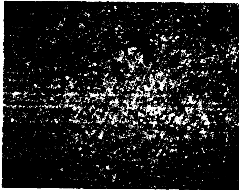
Figure 14. Micrograph Of 650 C Rolled 52100. The fine microstructure is a result of the rolling process. 1000X
