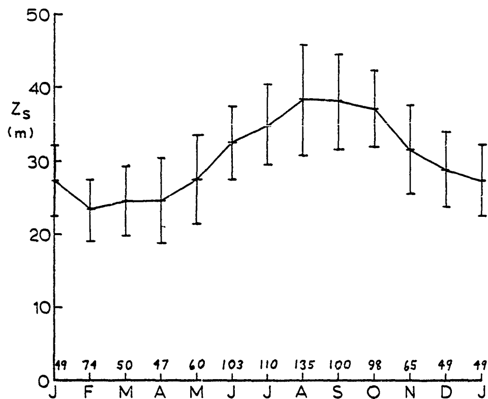
FIGURE 18 : SOUTH OF JAPAN (N 29° E 135°)
