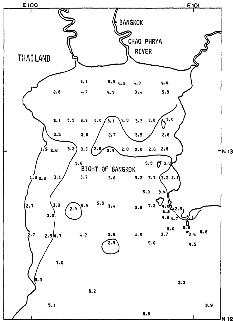
FIGURE 72 : KD VALUES, BANGKOK APPROACHES, NOV-MAR
