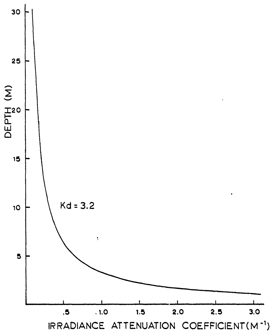
FIGURE 6: PENETRATION CAPABILITY OF A LASER BATHYMETRY SYSTEM WITH K_d = 3.2
