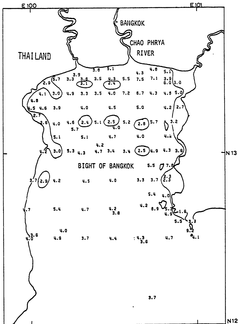
FIGURE 71 : KD VALUES, BANGKOK APPROACHES, APR-OCT
