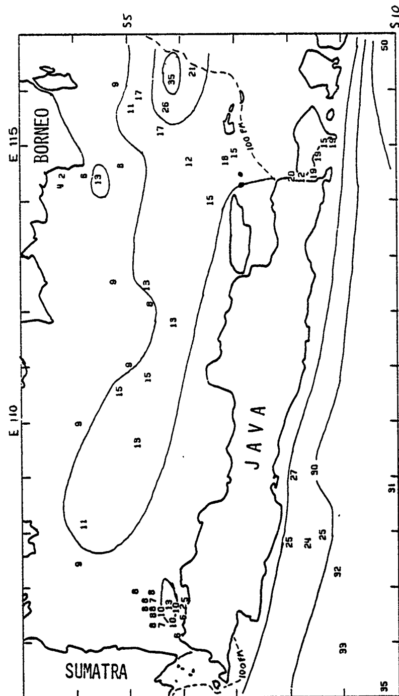
FIGURE 25 : SECCHI DEPTHS, JAVA SEA, JAN-MAR
