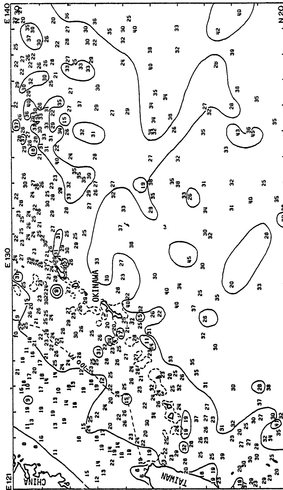
FIGURE 55 : SECCHI DEPTHS, PHILIPPINE SEA AND PACIFIC OCEAN (20°N - 30°N), APR-JUN
