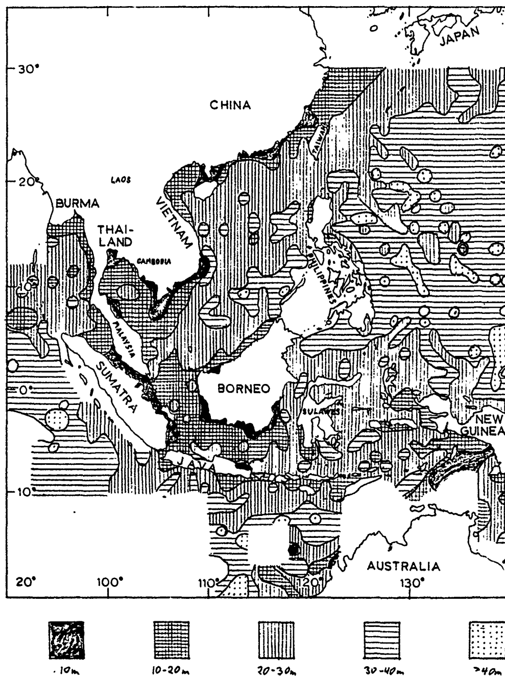
FIGURE 60 : SECCHI DEPTHS, SOUTHEAST ASIAN AND INDONESIAN WATERS
