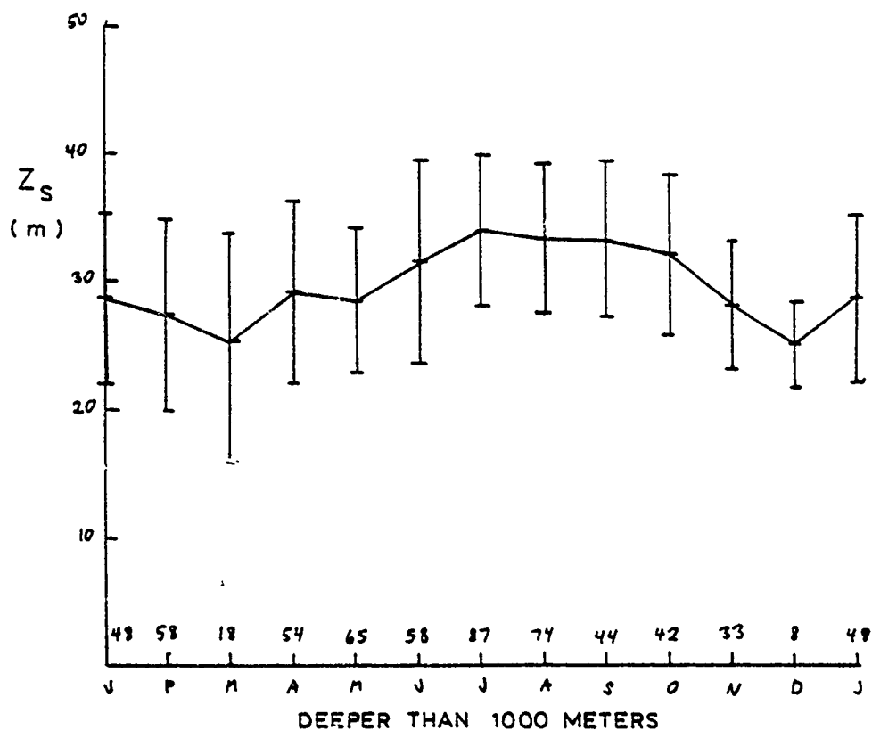
FIGURE 19 : PACIFIC OCEAN ( 20^\circ\text{N} - 30^\circ\text{N} )
