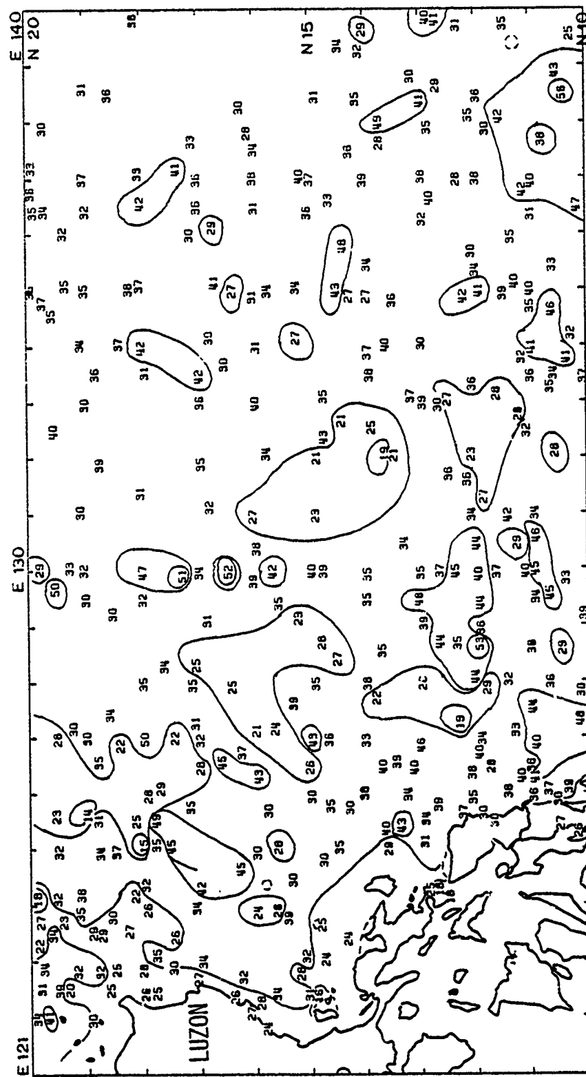
FIGURE 58 : SECCHI DEPTHS, PHILIPPINE SEA AND PACIFIC OCEAN (10°N - 20°N), ENTIRE YEAR
