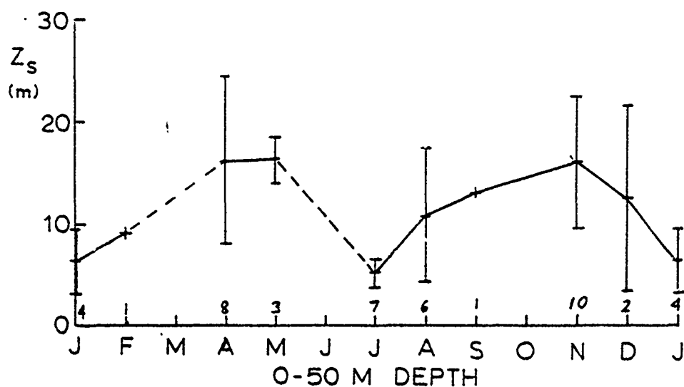
FIGURE 15 : JAVA SEA (EXCLUDING JAKARTA APPROACHES) Secchi depths (meters) The number of data points in each month appears along the abscissa.
