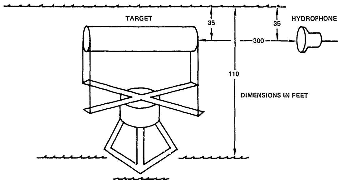
Figure 1. Target rotator.
