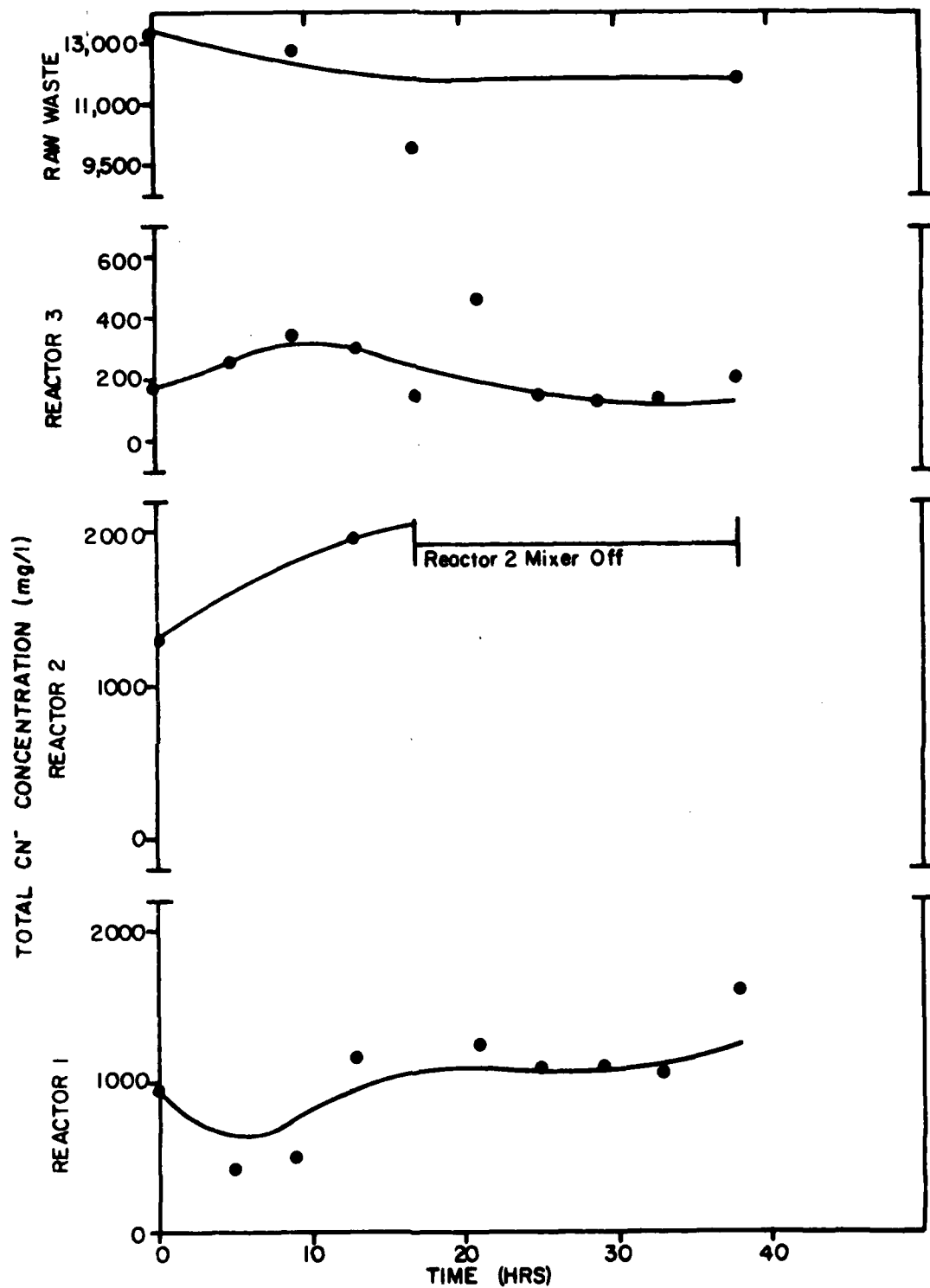
Figure 17 Treatment of \text{CN}^- waste with continuous inflow
