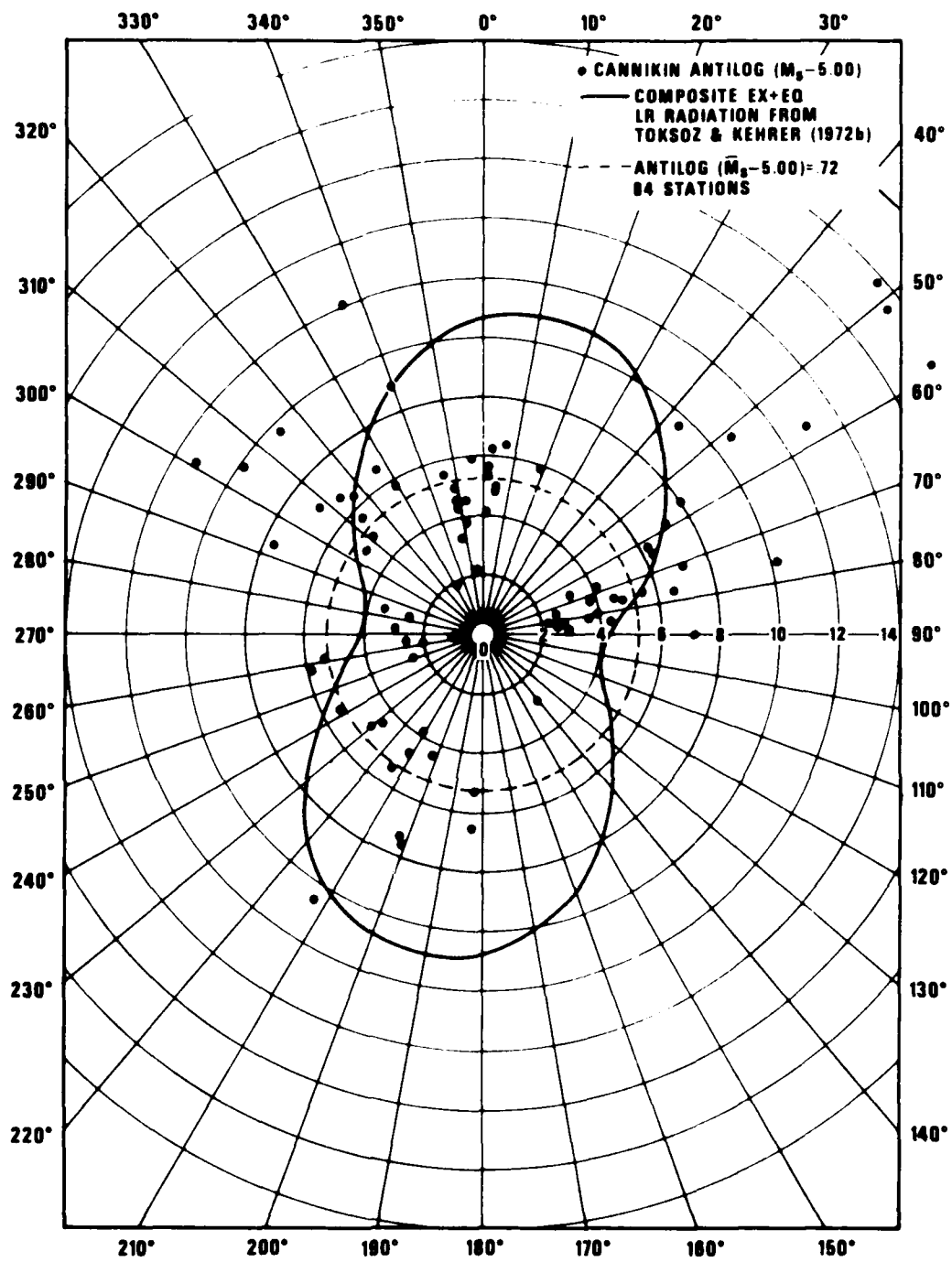
Figure 8 Azimuthal plot of CANNIKIN WWSSN M_s estimates.
