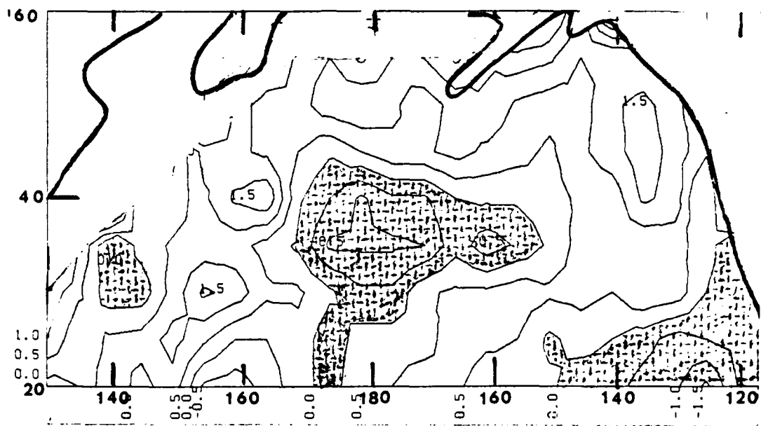
Figure 51. SST anomaly change from September 1976 to March 1977. Contour intervals are 0.5°C. Shaded areas indicate negative SST anomaly development.
