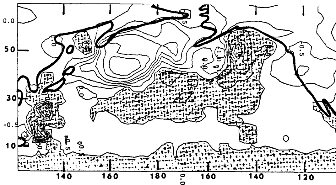
Figure 52. Filtered u_*^3 anomalies averaged from mid-September 1976 to mid-March 1977. Contour intervals are 0.5 \times 10^4 (cm/sec) 3 . Shaded areas indicate above normal storminess.
