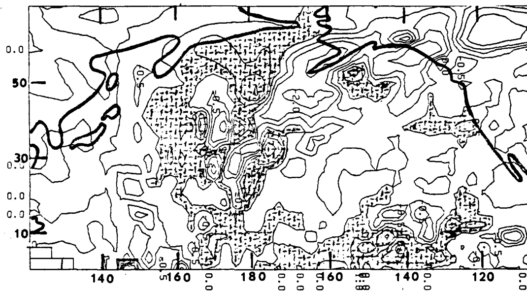
Figure 53. Filtered curl z τ anomalies averaged over the period mid-September 1976 to mid-March 1977. Contour intervals are 0.5 \times 10^{-9} dynes/cm 3 . Shaded areas indicate above normal curl z τ values.
