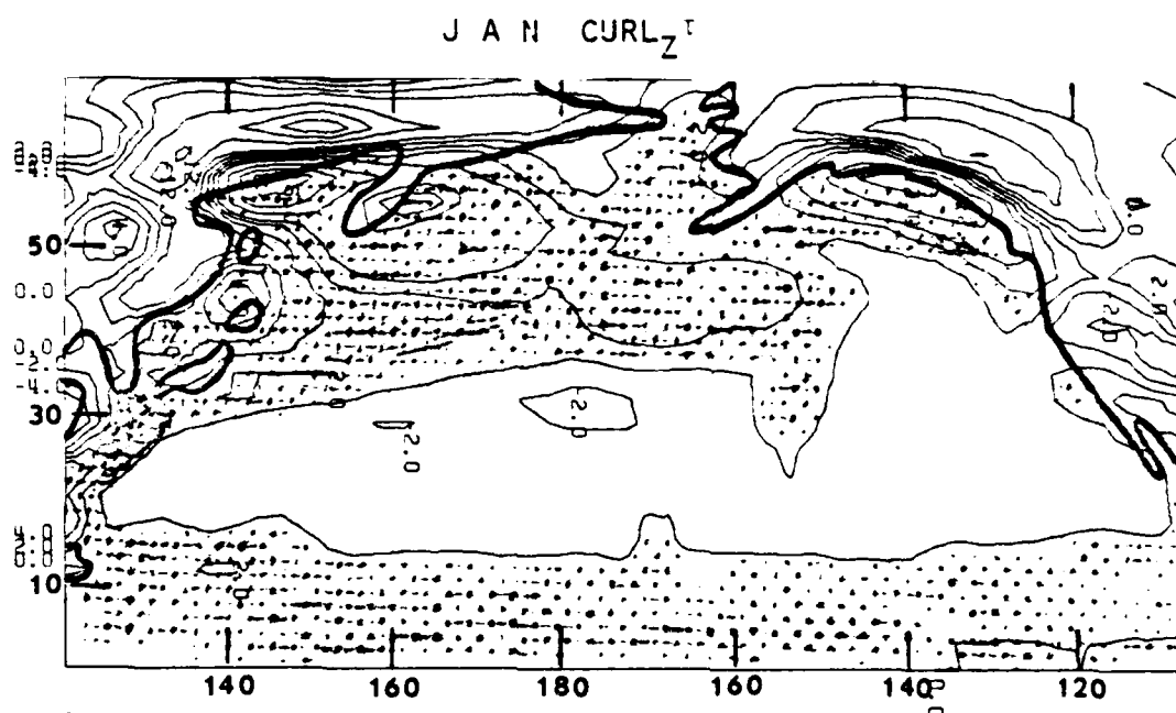
Figure 27. Climatological values of the vertical components of wind stress curl ( \text{Curl}_Z^T ) from total u and v wind components. Contour values are -16.0, -12.0, -8.0, -4.0, -2.0, 0.0, 2.0, 4.0, 8.0, 12.0, 16.0 \times 10^{-8} dynes/cm 2 . Shaded areas indicate positive curl.
