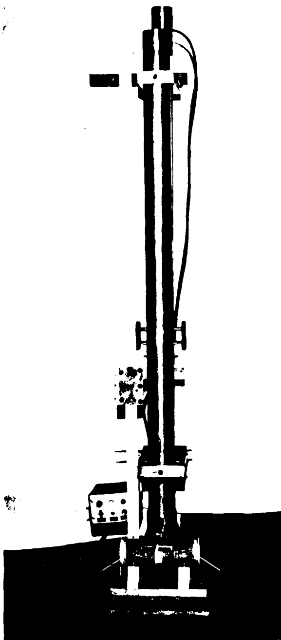
Figure 16. Falling tup impact tester with specimen.
