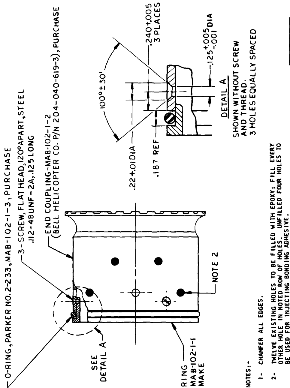
Figure E-3. End coupling assembly.
