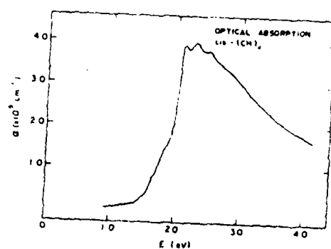
Fig. 3b. Absorption coefficient as a function of frequency; cis -(CH) x (ref. 29).
