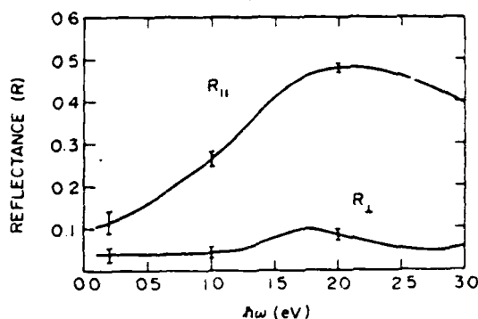
Fig. 4. Polarized reflectance as a function of frequency from partially oriented (CH)_x ( l/l_0=2.5 ). R_{||} and R_{\perp} refer to light polarization parallel and perpendicular to the orientation direction (ref. 29).
