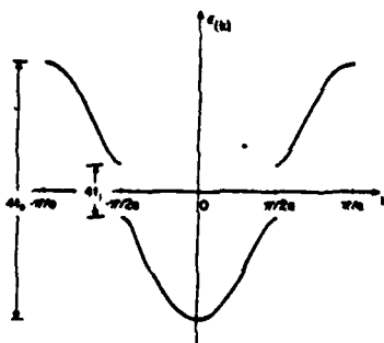
Fig. 2. Band structure of perfectly dimerized (\text{CH})_x .
