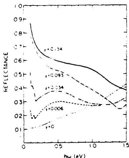
Fig. 16. Reflectance ( R_{||} ) for oriented [\text{CH}(\text{AsF}_5)_y]_x (ref. 42).
