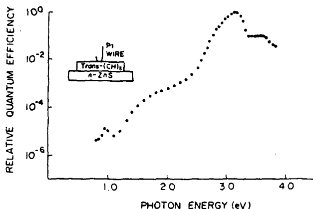
Fig. 7. Photoresponse of n-ZnS:undoped trans-(CH) x n-p heterojunction. Quantum efficiency normalized to 3.1 eV peak where the absolute quantum efficiency is of order unity. (ref. 18).
