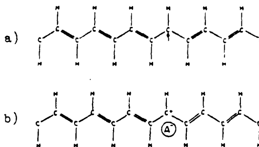
Fig. 10. a. Neutral soliton defect in \text{trans}-(\text{CH})_x (paramagnetic). b. Soliton kink after charge transfer (diamagnetic).
