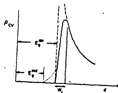
Fig. 3c. The joint optical density of states corresponding to the band structure of Fig. 10(a). The rounding of the square-root singularity arises from interchain coupling ( W_1 ) (ref. 29).
