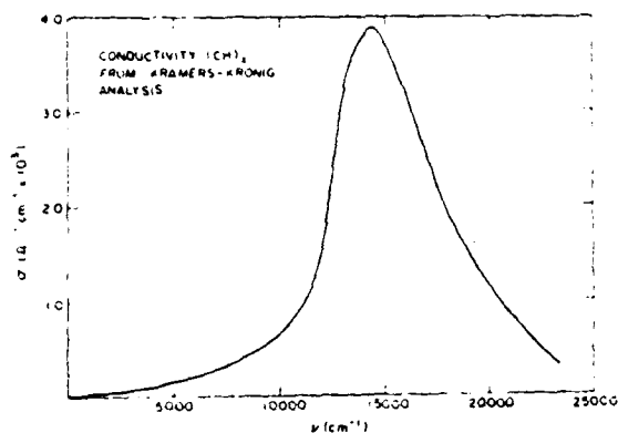
Fig. 5. \sigma(\omega) for \text{trans}-(\text{CH})_x as obtained from Kramers-Kronig analysis of the R_{||} reflection spectrum (ref. 29).
