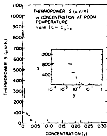
Fig. 12. Thermopower of (\text{CHI}_y)_x as a function of iodine concentration y . The inset shows the data with y on a log scale; the value for undoped (\text{CH})_x is indicated with an arrow (ref. 35).
