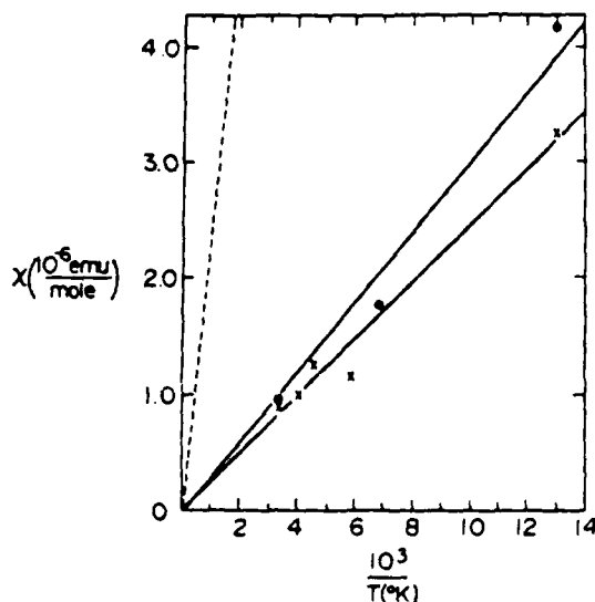
Fig. 11. Spin susceptibility of nonmagnetic (\text{CH})_x ooo undoped sample. xxx [\text{CH}(\text{AsF}_6)_{0.006}]_x . Both samples were from same batch of undoped polymer. The dotted line represents the Curie law expected for y=0.006 assuming \text{AsF}_6^- with spin \frac{1}{2} (ref. 22).
