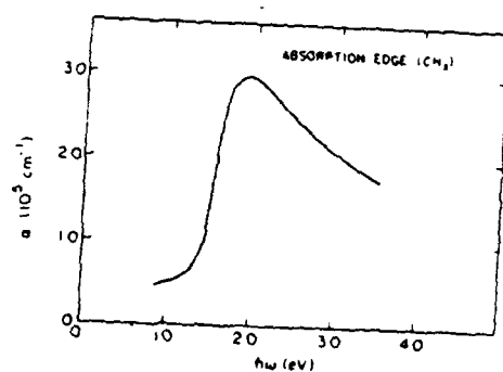
Fig. 3a. Absorption coefficient as a function of frequency; trans -(CH) x (ref. 29).
