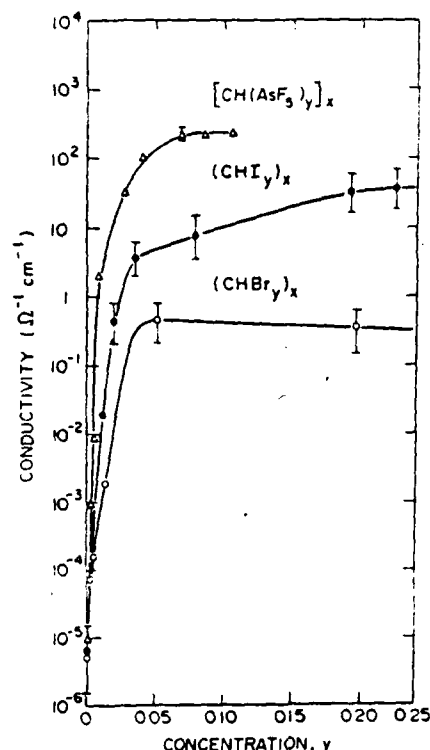
Fig. 8. Electrical conductivity (room temperature) as a function of dopant concentration.
