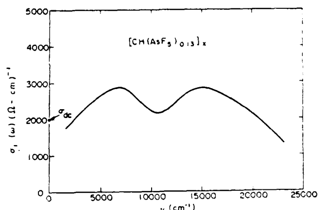
Fig. 17. \sigma_{||}(\omega) for heavily doped metallic [\text{CH}(\text{AsF}_6)_{0.13}]_x as obtained from the R_{||} reflection spectrum (ref. 29).
