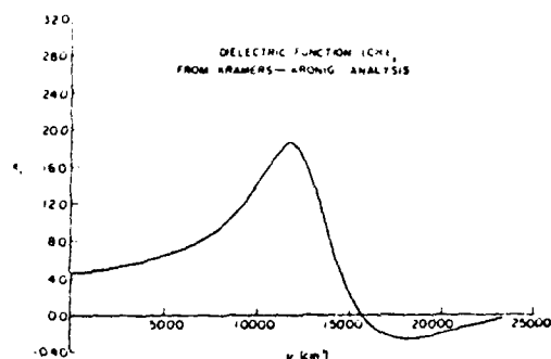
Fig. 6. \epsilon(\omega) for \text{trans}-(\text{CH})_x as obtained from Kramers-Kronig analysis of the R_{||} reflection spectrum (ref. 29).
