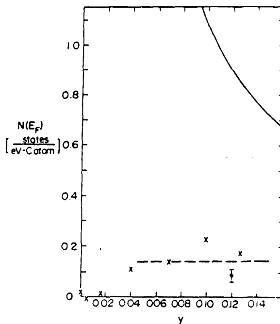
Fig. 14. Fermi-surface density of states vs \text{AsF}_5 concentration. The solid curve represents a rigid band one-dimensional density of state ( m^*/m = 1 ). The dashed curve would result from a half-filled simple tight-binding band with transfer integral t = 2.25 eV (bandwidth of 9 eV). x Faraday balance; • ESR (see ref.22).
