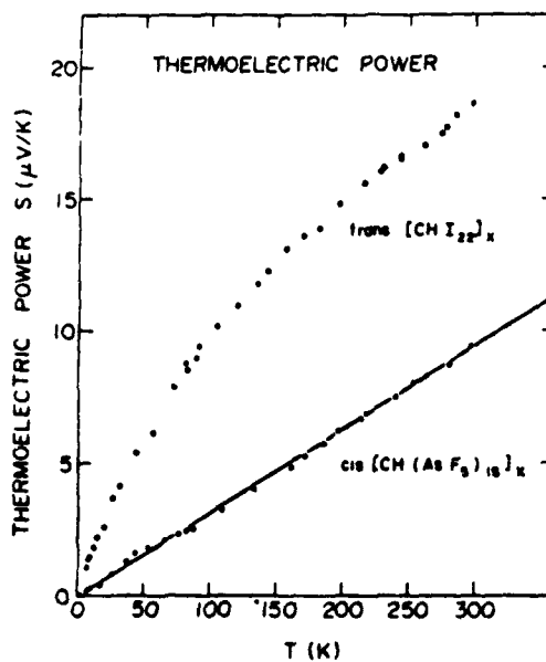
Fig. 13. Temperature dependence of the thermopower for heavily doped metallic (\text{CH})_x .
