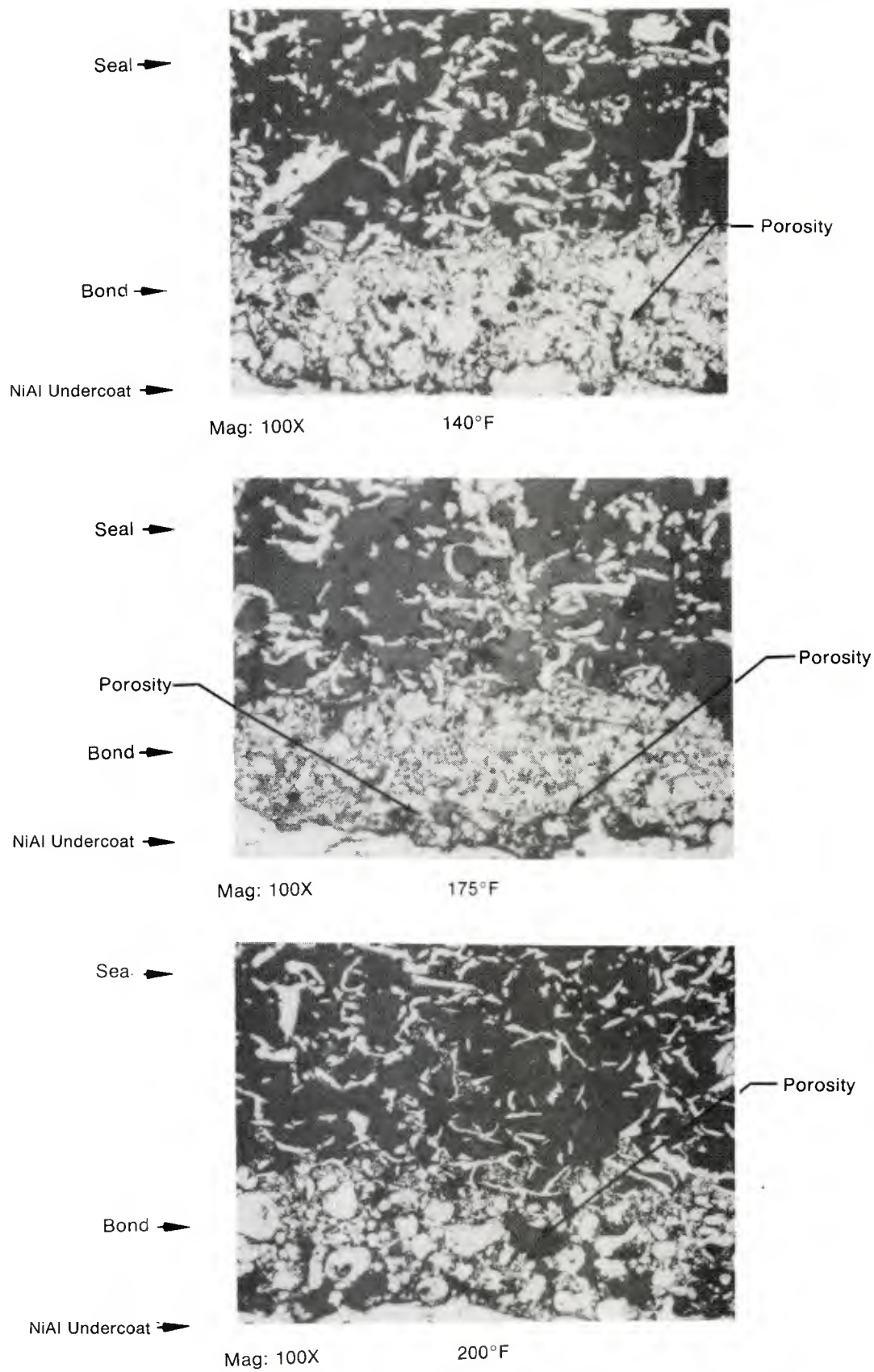
Figure 5. Effect of Drying Temperature on Inhibited Chem-Braze Porosity
