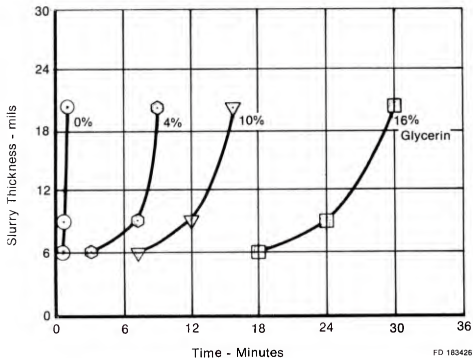
Figure 1. Glycerin Concentration Effect on Working Time
