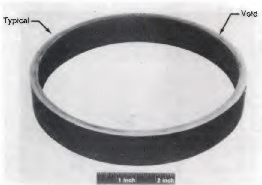
Figure 11. Simulated Engine Hardware Demonstration
