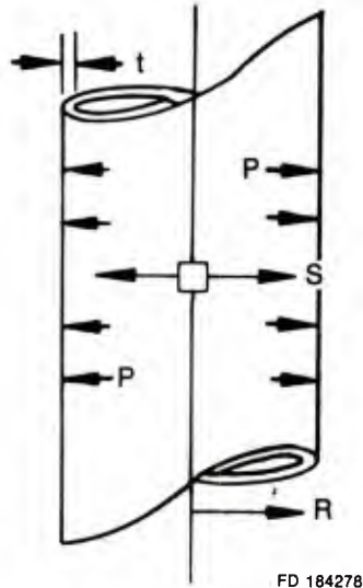
Figure I-1. Thin Walled Pressure Vessel
