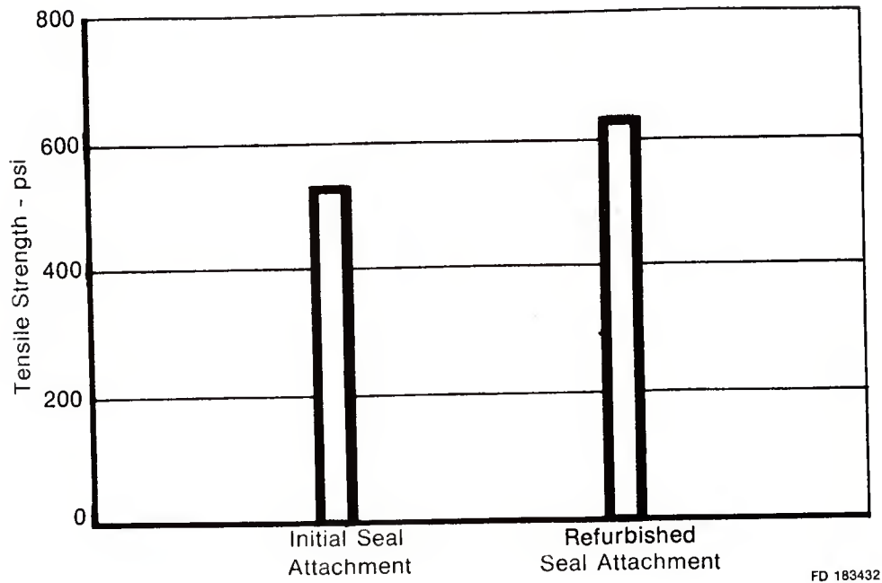
Figure 7. Tensile Strengths of Initial and Refurbished Seal Attachments
