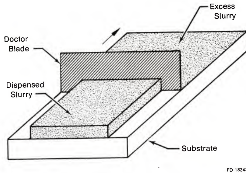
Figure 8. Doctor Blade Technique for Dispensing Inhibited Chem-Braze Slurry
