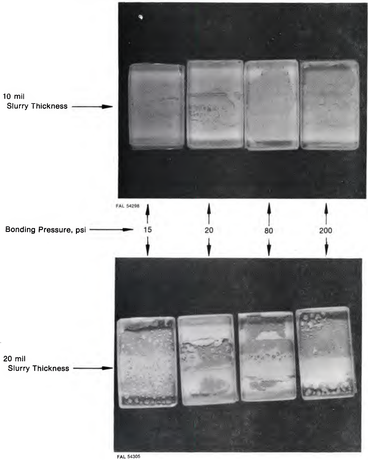
Figure 3. Inhibited Chem-Braze Slurry Thickness and Bonding Pressure Effects
