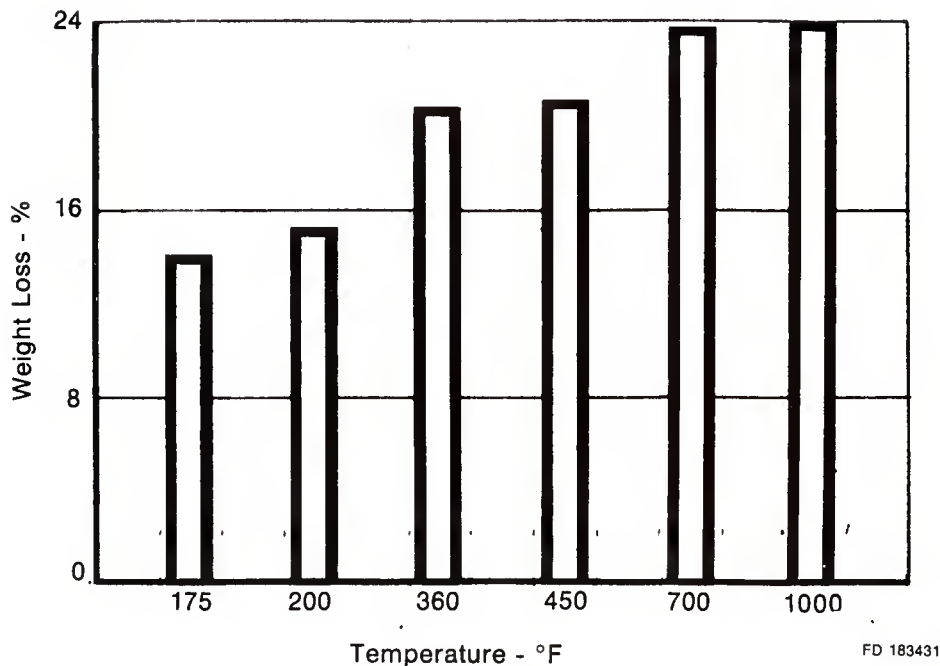
Figure 6. Inhibited Chem-Braze Cure Cycle Weight Losses
