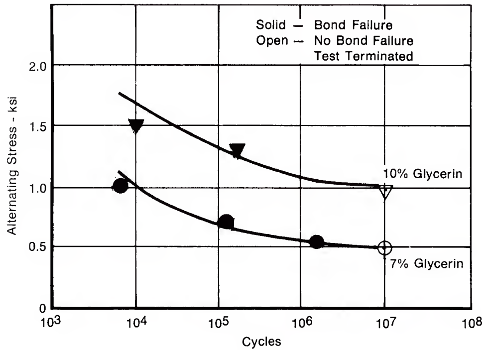
Figure 2. Inhibited Chem-Braze Vibration Test Results
