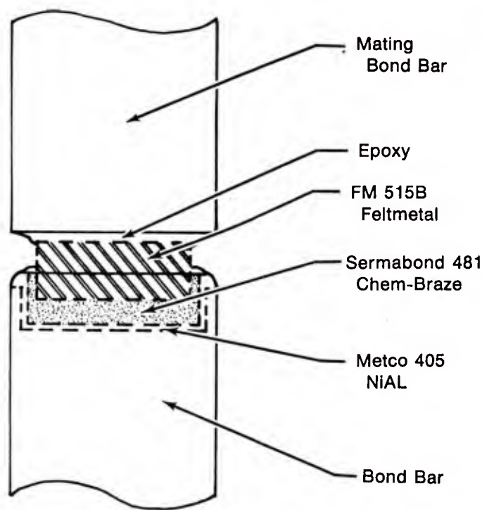
Figure D-1. Tensile Test Schematic
