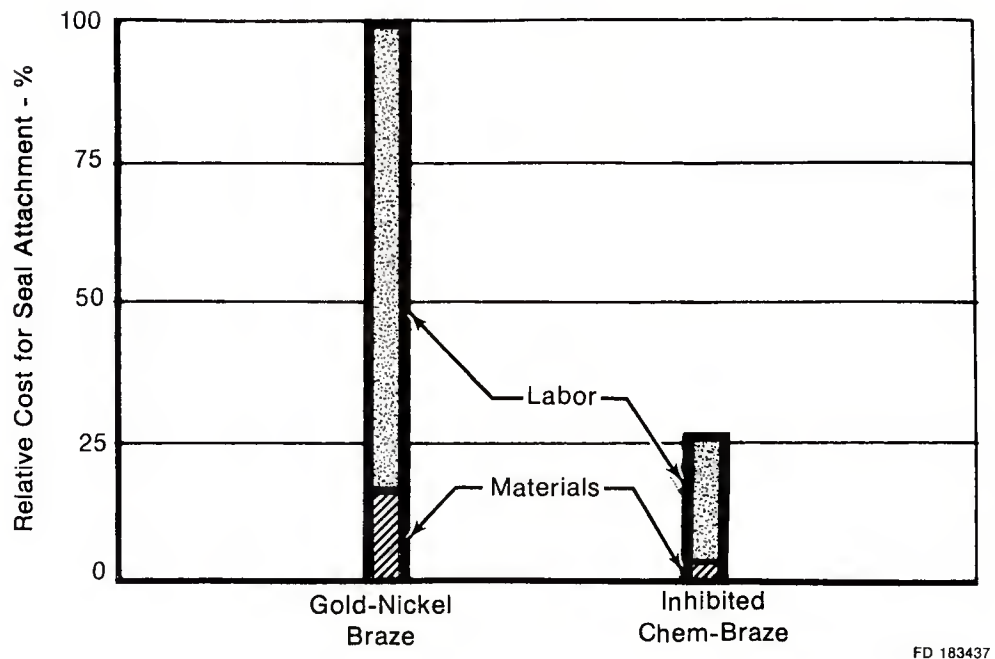
Figure 12. Preliminary Economic Comparison of Brazing Techniques for Common Compressor Stage Seal Attachment
