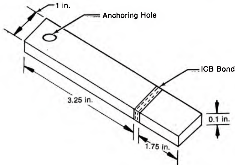
Figure G-1. Vibration Test Sample
