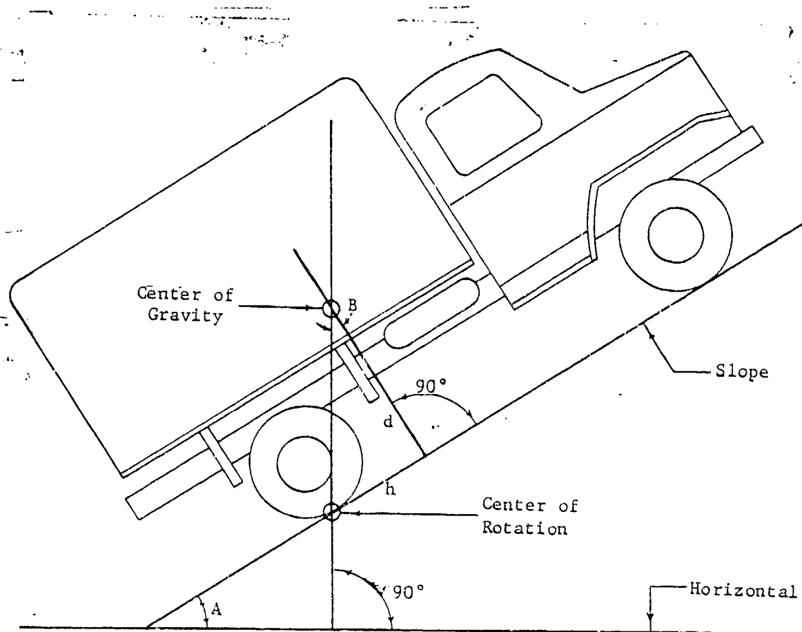
Figure 1. Critical Angle for Vehicle on a Slope.
