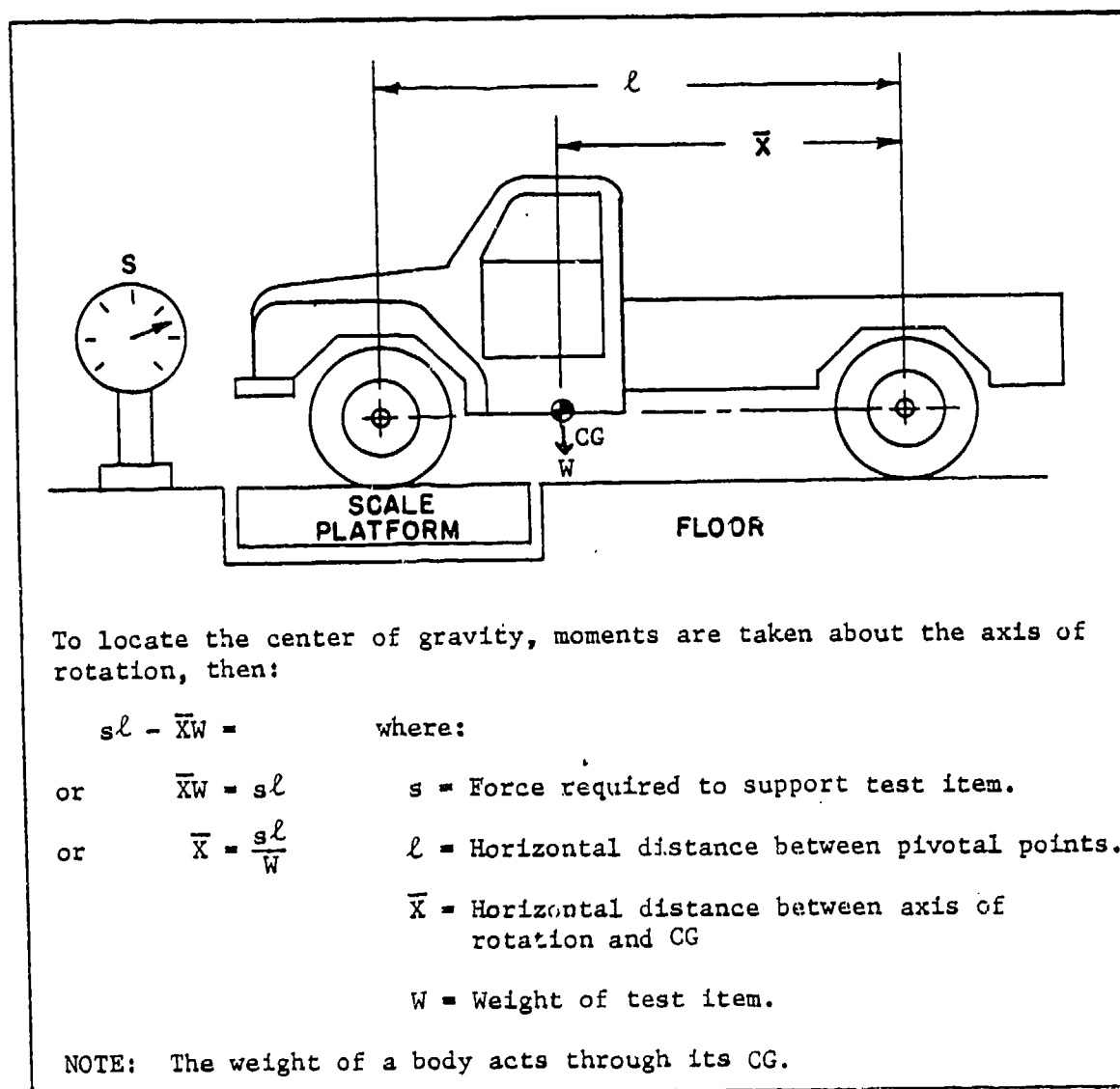
Figure 3. Weighing Method for Determining Horizontal Center of Gravity.
